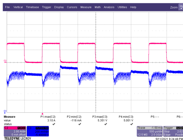
Figure 29 – Transient Response. 265 VAC, 5.0 V, 0 – 3 A Load Step. V_{MIN} : 5.001 V, V_{MAX} : 5.351 V. C3: V_{OUT} , 0.2 V / div. C2: I_{LOAD} , 2 A / div. Time: 0.5 ms / div.
