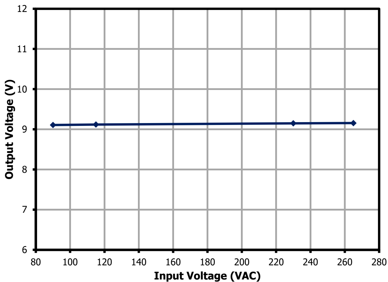
Figure 16 – Output Voltage vs. Input Line Voltage for 9 V Output, Room Temperature.
