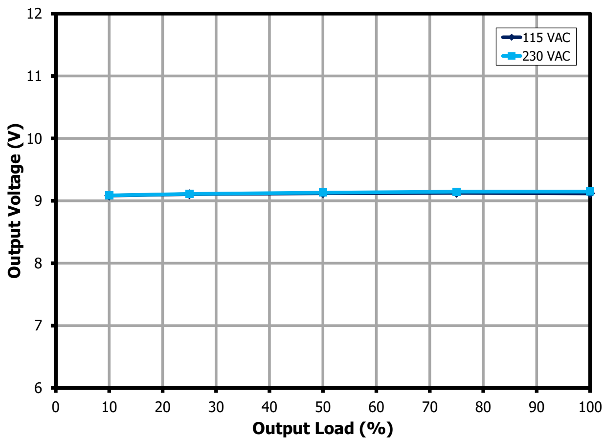
Figure 12 – Output Voltage vs. Output Load for 9 V Output, Room Temperature.
