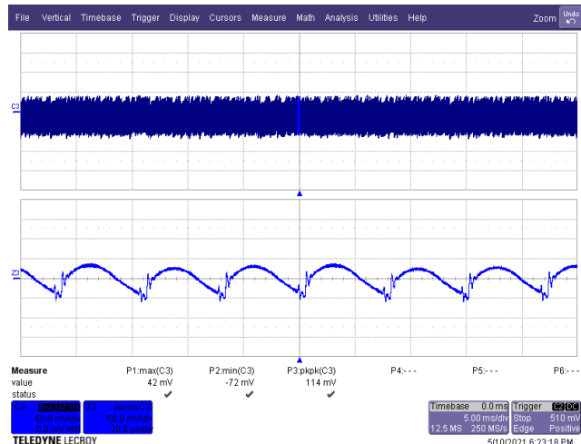
Figure 65 – Output Voltage Ripple. 265 VAC, 5.0 V, 3 A Load (114 mV PK-PK ). C3: V_{OUT(AC)} , 50 mV / div. Time: 5 ms / div. (20 \mu s / div. Zoom)
