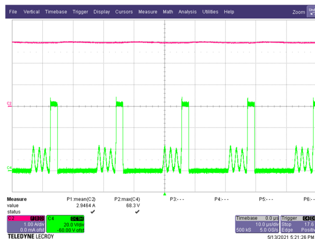
Figure 55 – SR FET Drain Voltage and Current. 265 VAC, 9.0 V, 3 A Load (68.3 V MAX ). C4: V DRAIN(SR) , 20 V / div. C2: I LOAD , 1 A / div. Time: 10 μs / div.
