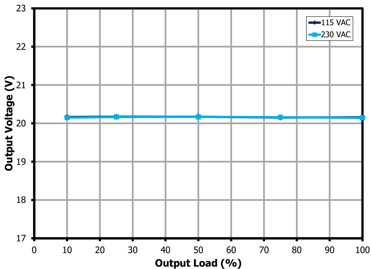
Figure 14 – Output Voltage vs. Output Load for 20 V Output, Room Temperature.
