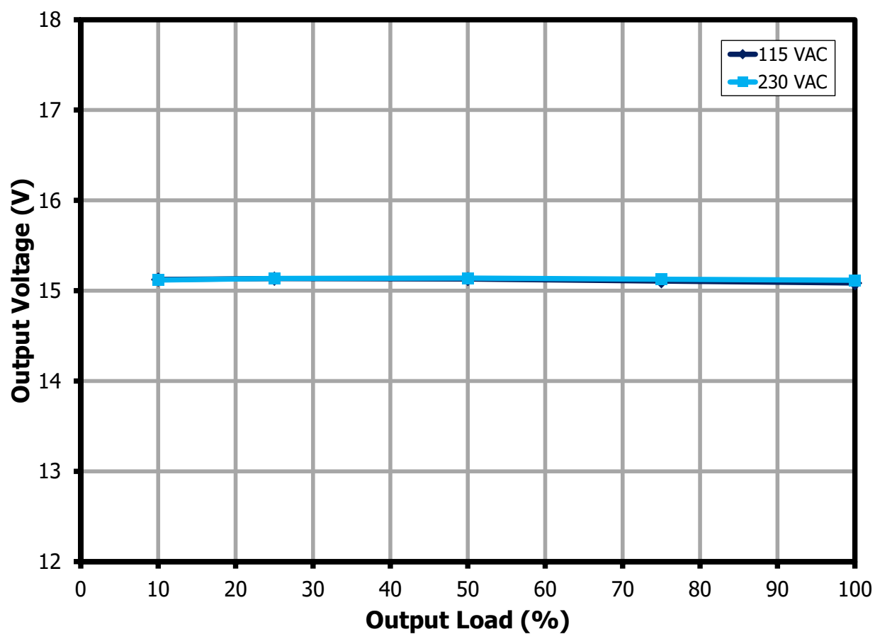
Figure 13 – Output Voltage vs. Output Load for 15 V Output, Room Temperature.
