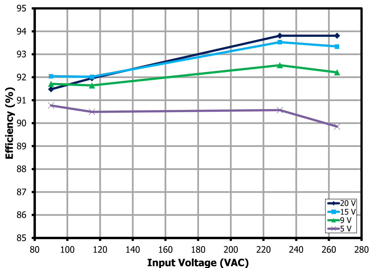
Figure 10 – Full Load Efficiency vs. Input Line for 5 V, 9 V, 15 V, and 20 V Output, Room Temperature.
