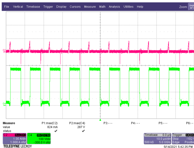
Figure 50 – Primary Clamp Drain Voltage and Current. 90 VAC, 20.0 V, 3 A Load (287 V MAX ). C4: V DRAIN , 100 V / div. C2: I DRAIN , 1 A / div. Time: 10 μs / div.
