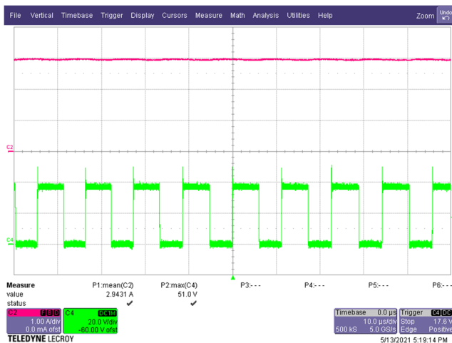
Figure 58 – SR FET Drain Voltage and Current. 90 VAC, 20.0 V, 3 A Load (51.0 V MAX ). C4: V DRAIN(SR) , 20 V / div. C2: I LOAD , 1 A / div. Time: 10 μs / div.
