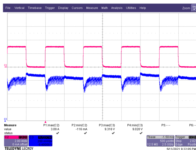
Figure 31 – Transient Response. 265 VAC, 9.0 V, 0 – 3 A Load Step. V_{MIN} : 9.020 V, V_{MAX} : 9.316 V. C3: V_{OUT} , 0.2 V / div. C2: I_{LOAD} , 2 A / div. Time: 0.5 ms / div.
