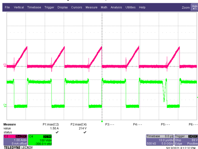
Figure 38 – Primary Drain Voltage and Current. 90 VAC, 9.0 V, 3 A Load (214 V MAX ). C4: V DRAIN , 100 V / div. C2: I DRAIN , 1 A / div. Time: 10 µs / div.
