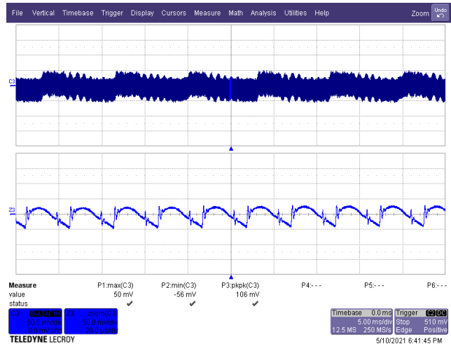
Figure 67 – Output Voltage Ripple. 115 VAC, 9.0 V, 3 A Load (106 mV PK-PK ). C3: V_{OUT(AC)} , 50 mV / div. Time: 5 ms / div. (20 \mu s / div. Zoom)
