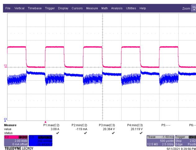
Figure 35 – Transient Response. 265 VAC, 20.0 V, 0 – 3 A Load Step. V_{MIN} : 20.119 V, V_{MAX} : 20.364 V. C3: V_{OUT} , 0.2 V / div. C2: I_{LOAD} , 2 A / div. Time: 0.5 ms / div.
