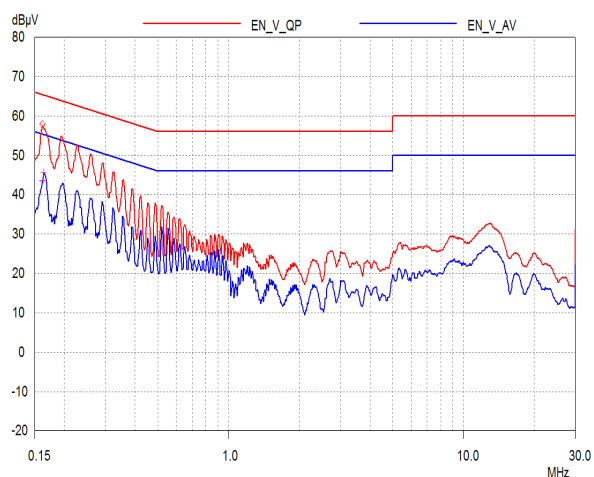
Figure 94 – Floating Ground EMI, 5 V / 3 A Load.
