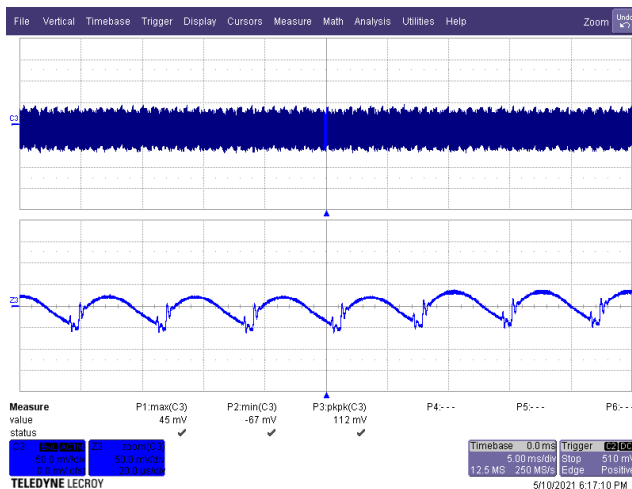
Figure 64 – Output Voltage Ripple. 230 VAC, 5.0 V, 3 A Load (112 mV PK-PK ). C3: V_{OUT(AC)} , 50 mV / div. Time: 5 ms / div. (20 \mu s / div. Zoom)
