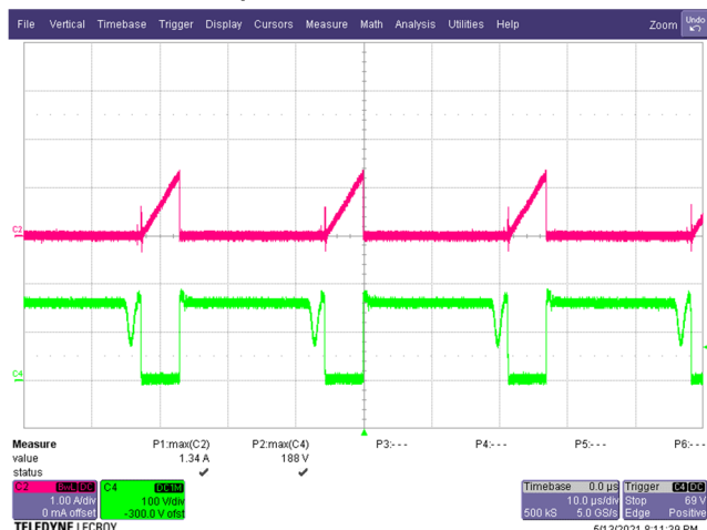
Figure 36 – Primary Drain Voltage and Current. 90 VAC, 5.0 V, 3 A Load (188 V MAX ). C4: V DRAIN , 100 V / div. C2: I DRAIN , 1 A / div. Time: 10 µs / div.
