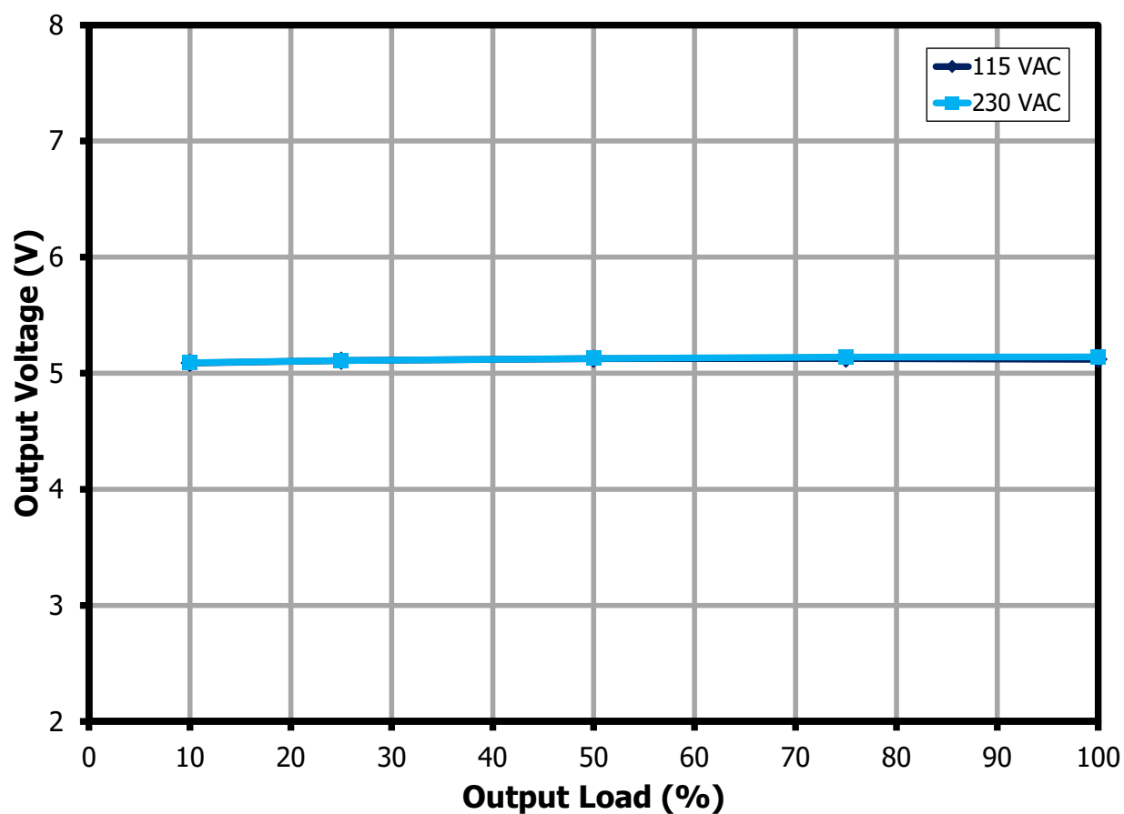
Figure 11 – Output Voltage vs. Output Load for 5 V Output, Room Temperature.
