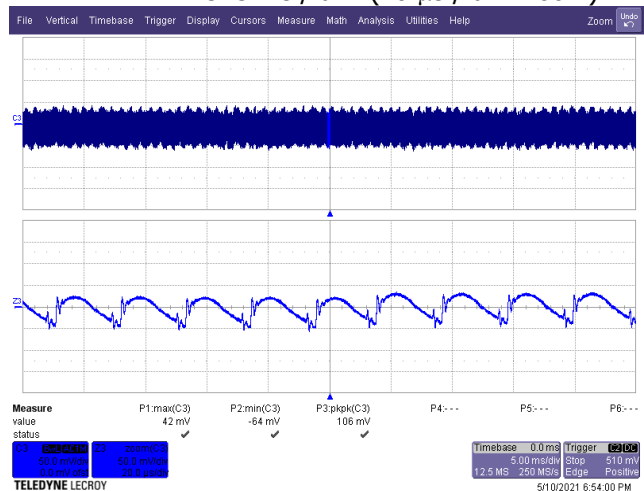
Figure 69 – Output Voltage Ripple. 265 VAC, 9.0 V, 3 A Load (106 mV PK-PK ). C3: V_{OUT(AC)} , 50 mV / div. Time: 5 ms / div. (20 \mu s / div. Zoom)
