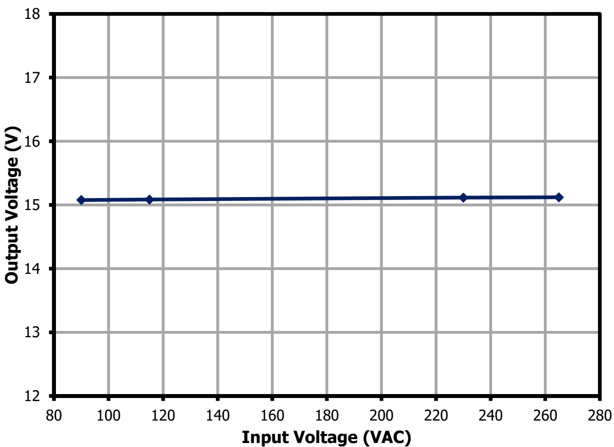
Figure 17 – Output Voltage vs. Input Line Voltage for 15 V Output, Room Temperature.
