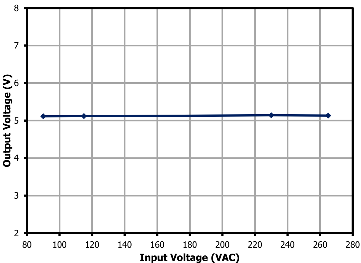
Figure 15 – Output Voltage vs. Input Line Voltage for 5 V Output, Room Temperature.
