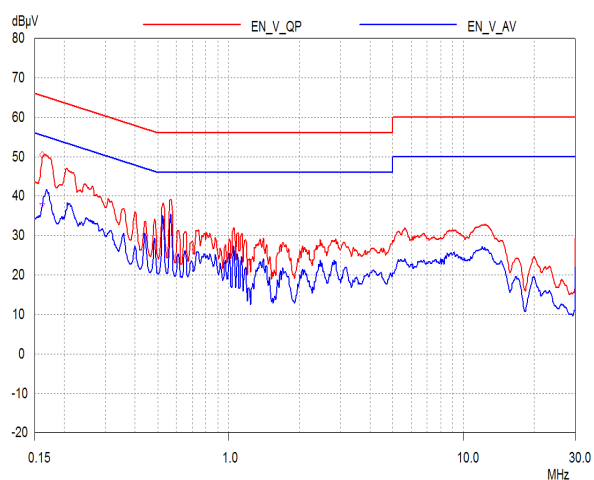
Figure 95 – Floating Ground EMI, 9 V / 3 A Load.
