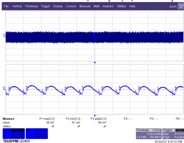
Figure 68 – Output Voltage Ripple. 230 VAC, 9.0 V, 3 A Load (99 mV PK-PK ). C3: V_{OUT(AC)} , 50 mV / div. Time: 5 ms / div. (20 \mu s / div. Zoom)
