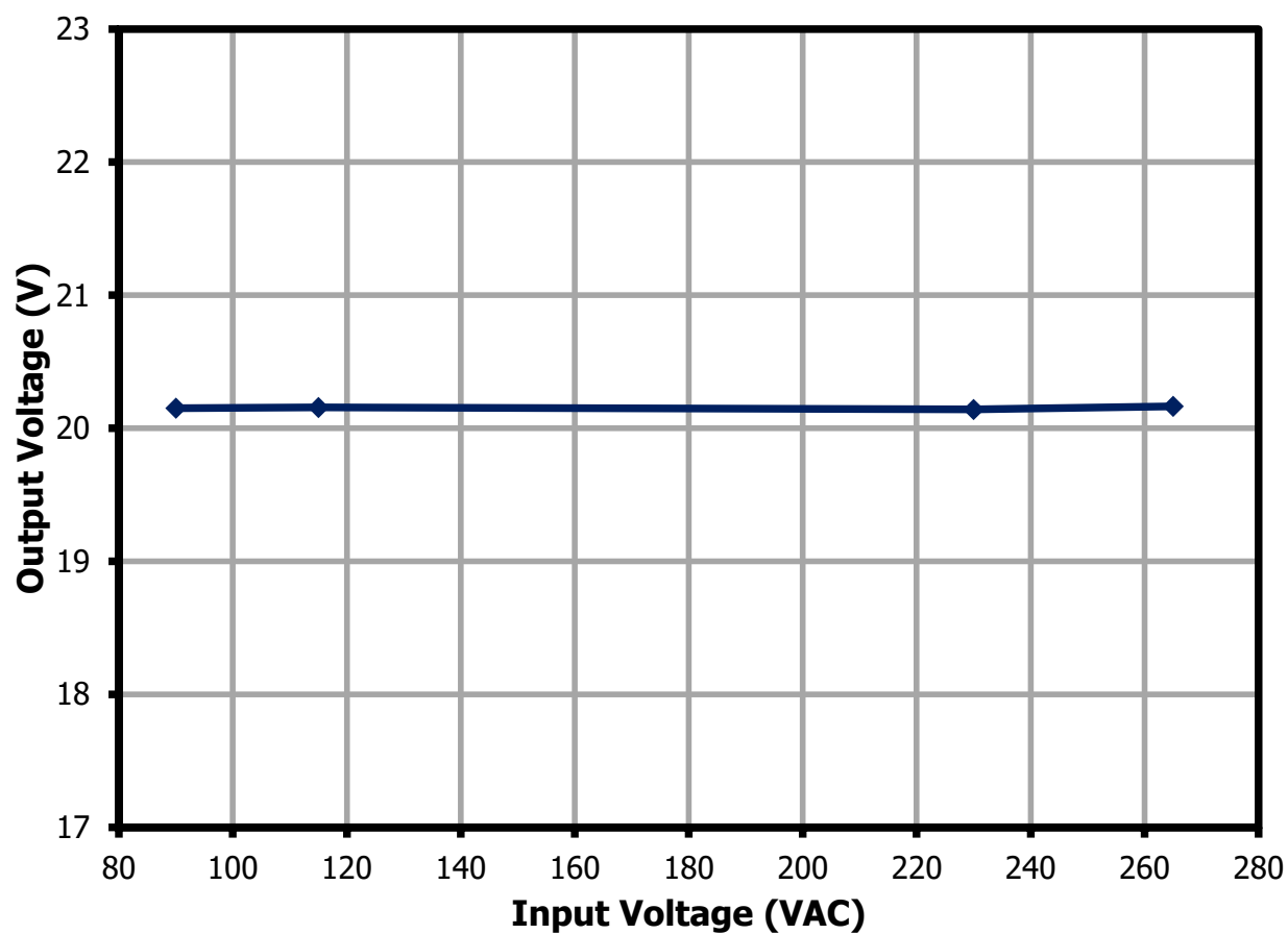
Figure 18 – Output Voltage vs. Input Line Voltage for 20 V Output, Room Temperature.
