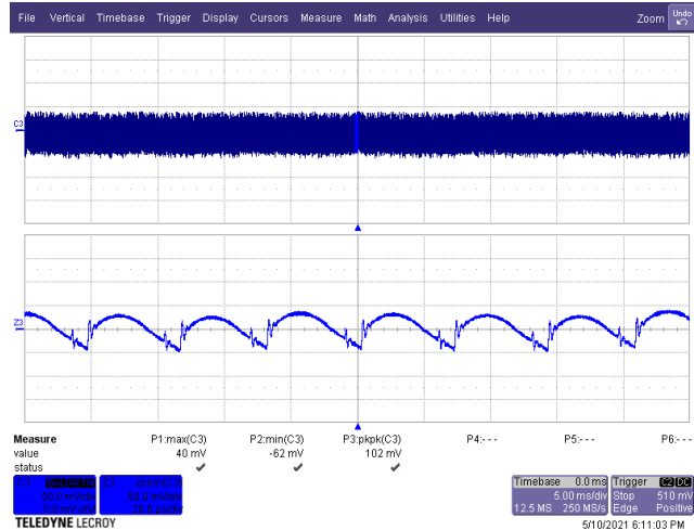
Figure 63 – Output Voltage Ripple. 115 VAC, 5.0 V, 3 A Load (102 mV PK-PK ). C3: V_{OUT(AC)} , 50 mV / div. Time: 5 ms / div. (20 \mu s / div. Zoom)
