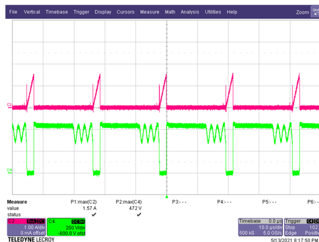
Figure 39 – Primary Drain Voltage and Current. 265 VAC, 9.0 V, 3 A Load (472 V MAX ). C4: V DRAIN , 200 V / div. C2: I DRAIN , 1 A / div. Time: 10 µs / div.
