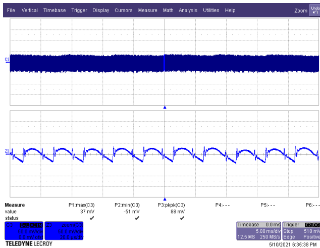
Figure 66 – Output Voltage Ripple. 90 VAC, 9.0 V, 3 A Load (88 mV PK-PK ). C3: V_{OUT(AC)} , 50 mV / div. Time: 5 ms / div. (20 \mu s / div. Zoom)
