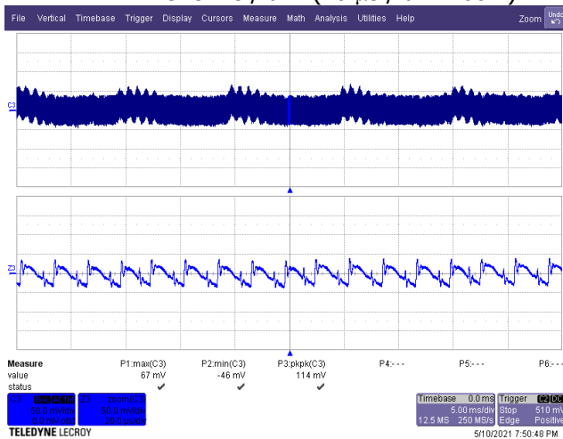
Figure 74 – Output Voltage Ripple. 90 VAC, 20.0 V, 3 A Load (114 mV PK-PK ). C3: V OUT(AC) , 50 mV / div. Time: 5 ms / div. (20 \mu s / div. Zoom)
