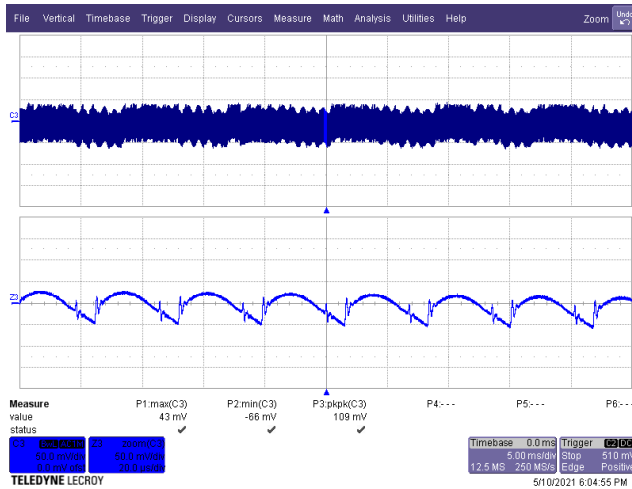
Figure 62 – Output Voltage Ripple. 90 VAC, 5.0 V, 3 A Load (109 mV PK-PK ). C3: V_{OUT(AC)} , 50 mV / div. Time: 5 ms / div. (20 \mu s / div. Zoom)
