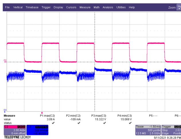
Figure 33 – Transient Response. 265 VAC, 15.0 V, 0 – 3 A Load Step. V_{MIN} : 15.069 V, V_{MAX} : 15.322 V. C3: V_{OUT} , 0.2 V / div. C2: I_{LOAD} , 2 A / div. Time: 0.5 ms / div.
