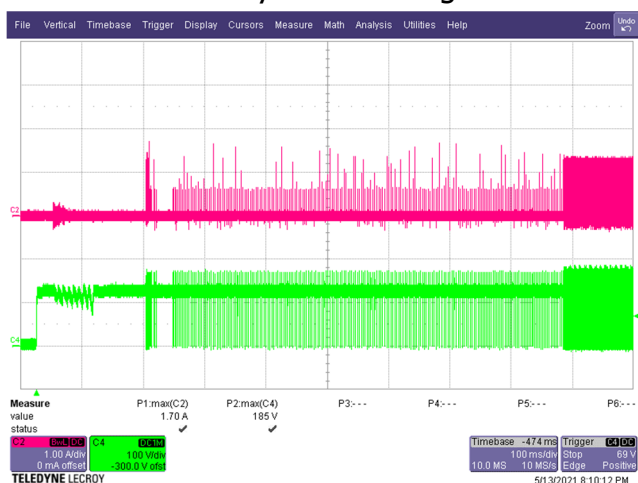
Figure 22 – Primary Drain Voltage and Current. 90 VAC, 5.0 V, 3 A Load (185 V MAX ). C4: V_{DRAIN} , 100 V / div. C2: I_{DRAIN} , 1 A / div. Time: 100 ms / div.
