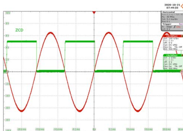
Figure 38 – 265 VAC 50 Hz, Full Load.
