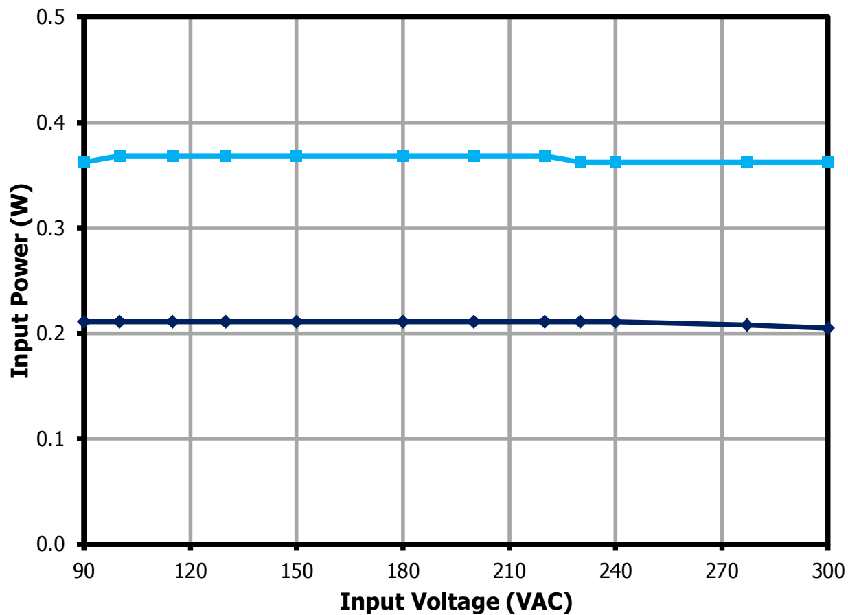
Figure 11 – Available Standby Output Power for 0.3 W and 0.5 W Input Power.
