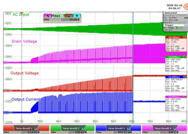
Figure 99 – Brown-in, Full Load.
