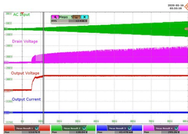
Figure 100 – Brown-in, No Load.
