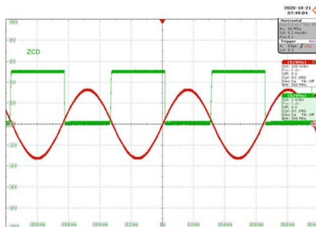
Figure 36 – 115 VAC 60 Hz, Full Load.
