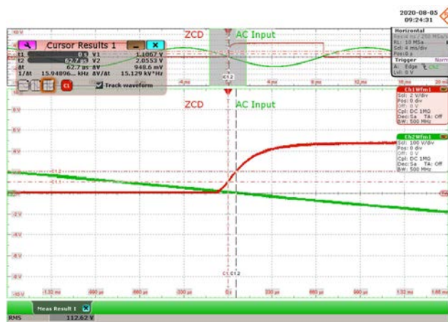
Figure 32 – 115 VAC 60 Hz, Full Load.
