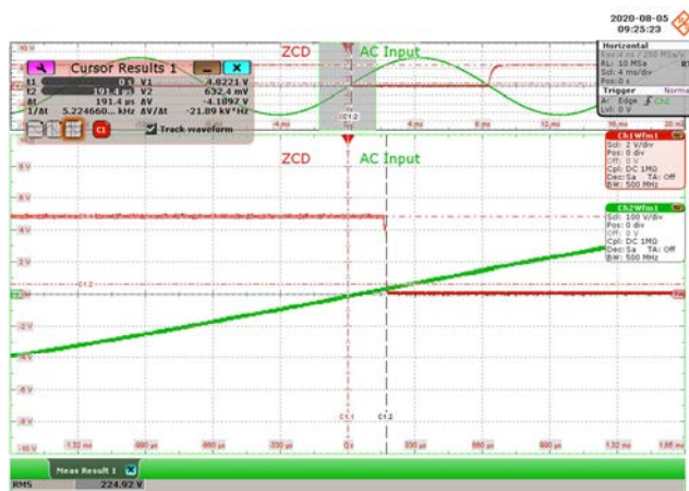
Figure 33 – 230 VAC 50 Hz, Full Load.
