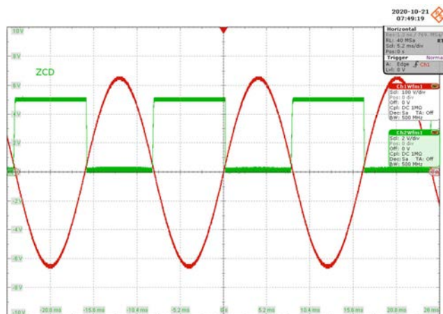
Figure 37 – 230 VAC 50 Hz, No-Load.
