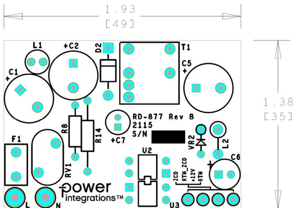
Figure 4 – Populated Circuit Board, Top View.
