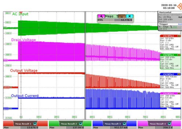
Figure 101 – Brown-out, Full Load.
