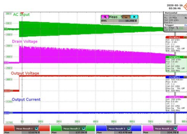
Figure 102 – Brown-out, No Load.
