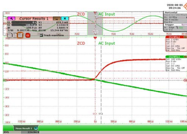
Figure 34 – 230 VAC 50 Hz, Full Load.
