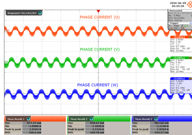
Figure 25 – Phase Current at 100 W Load.
