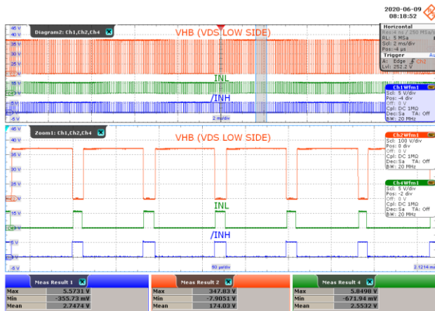
Figure 30 – INL and /INH Signal at 200 W Load.
