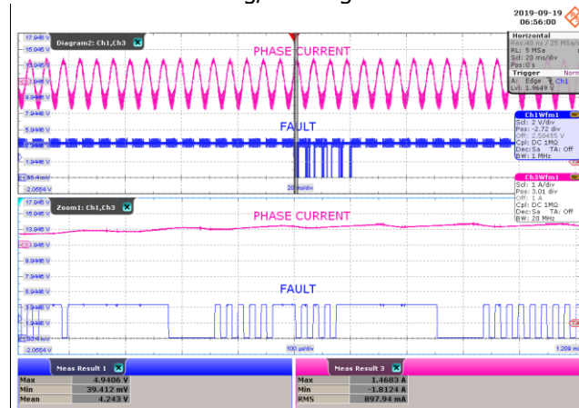
Figure 50 – Thermal Warning at 300 W.
