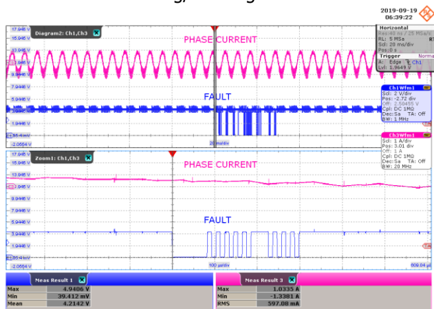
Figure 49 – Thermal Warning at 200 W.
