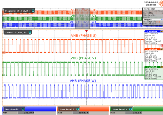
Figure 16 – Drain to Source Voltage at Light Load.
