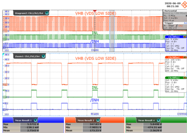
Figure 28 – INL and /INH Signal at Light Load.
