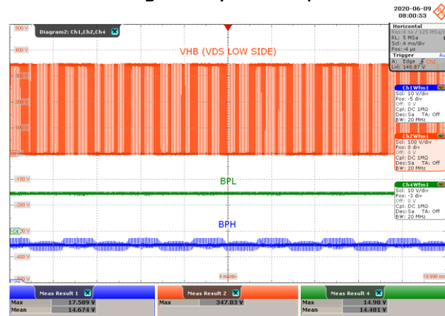
Figure 33 – BPL and BPH Signal at 100 W Load.
