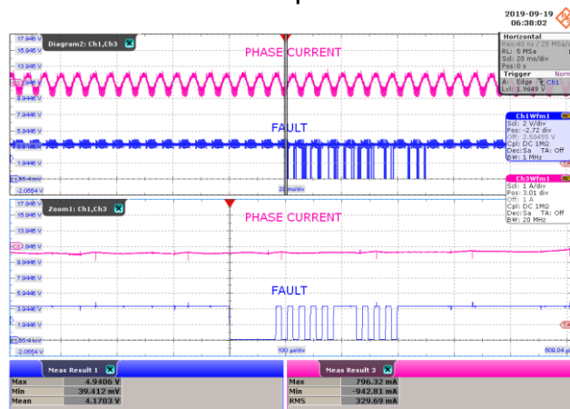
Figure 48 – Thermal Warning at 100 W.
