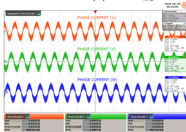
Figure 27 – Phase Current at 300 W Load.
