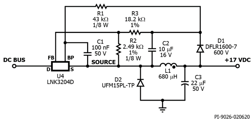
Figure 7 – Auxiliary Schematic.
