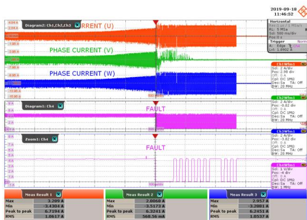
Figure 62 – At Stalled Condition, 200 W Load.
