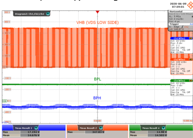
Figure 32 – BPL and BPH Signal at Light Load.
