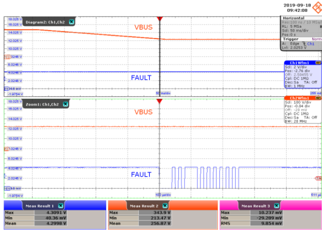
Figure 52 – UVP, 5000 RPM, No-Load, 340 V to 220 V.
