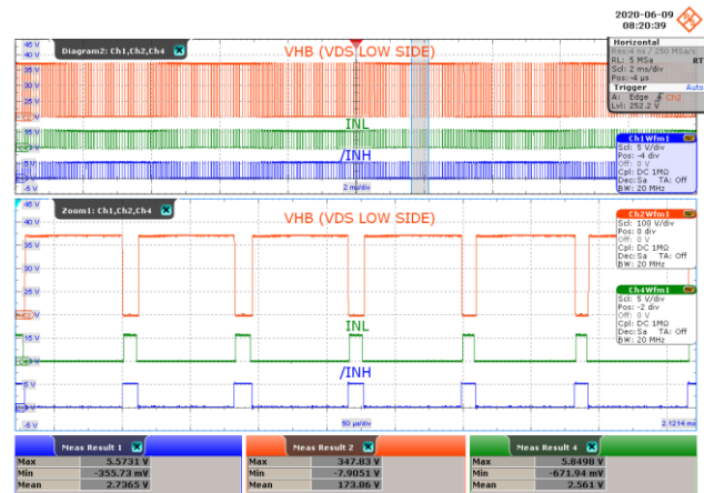
Figure 31 – INL and /INH Signal at 300 W Load.
