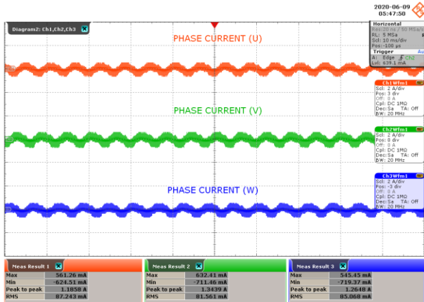
Figure 24 – Phase Current at No-Load.
