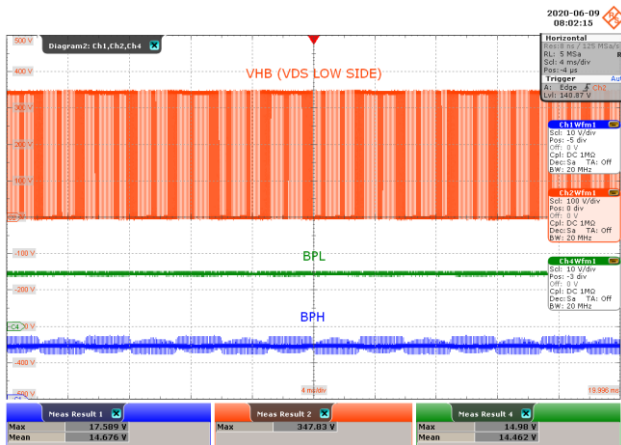
Figure 34 – BPL and BPH Signal at 200 W Load.
