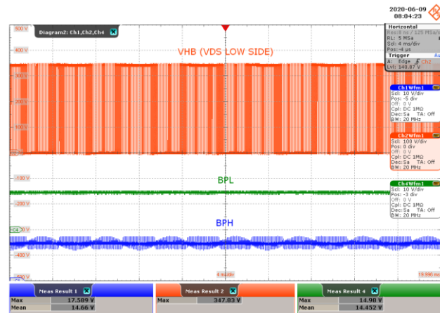
Figure 35 – BPL and BPH Signal at 300 W Load.
