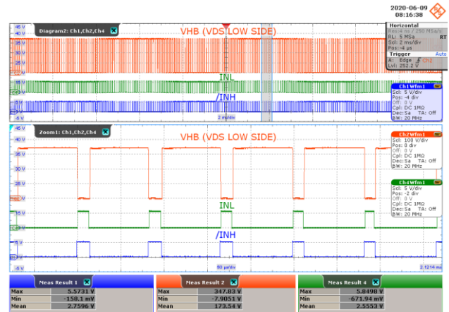
Figure 29 – INL and /INH Signal at 100 W Load.
