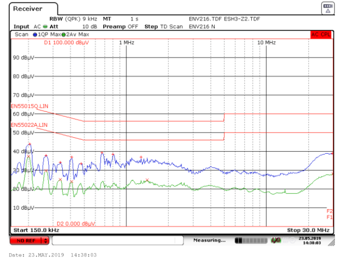
Figure 136 – 115 VAC 60 Hz, Neutral with Artificial Hand.
