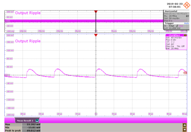
Figure 116 – 265 VAC 50 Hz.
