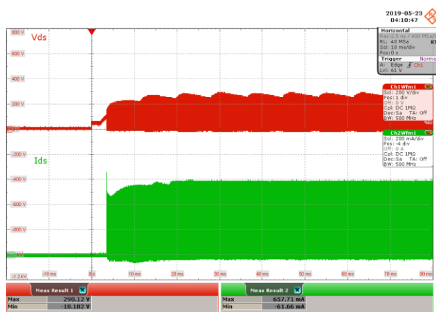
Figure 47 – 85 VAC 60 Hz.
