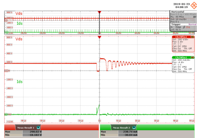
Figure 44 – 115 VAC 60 Hz.
