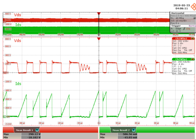
Figure 39 – 85 VAC 60 Hz.
