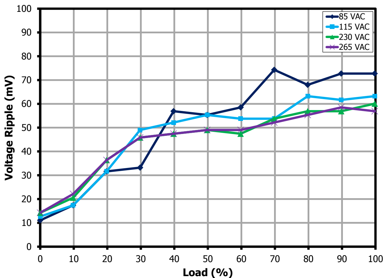
Figure 125 – Measured at the Board Output Terminals at Room Temperature.
