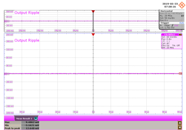
Figure 122 – 115 VAC 60 Hz.
