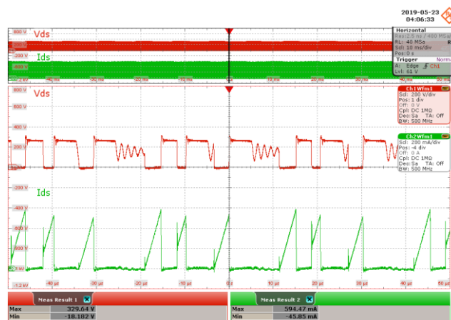
Figure 40 – 115 VAC 60 Hz.
