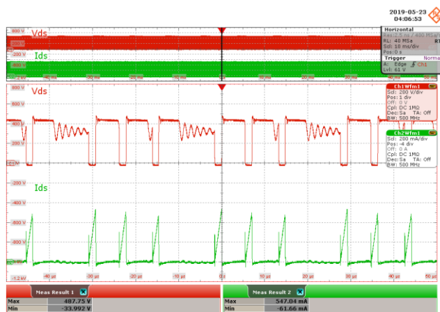
Figure 41 – 230 VAC 50 Hz.
