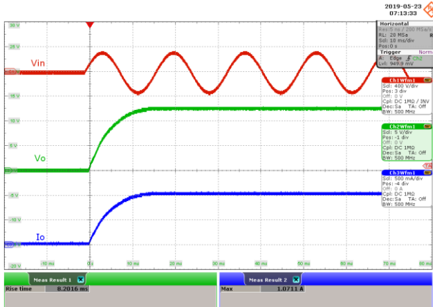
Figure 33 – 230 VAC 50 Hz.
