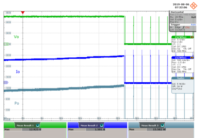
Figure 102 – 265 VAC 50 Hz.
