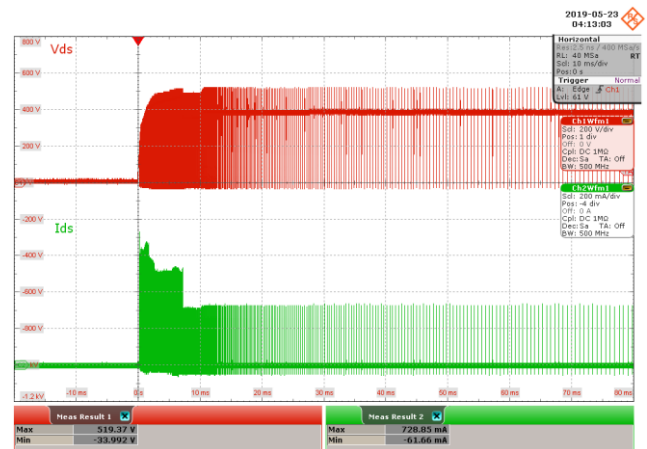
Figure 54 – 265 VAC 50 Hz.
