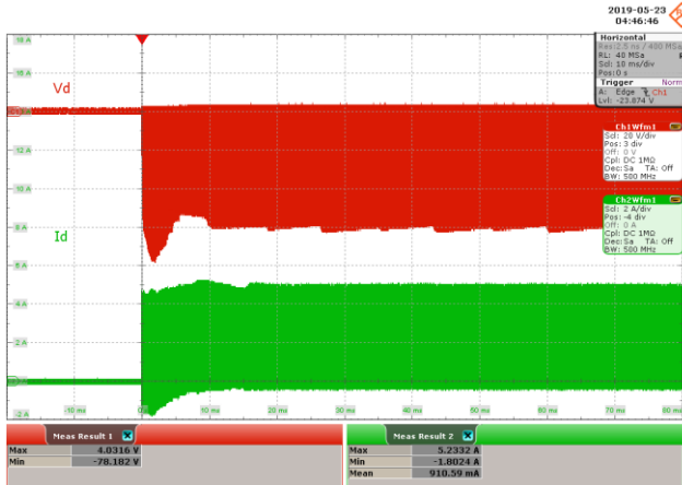
Figure 65 – 230 VAC 50 Hz.
