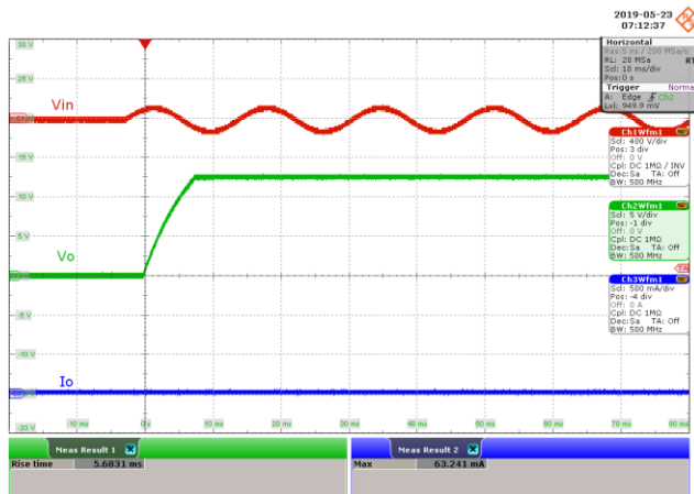
Figure 35 – 85 VAC 60 Hz.
