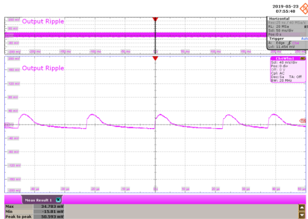
Figure 115 – 230 VAC 50 Hz.
