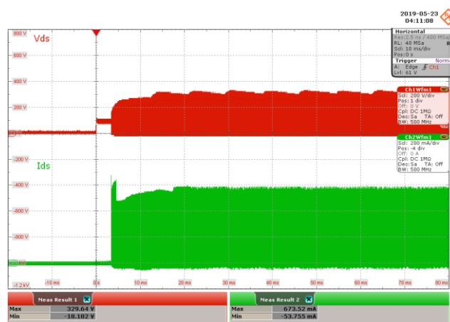
Figure 48 – 115 VAC 60 Hz.
