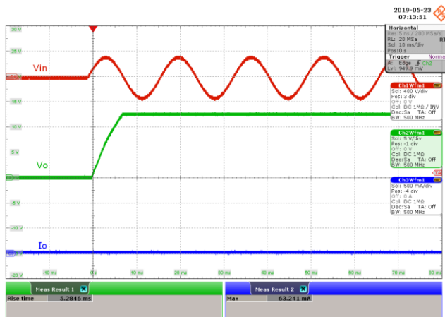
Figure 37 – 230 VAC 50 Hz.
