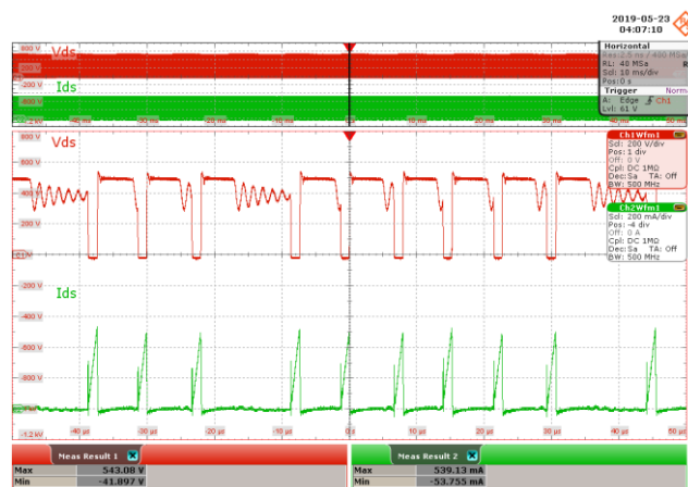
Figure 42 – 265 VAC 50 Hz.
