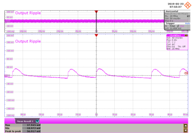
Figure 114 – 115 VAC 60 Hz.
