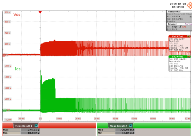
Figure 51 – 85 VAC 60 Hz.
