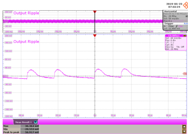
Figure 113 – 85 VAC 60 Hz.
