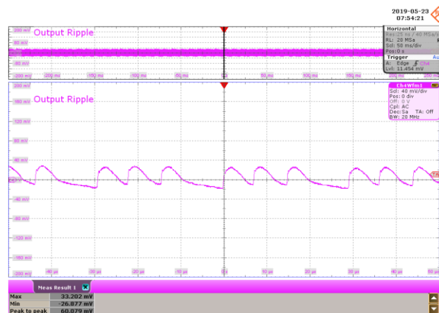
Figure 108 – 265 VAC 50 Hz.
