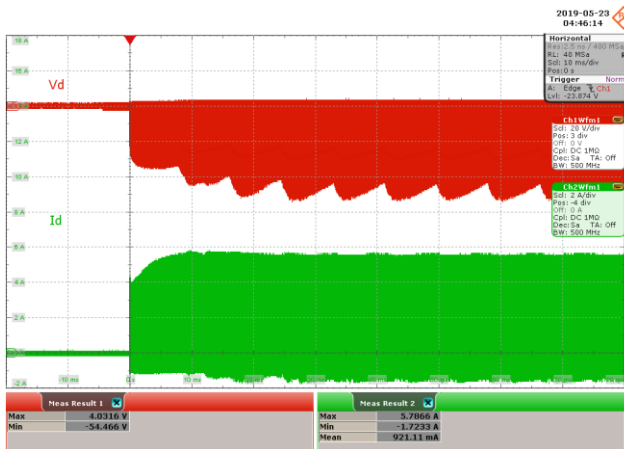
Figure 63 – 85 VAC 60 Hz.
