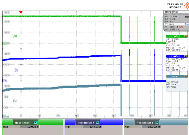
Figure 101 – 230 VAC 50 Hz.
