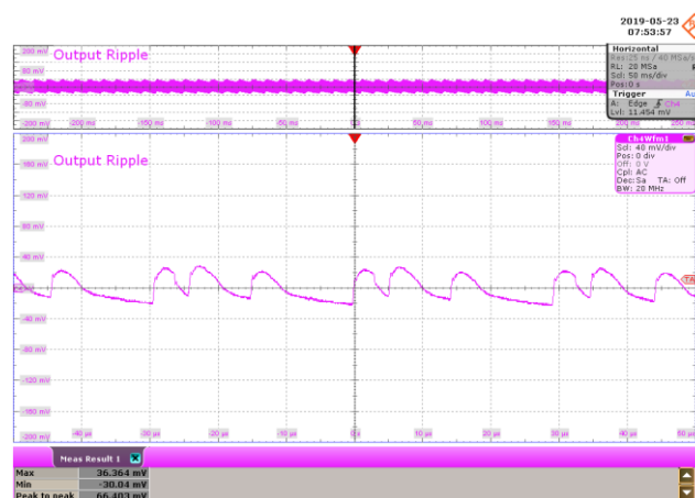
Figure 106 – 115 VAC 60 Hz.
