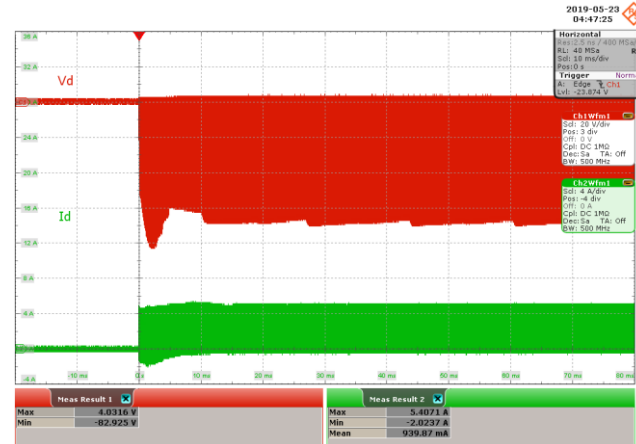
Figure 66 – 265 VAC 50 Hz.
