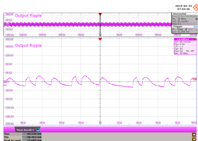
Figure 105 – 85 VAC 60 Hz.
