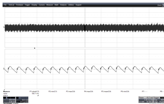
Figure 114 – Output Ripple. PK-PK = 100.7 mV. 265 VAC IN 20 V, 3 A Load. V OUT , 50 mV / div., 5 ms / div. Zoom: 31.5 μs / div.
