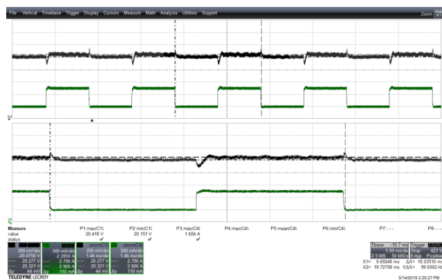
Figure 71 – Transient Response.
