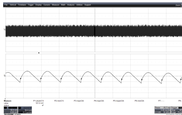
Figure 100 – Output Ripple. PK-PK = 121 mV. 115 VAC IN 5.0 V, 3 A Load. V OUT , 50 mV / div., 5 ms / div. Zoom: 31.5 \mu s / div.
