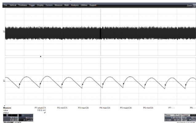
Figure 99 – Output Ripple. PK-PK = 119.6 mV. 85 VAC IN 5.0 V, 3 A Load. V OUT , 50 mV / div., 5 ms / div. Zoom: 31.5 \mu s / div.
