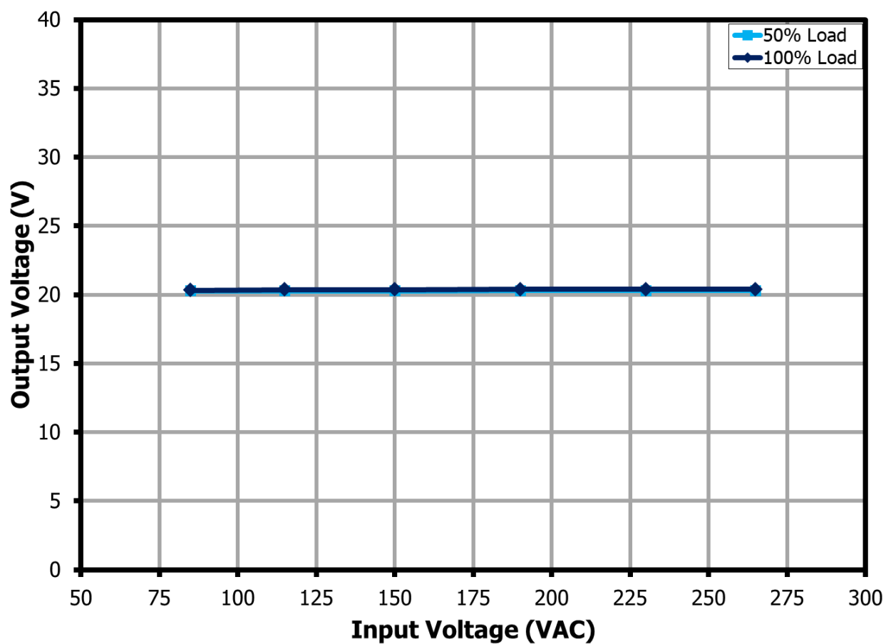
Figure 25 – Output Voltage vs. Input Line Voltage for 20 V Output, Room Temperature.
