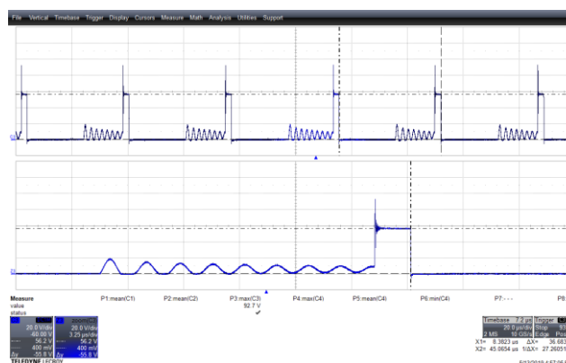
Figure 86 – SR FET Voltage Waveforms. 265 VAC, 5.0 V, 3 A Load (92.7 V_{MAX} ). Blue: V_{DRAIN} , 20 V, 10 \mu s / div. Zoom: 3.25 \mu s / div.
