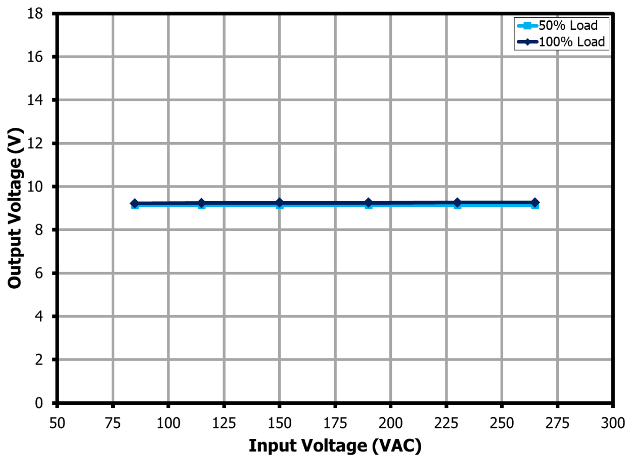
Figure 23 – Output Voltage vs. Input Line Voltage for 9 V Output, Room Temperature.
