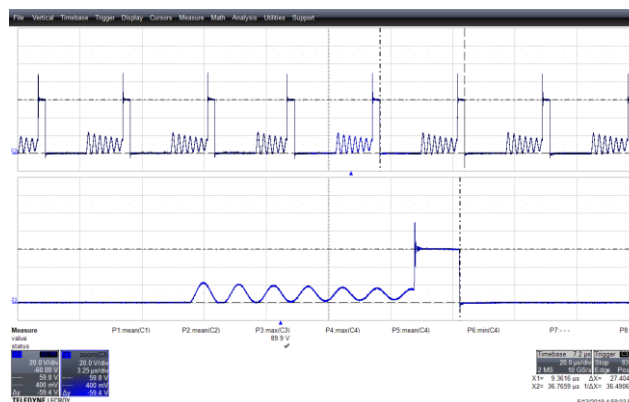
Figure 88 – SR FET Voltage Waveforms. 265 VAC, 9.0 V, 3 A Load (89.9 V_{MAX} ). Blue: V_{DRAIN} , 20 V, 20 \mu s / div. Zoom: 3.25 \mu s / div.
