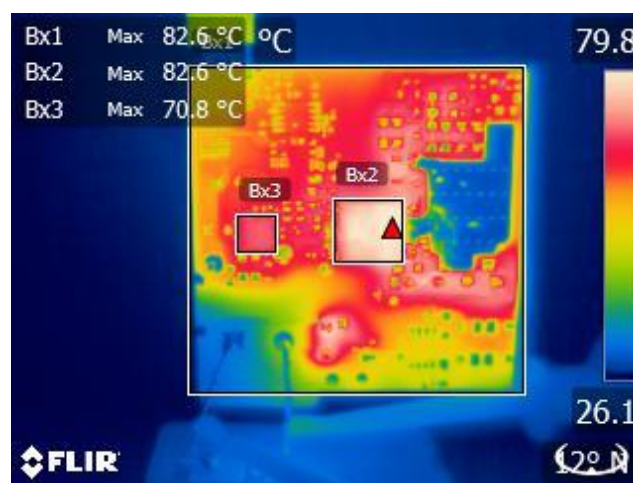
Figure 38 – Bottom Side Thermal Image. Ambient: 25.6 °C. Bx2: InnoSwitch3-Pro = 82.6 °C. Bx3: SR FET = 70.8 °C.
