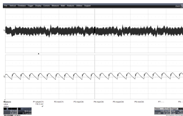
Figure 112 – Output Ripple. PK-PK = 116.3 mV. 115 VAC IN , 20 V, 3 A Load. V OUT , 50 mV / div., 5 ms / div. Zoom: 31.5 μs / div.
