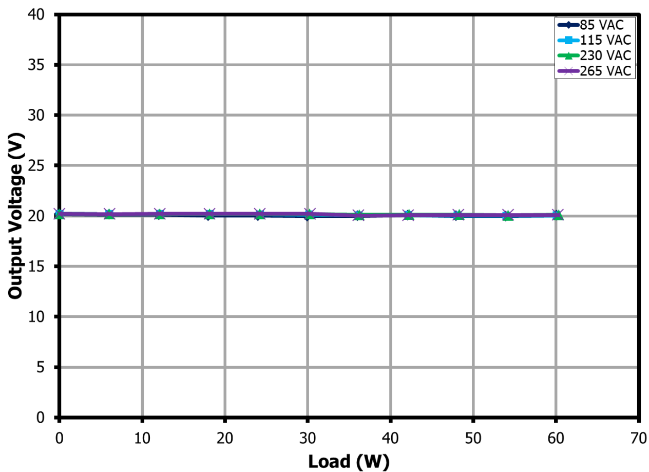
Figure 30 – Output Voltage vs. Output Load for 20 V Output, Room Temperature.
