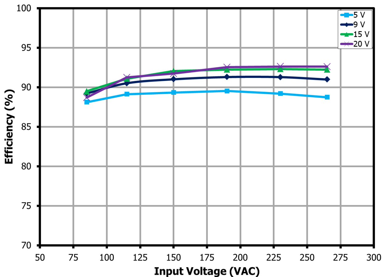
Figure 21 – Full Load Efficiency vs. Input Line for 5 V, 9 V, 15 V, and 20 V Output, Room Temperature.
