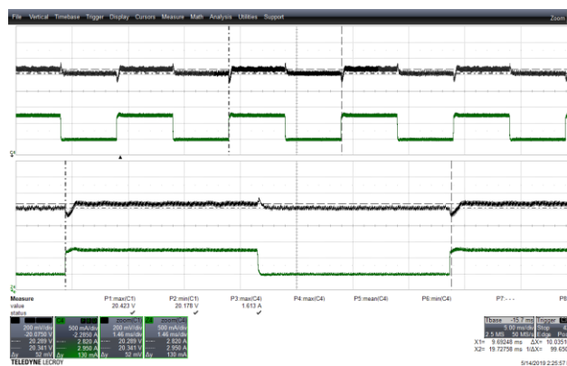
Figure 72 – Transient Response.
