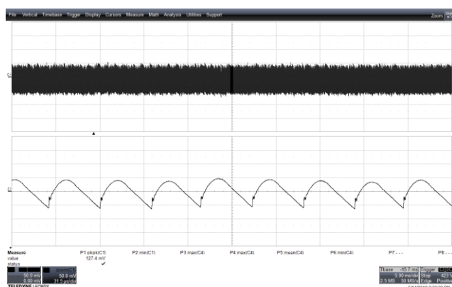
Figure 101 – Output Ripple. PK-PK = 127.4 mV. 230 VAC IN 5.0 V, 3 A Load. V OUT , 50 mV / div., 5 ms / div. Zoom: 31.5 \mu s / div.
