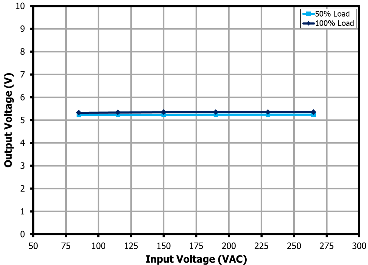
Figure 22 – Output Voltage vs. Input Line Voltage for 5 V Output, Room Temperature.
