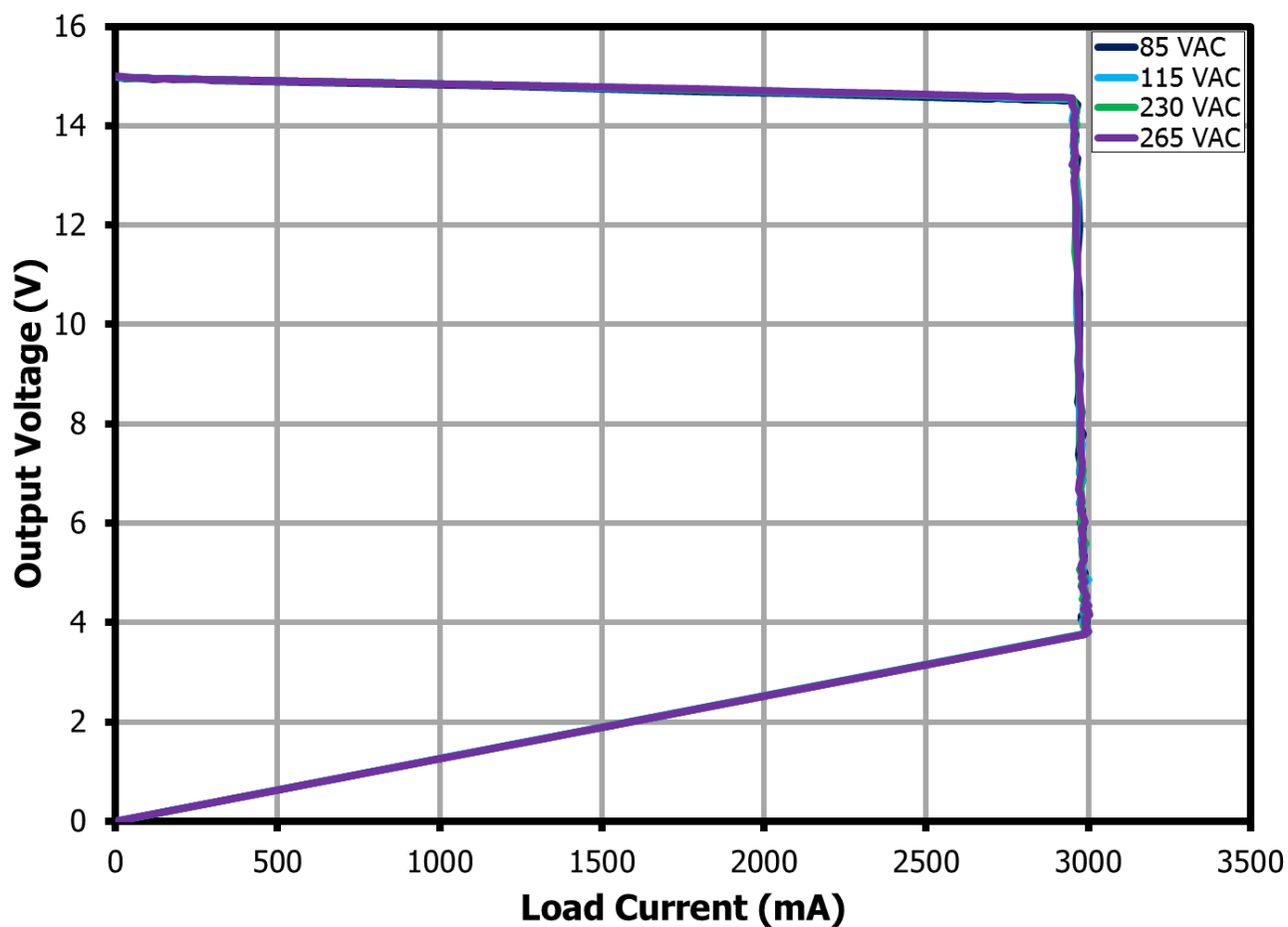
Figure 116 – CV/CC Profile with Output 15 V, 3 A.
