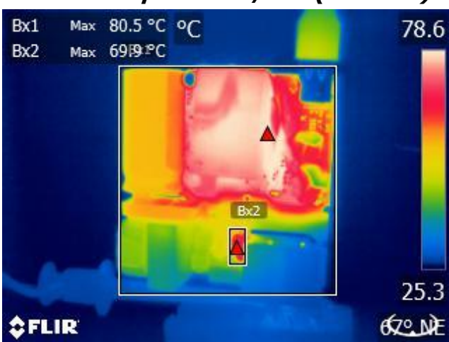
Figure 43 – Top Side Thermal Image. Ambient: 26.4 °C. Bx1: Transformer winding = 80.5 °C. Bx2: Thermistor RT1 = 69.9 °C.
