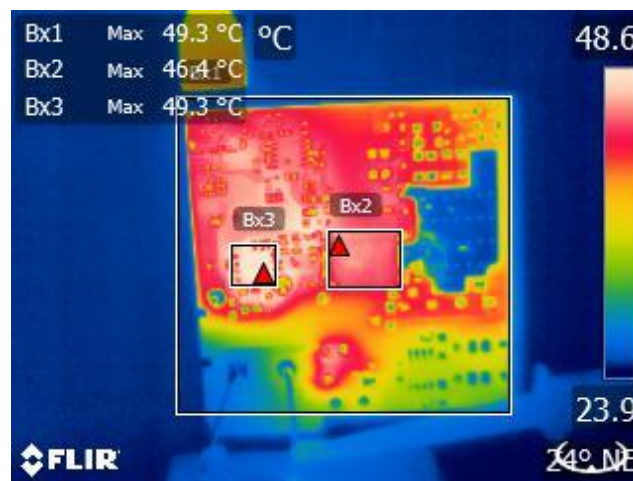
Figure 30 – Bottom Side Thermal Image. Ambient: 23.8 °C. Bx2: InnoSwitch3-Pro = 46.4 °C. Bx3: SR FET = 49.3 °C.
