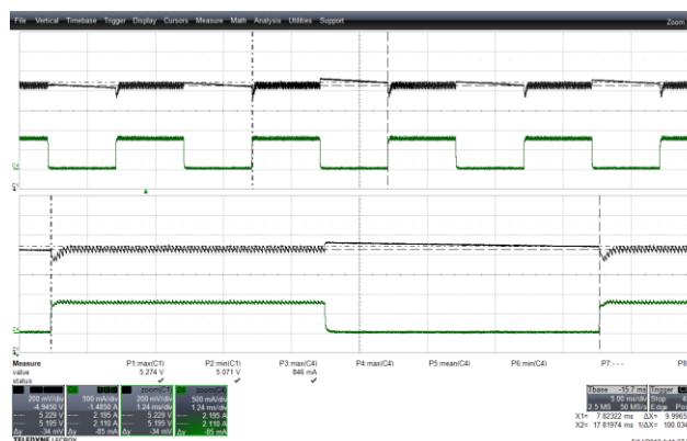
Figure 46 – Transient Response. 265 VAC, 5.0 V, 0 – 0.75 A Load Step. V_{MIN} : 5.071 V, V_{MAX} : 5.274 V. Upper: V OUT , 0.2 V / div., 5 ms / div. Lower: I LOAD , 0.5 A / div. Zoom: 1.24 ms / div.
