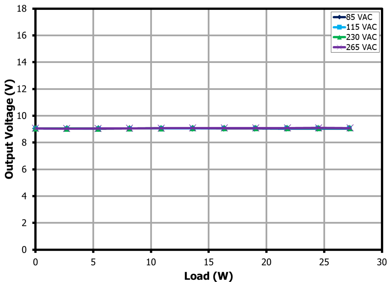
Figure 27 – Output Voltage vs. Output Load for 9 V Output, Room Temperature.
