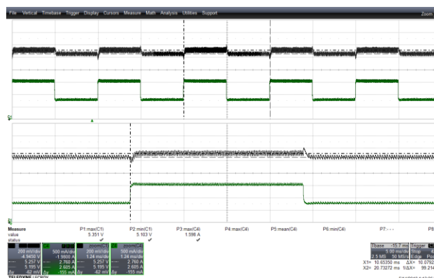
Figure 48 – Transient Response. 265 VAC, 5.0 V, 0.75 – 1.5 A Load Step. V_{MIN} : 5.103 V, V_{MAX} : 5.351 V. Upper: V OUT , 0.2 V / div., 5 ms / div. Lower: I LOAD , 0.5 A / div. Zoom: 1.24 ms / div.
