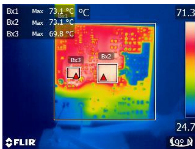
Figure 40 – Bottom Side Thermal Image. Ambient: 24.6 °C. Bx2: InnoSwitch3-Pro = 73.1 °C. Bx3: SR FET = 69.8 °C.
