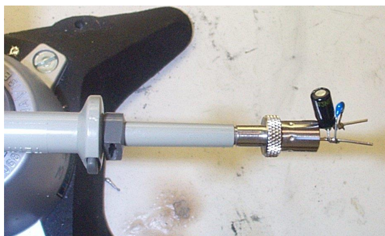
Figure 98 – Oscilloscope Probe with Probe Master ( www.probemaster.com ) 4987A BNC Adapter. (Modified with wires for ripple measurement, and two parallel decoupling capacitors added)
