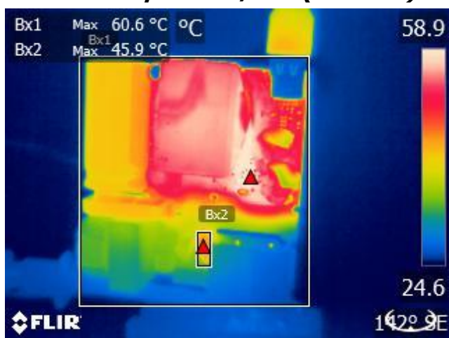
Figure 35 – Top Side Thermal Image. Ambient: 24.8 °C. Bx1: Transformer Winding = 60.6 °C. Bx2: Thermistor RT1 = 45.9 °C.
