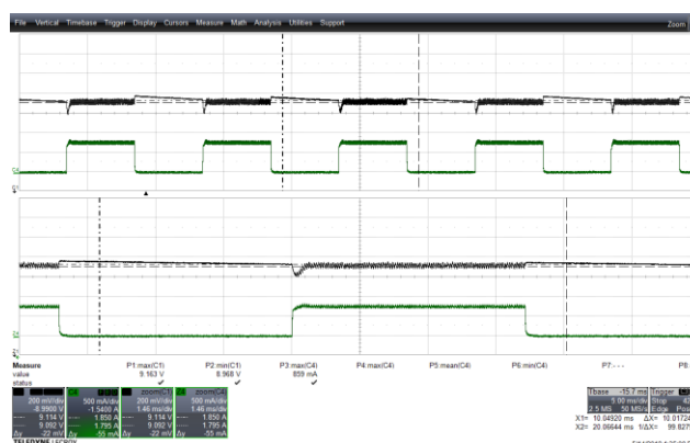
Figure 54 – Transient Response. 265 VAC, 9.0 V, 0 – 0.75 A Load Step. V_{MIN} : 8.968 V, V_{MAX} : 9.163 V. Upper: V_{OUT} , 0.2 V / div., 5 ms / div. Lower: I_{LOAD} , 0.5 A / div. Zoom: 1.46 ms / div.
