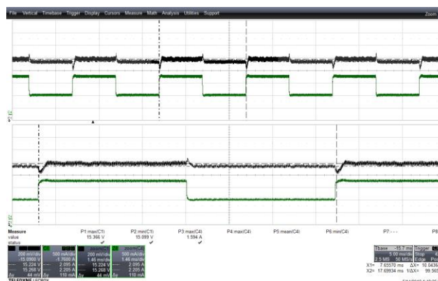
Figure 64 – Transient Response. 265 VAC, 15.0 V, 0.75 – 1.5 A Load Step. V_{MIN} : 15.099 V, V_{MAX} : 15.366 V. Upper: V_{OUT} , 0.2 V / div., 56 ms / div. Lower: I_{LOAD} , 0.5 A / div. Zoom: 1.46 ms / div.
