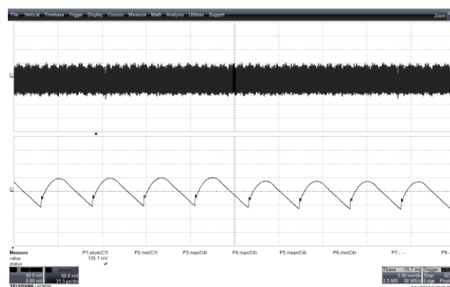
Figure 102 – Output Ripple. PK-PK = 135.1 mV. 265 VAC IN 5.0 V, 3 A Load. V OUT , 50 mV / div., 5 ms / div. Zoom: 31.5 \mu s / div.
