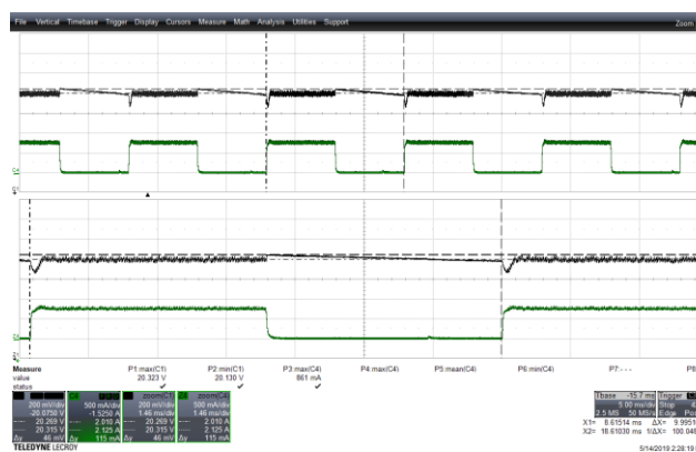
Figure 70 – Transient Response.
