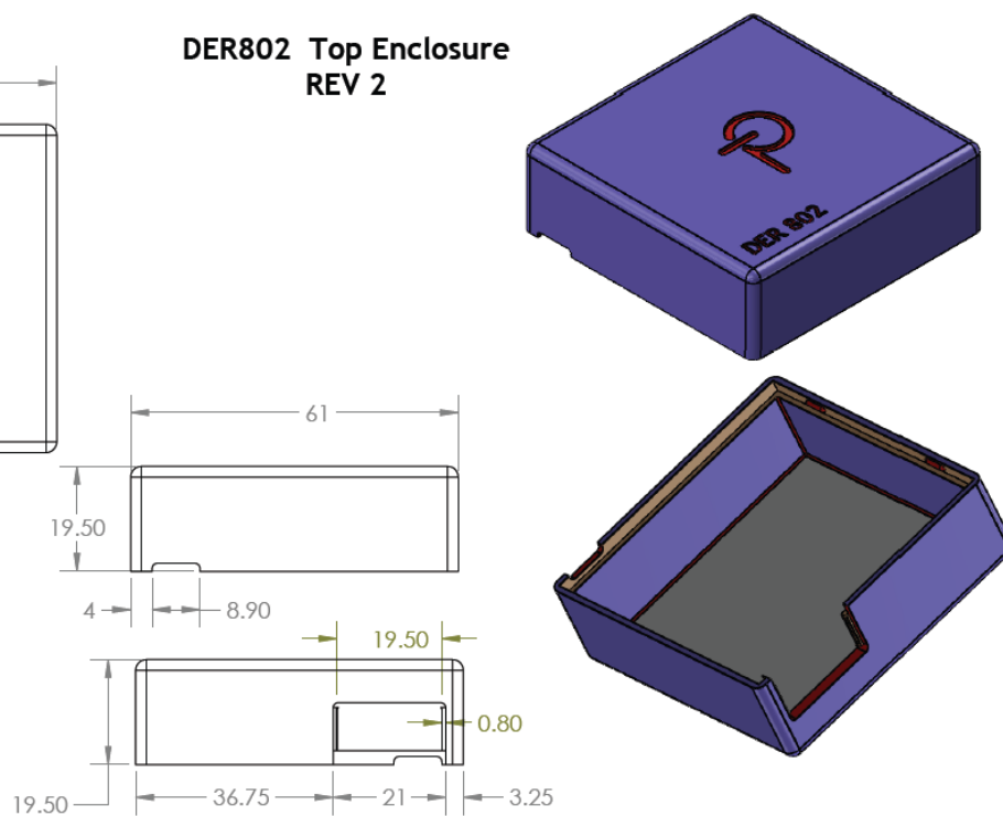
Figure 14 – DER-802 Adapter Case Top.
