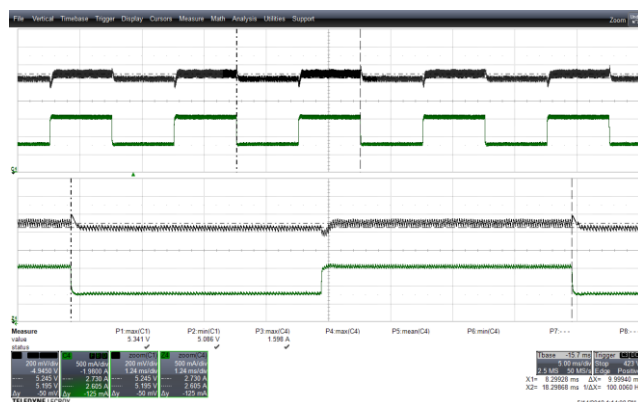
Figure 47 – Transient Response. 85 VAC, 5.0 V, 0.75 – 1.5 A Load Step. V_{MIN} : 5.086 V, V_{MAX} : 5.341 V. Upper: V OUT , 0.2 V / div., 5 ms / div. Lower: I LOAD , 0.5 A / div. Zoom: 1.24 ms / div.
