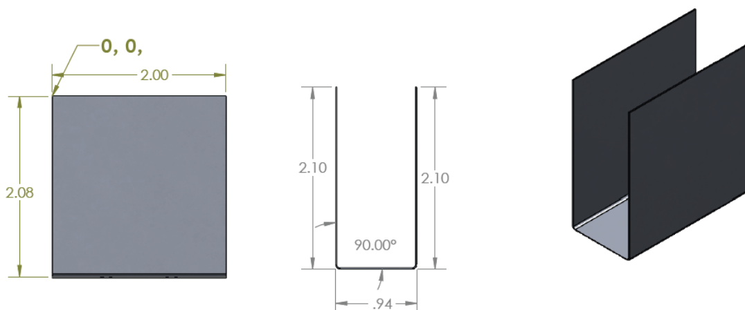
Figure 16 – Heat Spreader Drawing.
