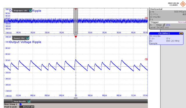
Figure 86 – Output Voltage Ripple Waveforms. 265 VAC, 80 mA Output. Ripple: 30 mV / div., 10 ms / div. Zoom: 300 \mu s / div. V_{PK-PK} : 65.217 mV.
