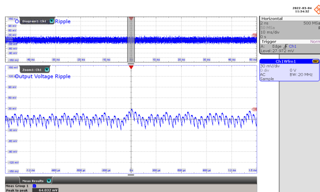
Figure 74 – Output Voltage Ripple Waveforms. 115 VAC, 400 mA Output. Ripple: 30 mV / div., 10 ms / div. Zoom: 300 \mu s / div. V_{PK-PK} : 64.032 mV.
