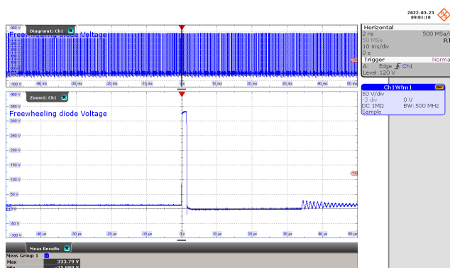
Figure 42 – Freewheeling Diode Voltage Waveforms. 230 VAC, 80 mA Output. Diode Voltage: 50 V / div., 10 ms / div. Zoom: 10 \mu s / div. V_{MAX} : 333.79 V.
