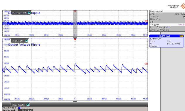
Figure 71 – Output Voltage Ripple Waveforms. 85 VAC, 80 mA Output. Ripple: 30 mV / div., 10 ms / div. Zoom: 300 \mu s / div. V_{PK-PK} : 52.174 mV.
