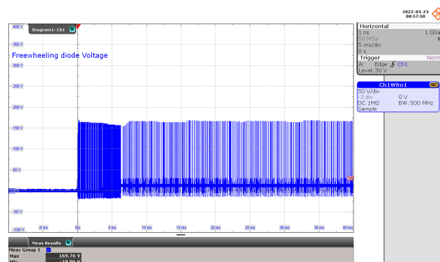
Figure 49 – Freewheeling Diode Voltage Waveforms. 115 VAC, 80 mA Output. Diode Voltage: 50 V / div., 5 ms / div. V_{MAX} : 169.76 V.
