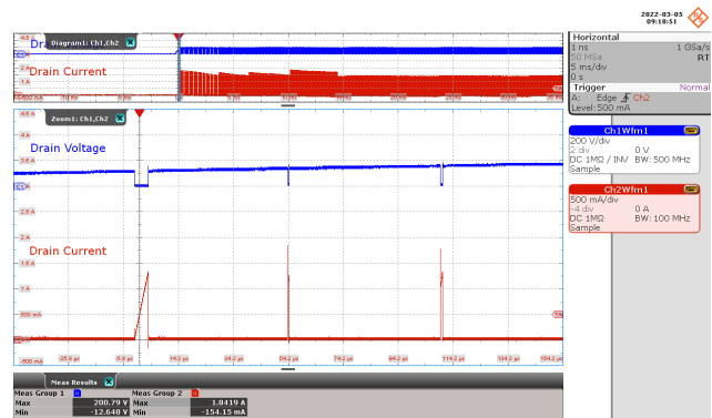
Figure 27 – Drain Voltage and Current Waveforms. 115 VAC, 800 mA Output. Drain Voltage: 200 V / div., 5 ms / div. Drain Current: 500 mA / div., 5 ms / div. Zoom = 20 \mu\text{s} / div. I_{\text{DS(MAX)}} = 1.84 \text{ A} , V_{\text{DS(MAX)}} = 200.79 \text{ V} .
