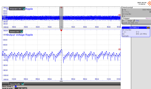
Figure 77 – Output Voltage Ripple Waveforms. 230 VAC, 800 mA Output. Ripple: 30 mV / div., 10 ms / div. Zoom: 300 \mu s / div. V_{PK-PK} : 91.304 mV.
