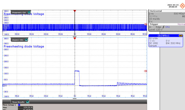
Figure 40 – Freewheeling Diode Voltage Waveforms. 85 VAC, 80 mA Output. Diode Voltage: 50 V / div., 10 ms / div. Zoom: 10 \mu s / div. V_{MAX} : 124.31 V.
