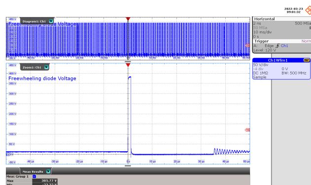
Figure 43 – Freewheeling Diode Voltage Waveforms. 265 VAC, 80 mA Output. Diode Voltage: 50 V / div., 10 ms / div. Zoom: 10 \mu s / div. V_{MAX} : 385.77 V.
