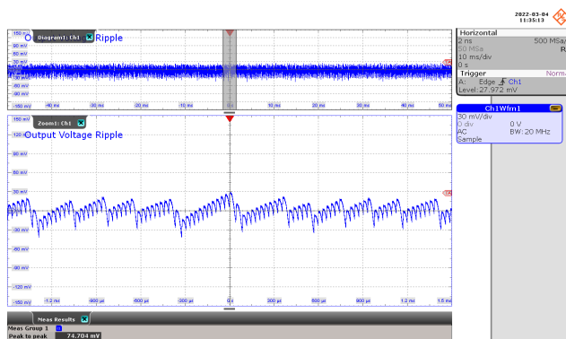
Figure 73 – Output Voltage Ripple Waveforms. 115 VAC, 600 mA Output. Ripple: 30 mV / div., 10 ms / div. Zoom: 300 \mu s / div. V_{PK-PK} : 74.704 mV.
