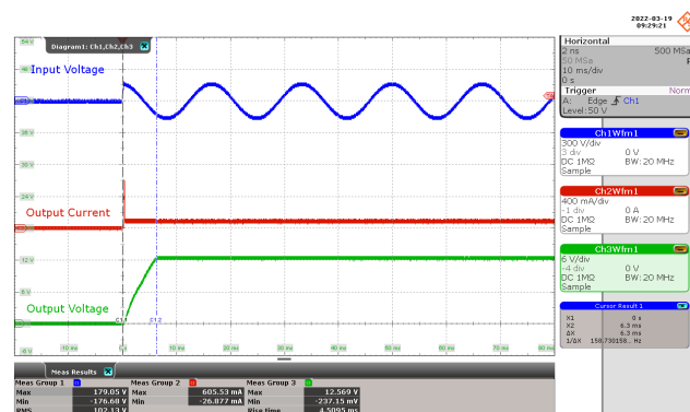
Figure 61 – Output Voltage and Current Waveforms. 115 VAC, 80 mA Output. Input Voltage: 300 V / div., 10 ms / div. Output Current: 400 mA / div., 10 ms / div. Output Voltage: 6 V / div., 10 ms / div. Rise Time = 4.5095 ms.
