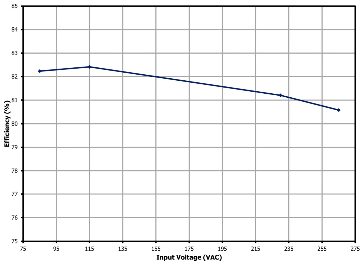
Figure 6 – Full Load (800 mA) Efficiency vs. Line Voltage, Room Temperature.
