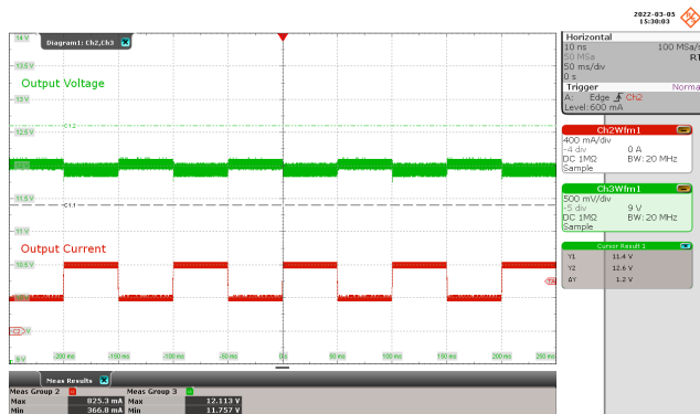
Figure 93 – Transient Output Waveforms. 265 VAC. Output Current: 400 mA / div., 50 ms / div. Output Voltage: 500 mV / div., 50 ms / div.. Load Transient: 50 % - 100%. Duty Cycle, Slew Rate: 50%, 0.8 A / \mu s. Frequency: 10 Hz. V_{MAX} : 12.113 V, V_{MIN} : 11.757 V.
