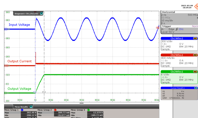
Figure 63 – Output Voltage and Current Waveforms. 265 VAC, 80 mA Output. Input Voltage: 300 V / div., 10 ms / div. Output Current: 400 mA / div., 10 ms / div. Output Voltage: 6 V / div., 10 ms / div. Rise Time = 4.1476 ms.
