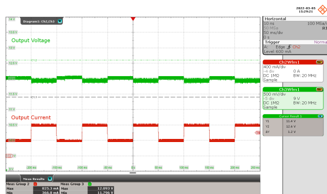
Figure 87 – Transient Output Waveforms. 85 VAC.
