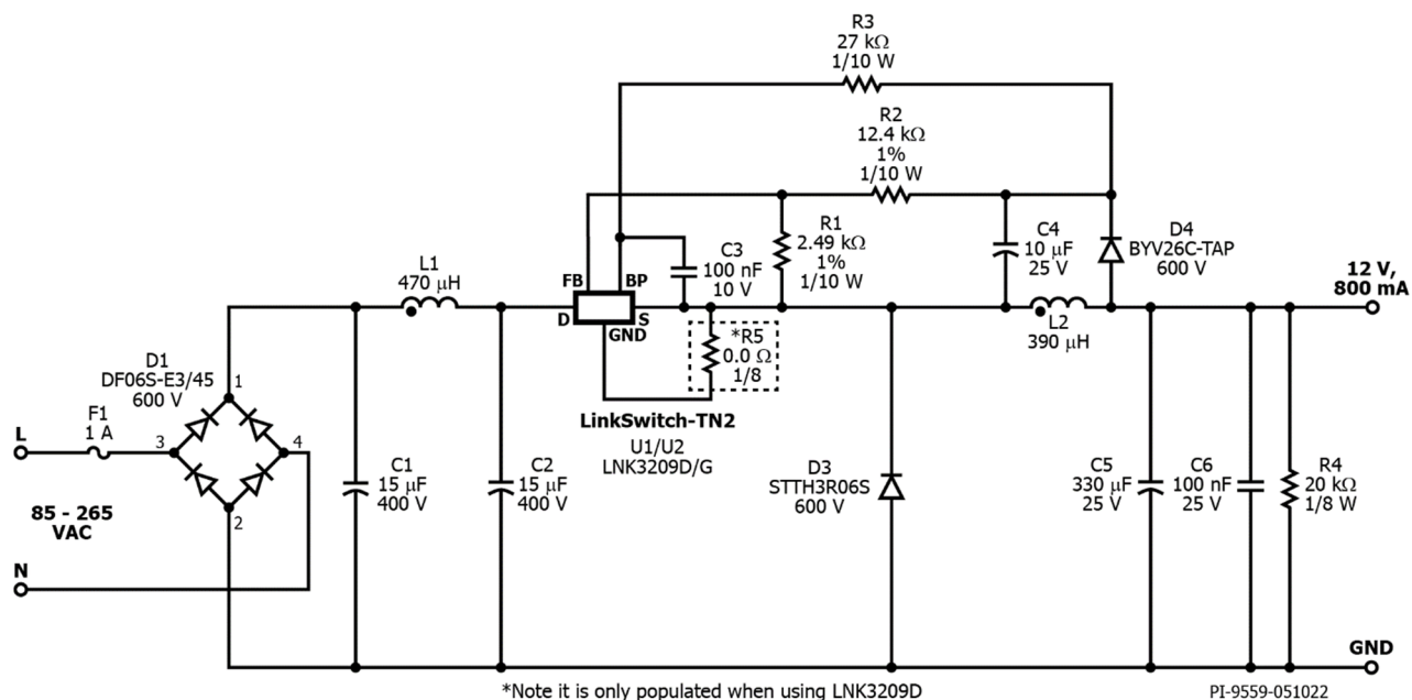
Figure 3 – Schematic.
