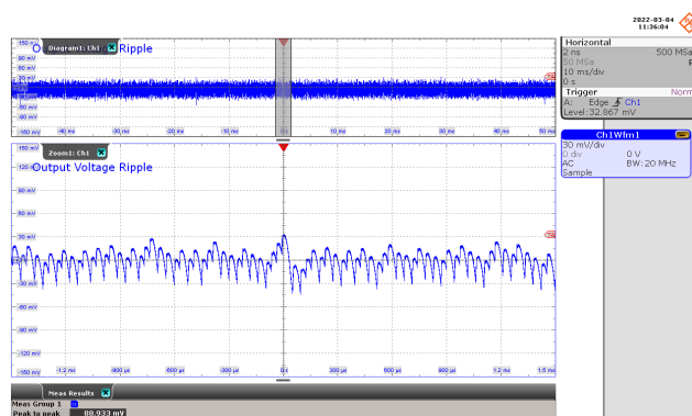
Figure 72 – Output Voltage Ripple Waveforms. 115 VAC, 800 mA Output. Ripple: 30 mV / div., 10 ms / div. Zoom: 300 \mu s / div. V_{PK-PK} : 88.933 mV.
