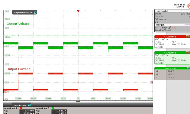
Figure 90 – Transient Output Waveforms. 115 VAC.
