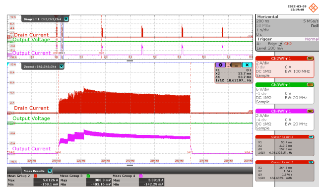
Figure 35 – Drain Current and Output Waveforms. 265 VAC Input.
