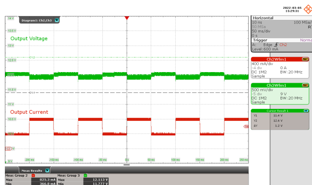
Figure 89 – Transient Output Waveforms. 115 VAC.
