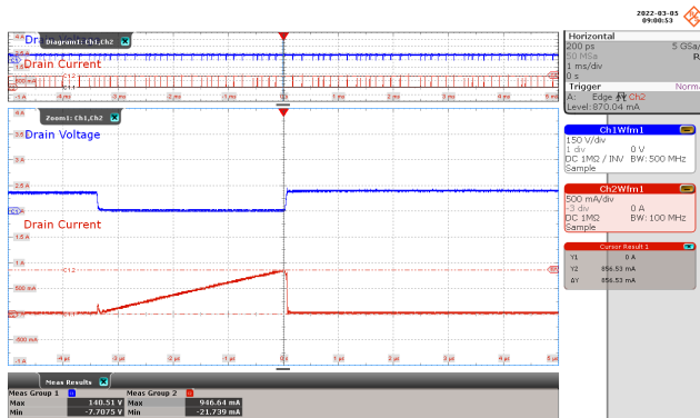
Figure 22 – Drain Voltage and Current Waveforms. 85 VAC, 80 mA Output. Drain Voltage: 150 V / div., 1 ms / div. Drain Current: 500 mA / div., 1 ms / div. Zoom = 1 μs / div. I_{DS(MAX)} = 946.64 \text{ mA} , V_{DS(MAX)} = 140.51 \text{ V} .
