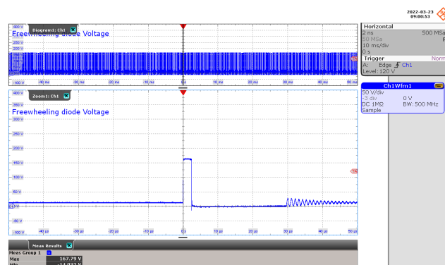
Figure 41 – Freewheeling Diode Voltage Waveforms. 115 VAC, 80 mA Output. Diode Voltage: 50 V / div., 10 ms / div. Zoom: 10 \mu s / div. V_{MAX} : 167.79 V.
