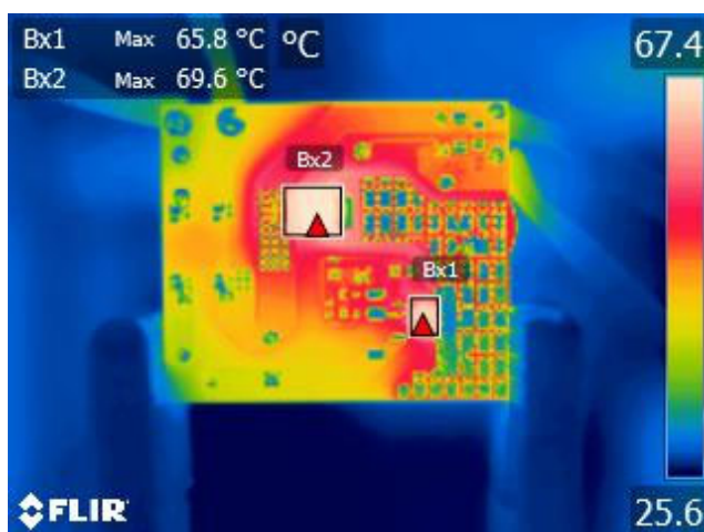
Figure 14 – LNK3209D (Bx1), 65.8 °C. Buck Diode (Bx2), 69.6 °C. 85 VAC, 800 mA Output.
