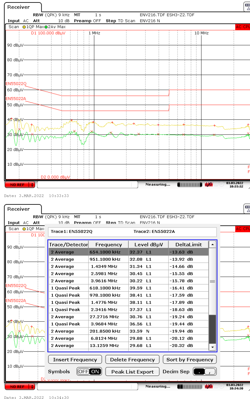
Figure 95 – 115 VAC Floating Ground EMI.
