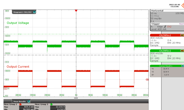
Figure 88 – Transient Output Waveforms. 85 VAC.
