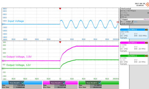
Figure 41 – 85 VAC Input.
