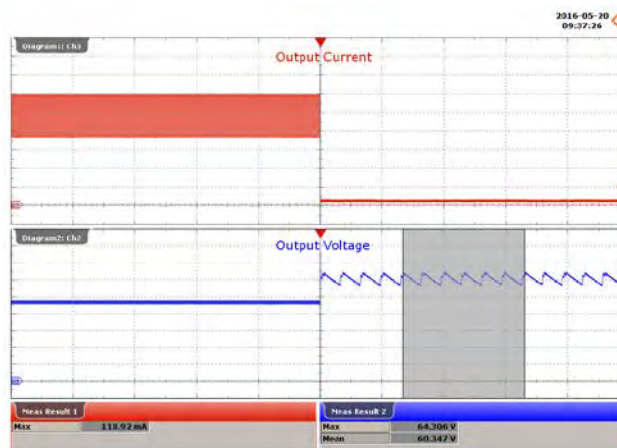
Figure 92 – 300 VAC, Open Load. Running Open Load. Upper: I_{OUT} , 20 mA / div. Lower: V_{OUT} , 10 V / div., 4 s / div.
