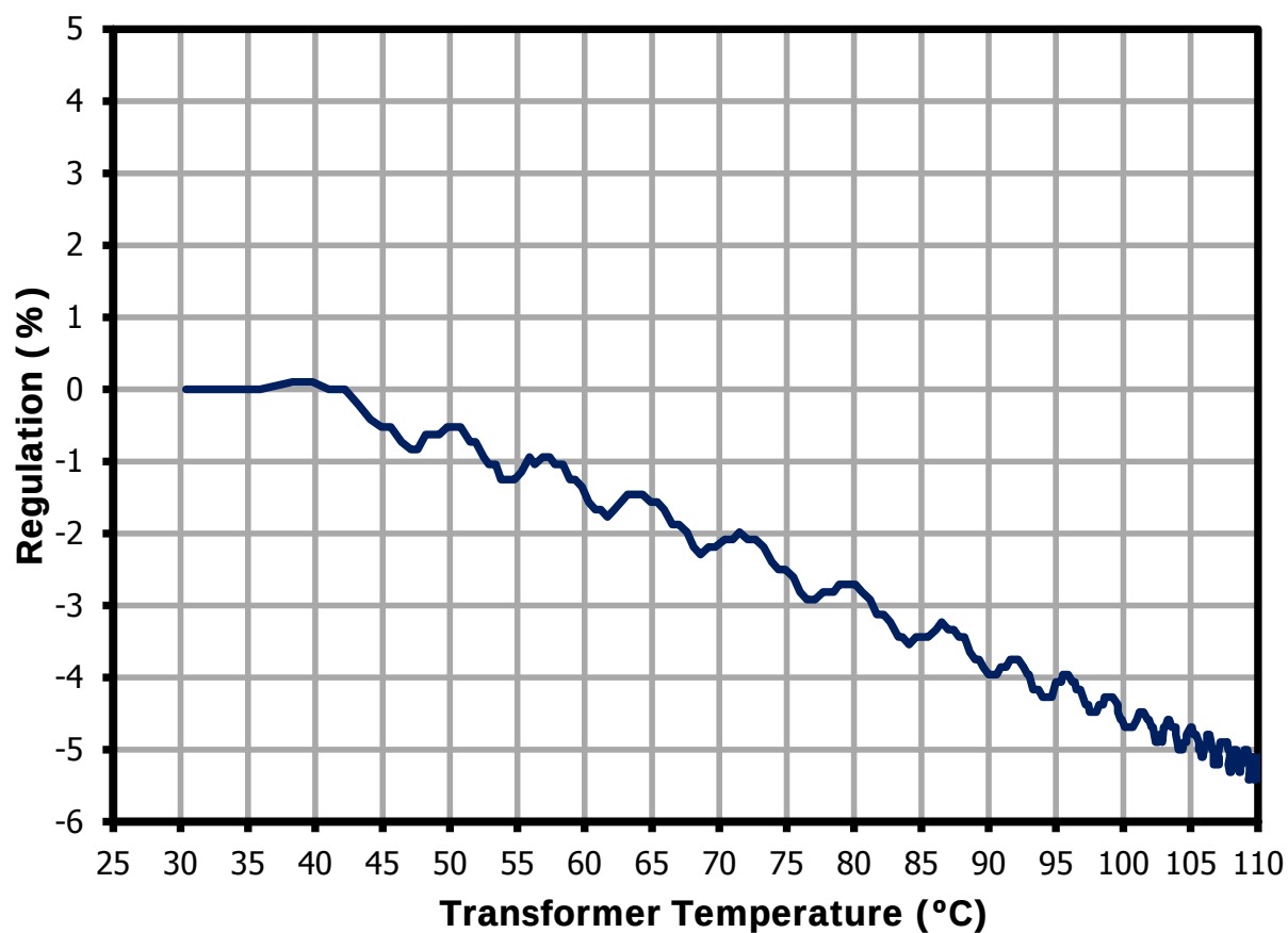
Figure 51 – Output Current Regulation vs. IC Temperature, 230 VAC, 48 V LED Load, 85 °C Ambient.
