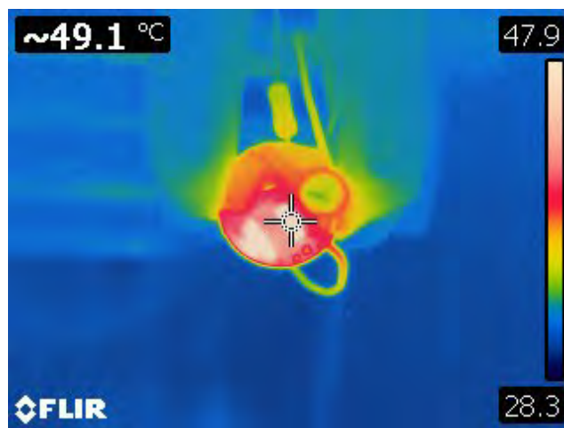
Figure 44 – 230 VAC, Output Short. Spot 1: Inductor (T1): 49.1 °C.
