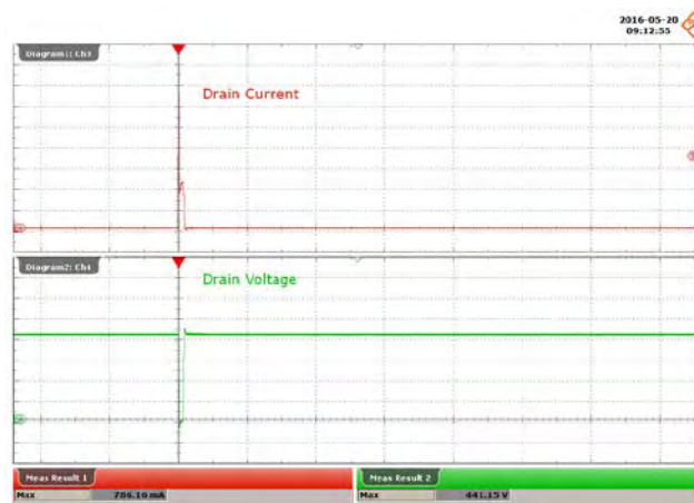
Figure 80 – 300 VAC, 48 V LED Load. Upper: I_{DRAIN} , 100 mA / div. Lower: V_{DRAIN} , 100 V / div., 4 \mu s / div.
