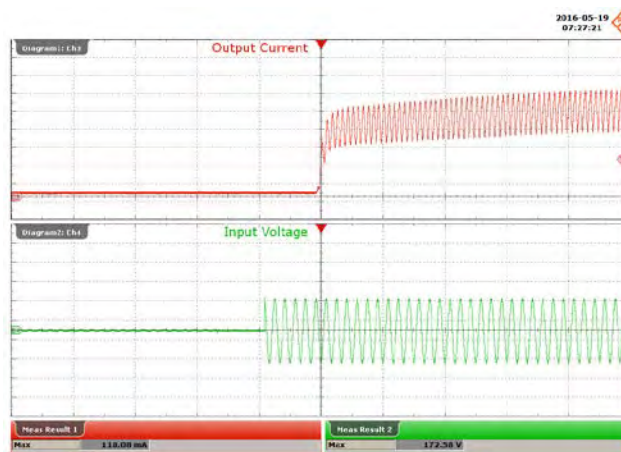
Figure 60 – 115 VAC, 48 V LED, Output Rise. Upper: I_{OUT} , 40 mA / div. Lower: V_{IN} , 100 V / div., 100 ms / div.
