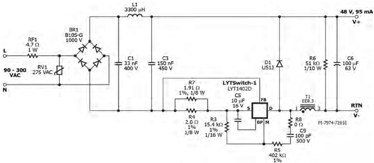
Figure 4 – Schematic.
