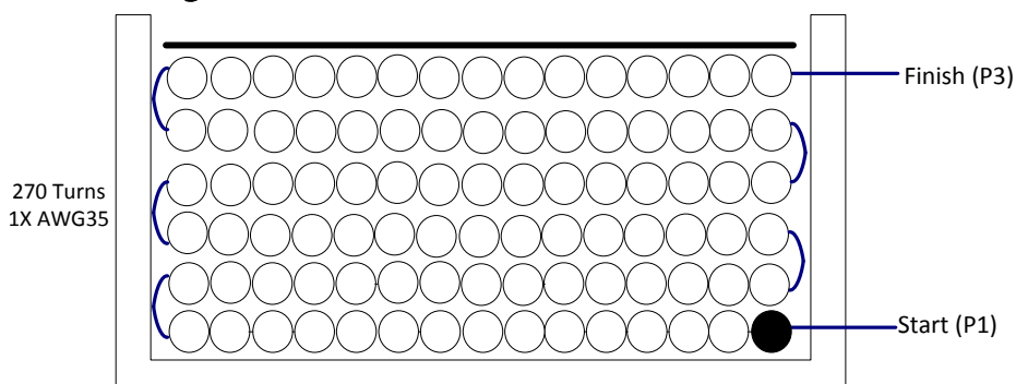
Figure 8 – Transformer Build Diagram.
