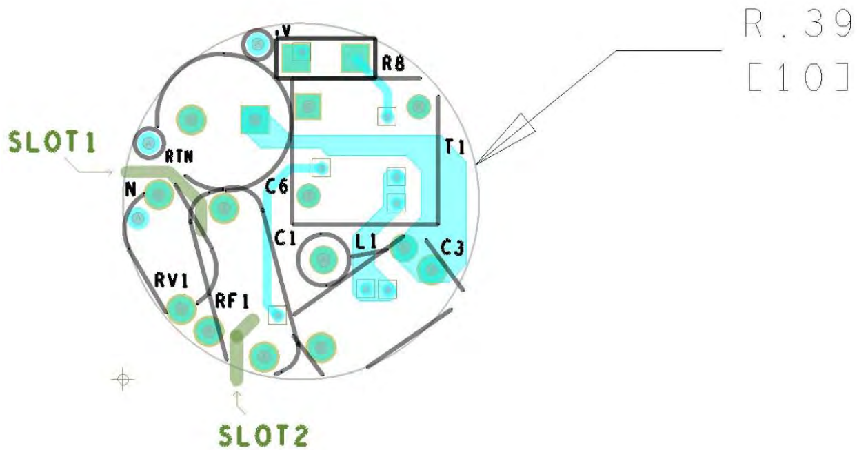
Figure 5 – Top Side.
