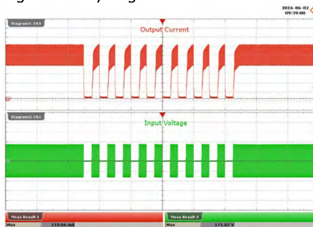
Figure 104 – 115 VAC, 48 V LED Load. 0.5 s On – 0.5 s Off. Upper: I_{OUT} , 20 mA / div. Lower: V_{IN} , 100 V / div., 2 s / div.
