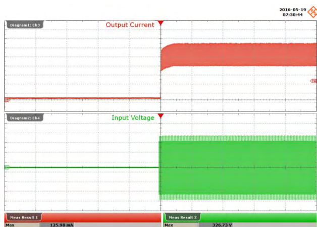
Figure 61 – 230 VAC, 48 V LED, Output Rise. Upper: I_{OUT} , 40 mA / div. Lower: V_{IN} , 100 V / div., 1 s / div.
