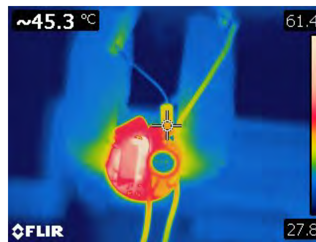
Figure 19 – 90 VAC, 48 V LED Load. Spot 1: Fusible Resistor (RF1): 45.3 °C.
