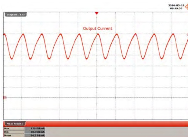
Figure 100 – 300 VAC, 60 Hz, 48 V LED Load. Upper: I_{OUT} , 50 mA / div., 10 ms / div.
