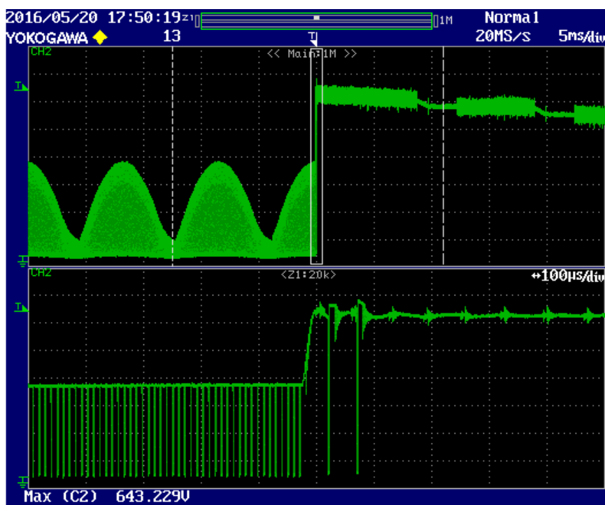
Figure 116 – +500 V Differential Surge, 90° Phase Angle.
