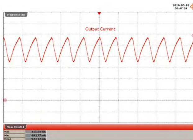
Figure 98 – 115 VAC, 60 Hz, 48 V LED Load. Upper: I_{OUT} , 20 mA / div., 10 ms / div.
