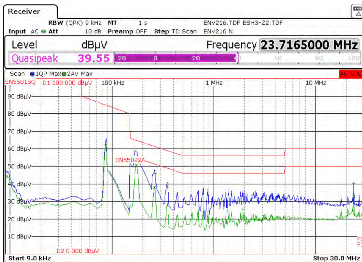
Figure 114 – Conducted EMI QP Scan at 48 V LED Load, 230 VAC, 50 Hz, and EN55015 B Limits.
