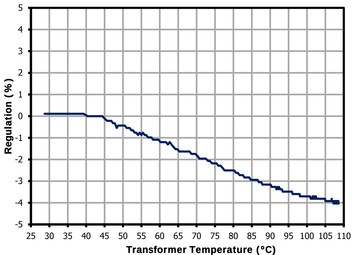
Figure 49 – Output Current Percent Regulation vs IC Temperature, 115 VAC, 48 V LED Load, 85 °C Ambient.
