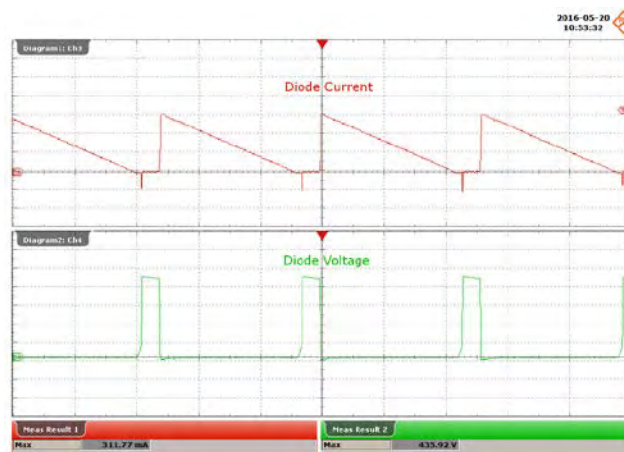
Figure 88 – 300 VAC, 48 V LED Load. Upper: I_{D1} , 100 mA / div. Lower: V_{D1} , 100 V / div., 4 \mu s / div.
