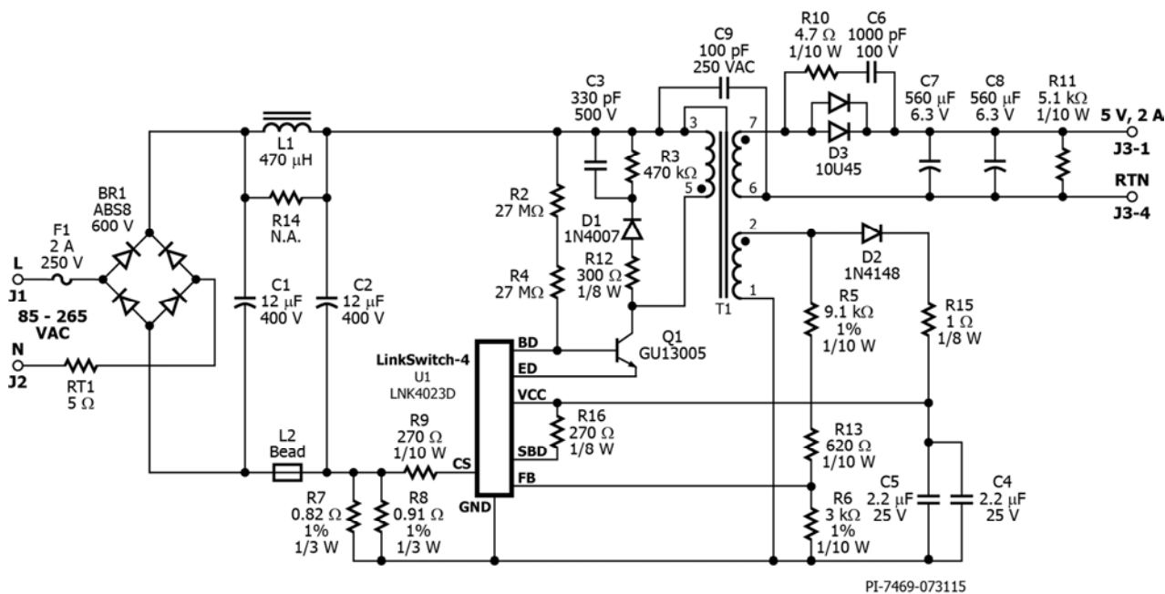
Figure 3 – Schematic.
