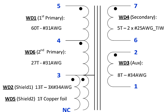
Figure 6 –Transformer Electrical Diagram.
