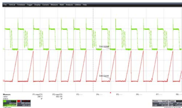
Figure 29 – Drain Voltage and Current Waveforms. 90 VAC, 2 A Load, 296 V MAX . Upper: V DRAIN , 100 V, 20 \mu s / div. Lower: I DRAIN , 200 mA / div.
