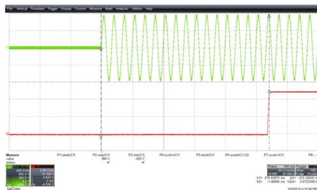
Figure 34 – Input AC and Output Waveforms. Start-up Time = 272.3 ms. 265 VAC, Zero Load. Upper: V_{ACr} 200 V, 50 ms / div. Lower: V_{OUT} , 2 V / div.
