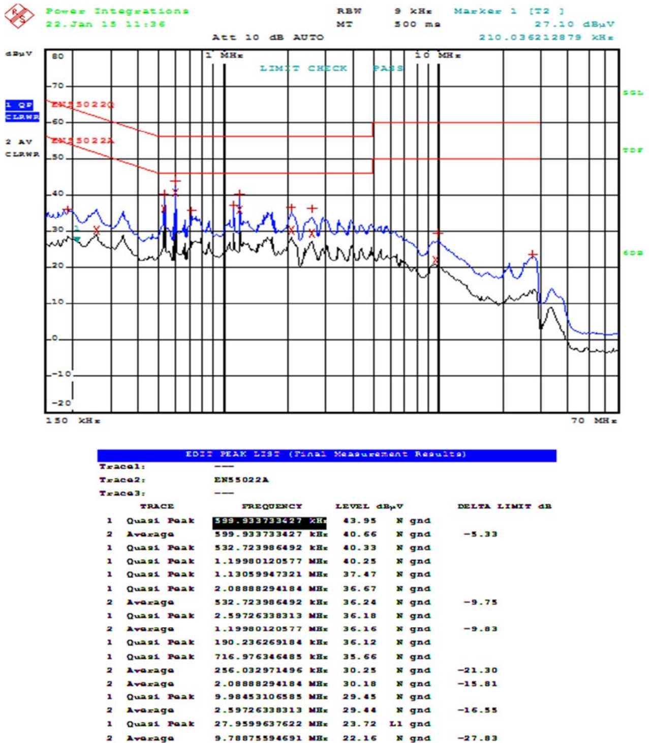
Figure 39 – Floating Ground at 230 VAC.
