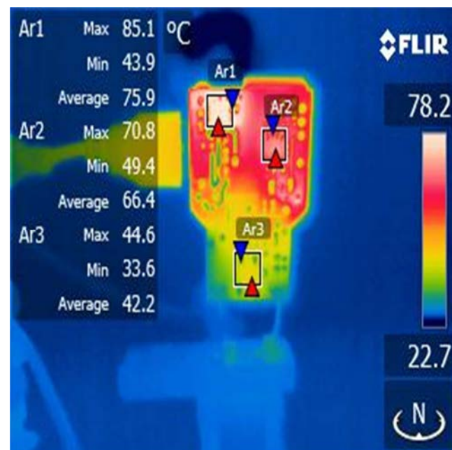
Figure 18 – LinkSwitch-4 Side. 230 VAC, 2 A Load. Ambient 25.7 °C, Schottky 85.1 °C, LinkSwitch-4 70.8 °C, Bridge 44.6 °C.
