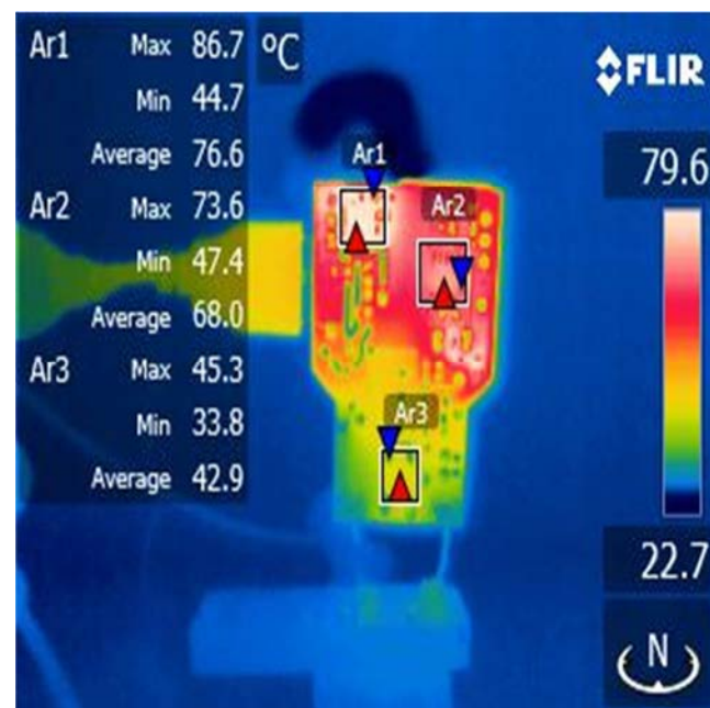
Figure 20 – LinkSwitch-4 Side. 265 VAC, 2 A Load. Ambient 25.7 °C, Schottky 86.7 °C, Link4 73.6 °C, Bridge 45.3 °C.
