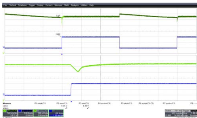
Figure 27 – Transient Response ( 4.35\text{ V}_{\text{MIN}} ). 230 VAC, 0-2 A Load Step. Upper: I_{\text{LOAD}} , 1 A / div. Lower: V_{\text{OUT}} , 500 mV, 50 ms / div.
