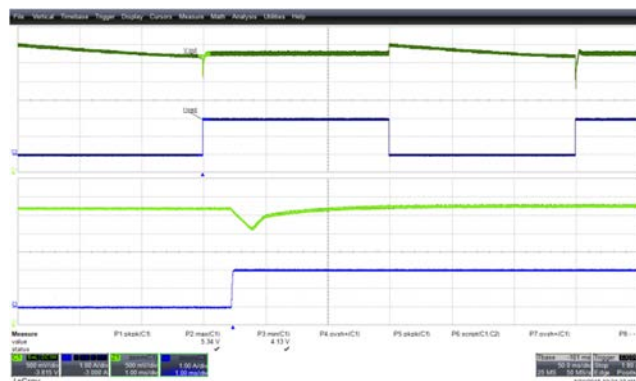
Figure 28 – Transient Response ( 4.13\text{ V}_{\text{MIN}} ). 265 VAC, 0-2 A Load Step. Upper: I_{\text{LOAD}} , 1 A / div. Lower: V_{\text{OUT}} , 500 mV, 50 ms / div.
