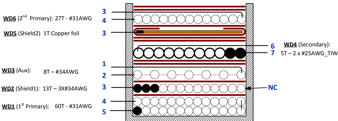
Figure 7 – Transformer Build Diagram.
