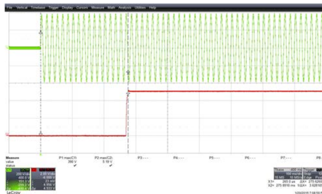
Figure 32 – Input AC and Output Waveforms. Start-up Time = 275.6 ms 265 VAC, 2.5 \Omega Load. Upper: V AC , 200 V, 100 ms / div. Lower: V OUT , 2 V / div.
