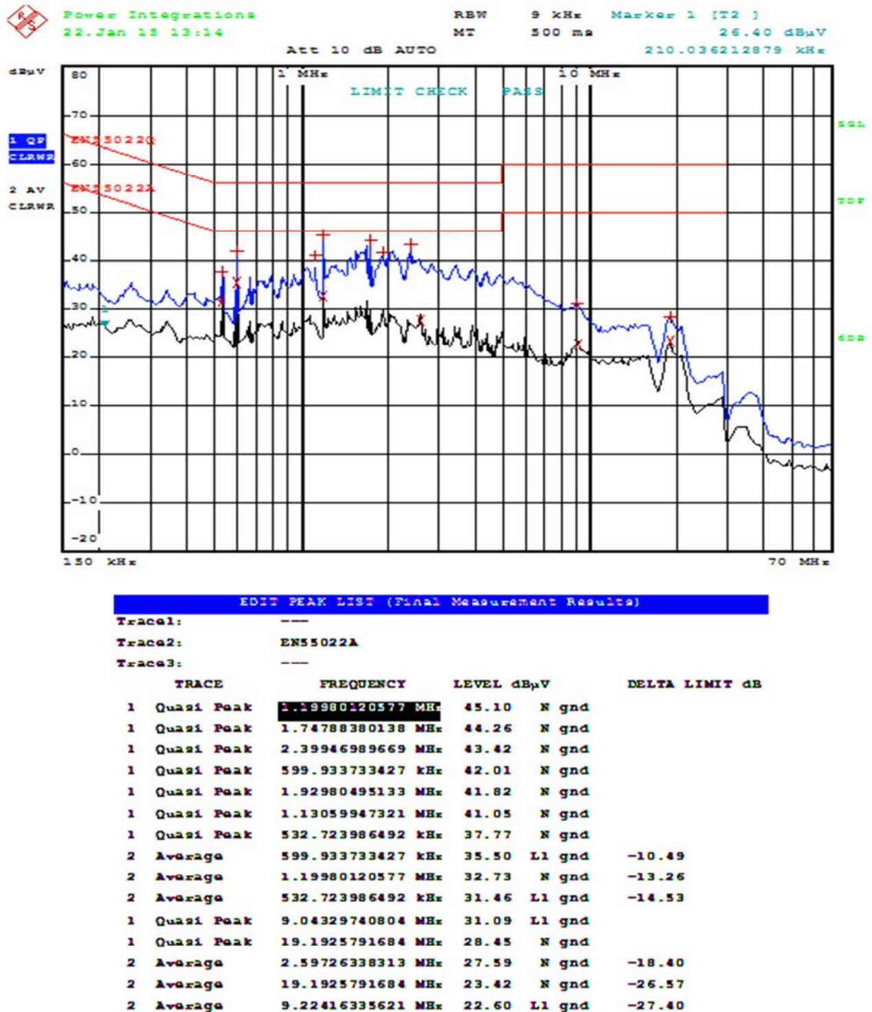
Figure 41 – Artificial Ground at 230 VAC.
