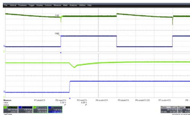
Figure 26 – Transient Response ( 4.28\text{ V}_{\text{MIN}} ). 115 VAC, 0-2 A Load Step. Upper: I_{\text{LOAD}} , 1 A / div. Lower: V_{\text{OUT}} , 500 mV, 50 ms / div.
