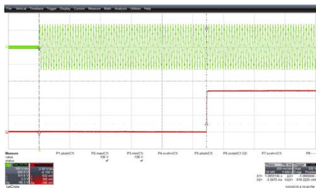
Figure 33 – Input AC and Output Waveforms. Start-up Time = 1.1 s. 90 VAC, Zero Load. Upper: V_{ACr} 100 V, 200 ms / div. Lower: V_{OUT} , 2 V / div.
