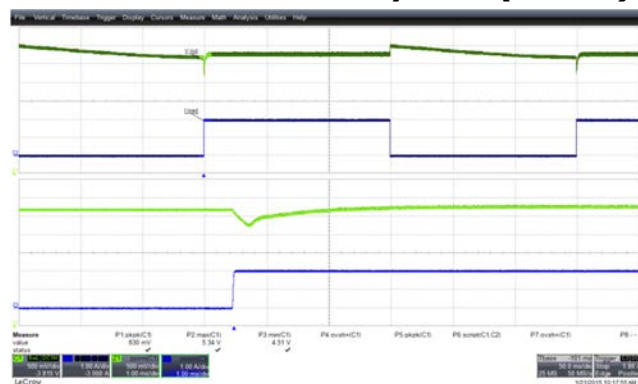
Figure 25 – Transient Response ( 4.51\text{ V}_{\text{MIN}} ). 90 VAC, 0-2 A Load Step. Upper: I_{\text{LOAD}} , 1 A / div. Lower: V_{\text{OUT}} , 500 mV, 50 ms / div.
