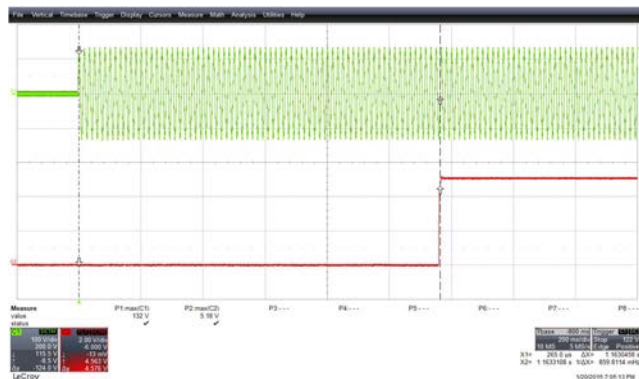
Figure 31 – Input AC and Output Waveforms. Start-up Time = 1.16 s 90 VAC, 2.5 \Omega load Upper: V AC , 100 V, 200 ms / div. Lower: V OUT , 2 V / div.
