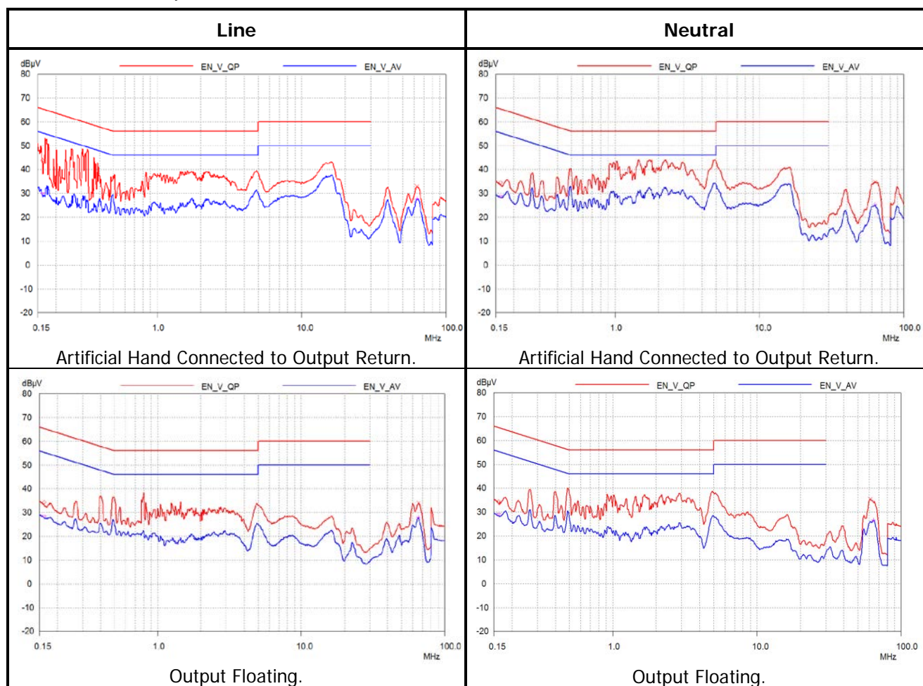
Figure 27 — Conducted EMI at 115 VAC.
