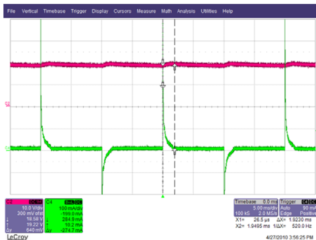
Figure 36 – 230 VAC, 34° Phase. Upper: V_{OUT} , 10 V / div. Lower: I_{IN} , 0.1 A / div., 5 ms / div.
