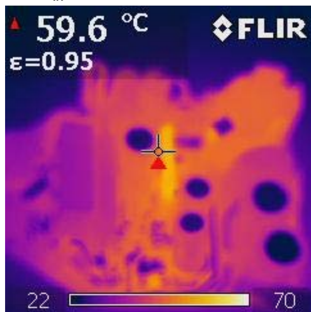
Figure 11 – Top Side.
