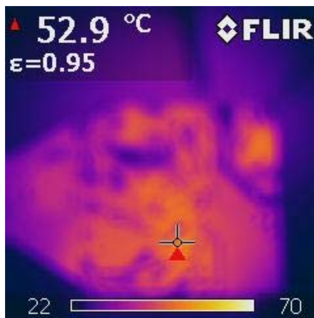
Figure 14 – Bottom Side.
