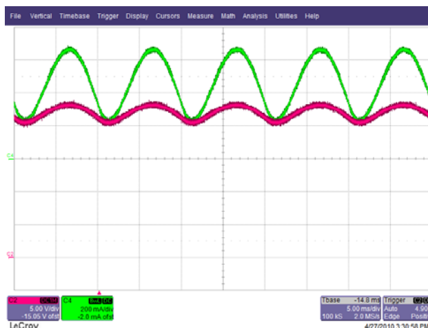
Figure 22 – 265 VAC, Full Load. Upper: I_{RIPPLE} , 0.2 A / div. Lower: V_{OUTPUT} 5 V, 5 ms / div.
