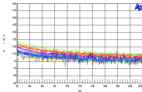
Figure 41 – 2 kHz – 22 kHz.
