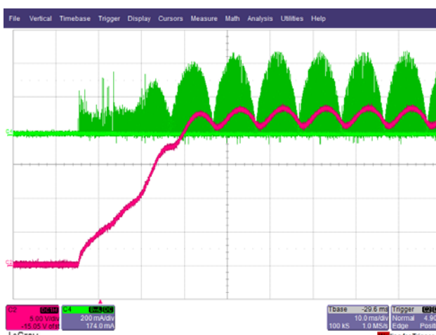
Figure 24 – 265 VAC, Full Load. Upper: I_{RIPPLE} , 0.2 A / div. Lower: V_{OUTPUT} , 5 V, 10 ms / div.
