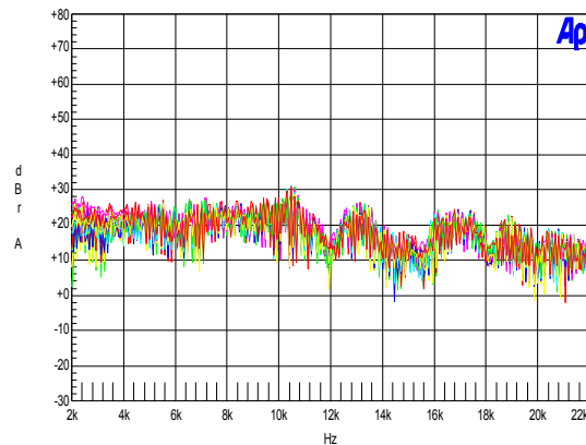
Figure 44 – 2 kHz – 22 kHz.
