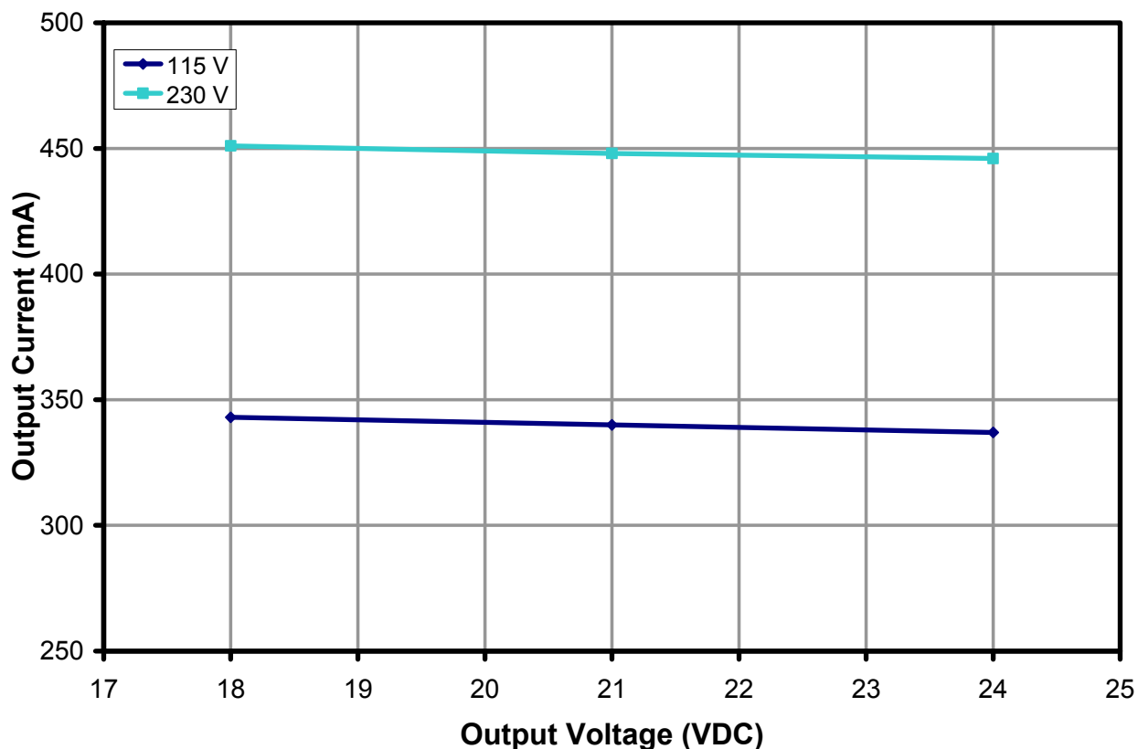
Figure 8 – Voltage and Line Regulation, Room Temperature.
