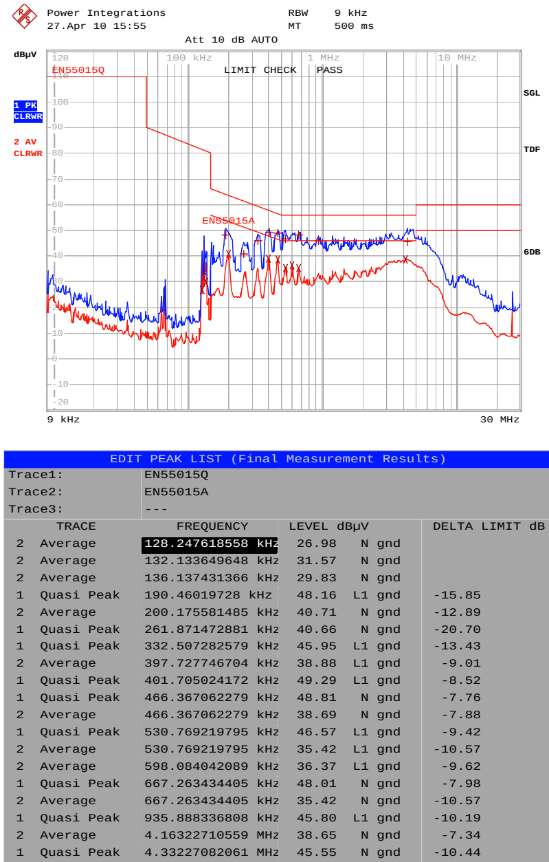
Figure 38 – Conducted EMI, Maximum Steady State Load, 115 VAC, 60 Hz, and EN55015 B Limits.
