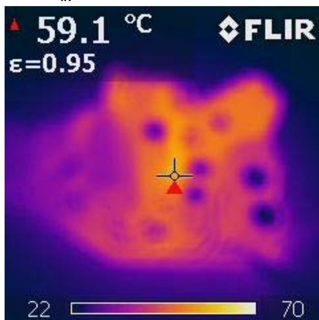
Figure 13 – Top Side.
