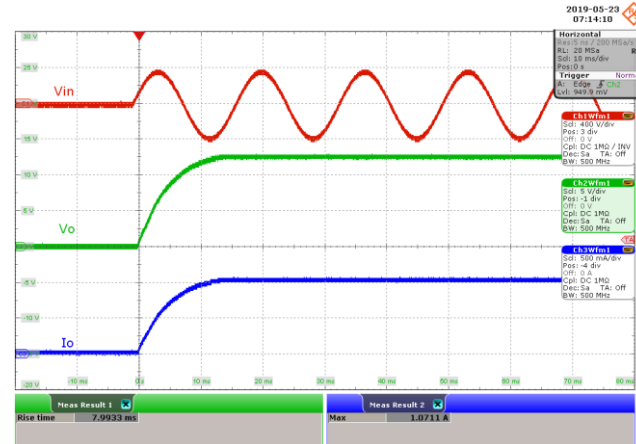
Figure 34 – 265 VAC 50 Hz.
