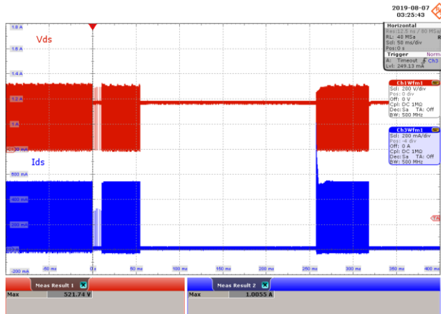
Figure 93 – 265 VAC 50 Hz.
