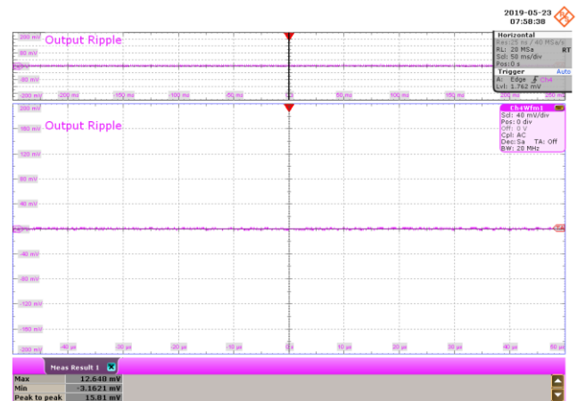
Figure 124 – 265 VAC 50 Hz.
