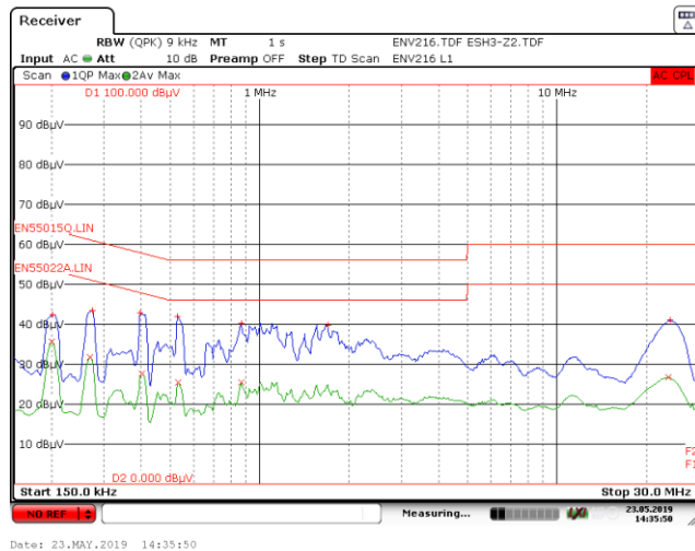
Figure 137 – 230 VAC 60 Hz, Line with Artificial Hand.
