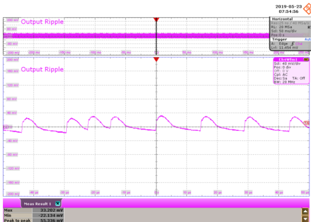
Figure 111 – 230 VAC 50 Hz.
