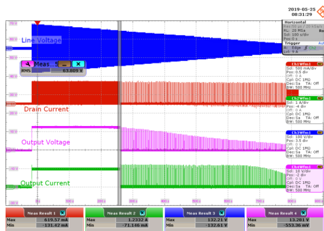
Figure 72 – Brown-Out, Full Load.
