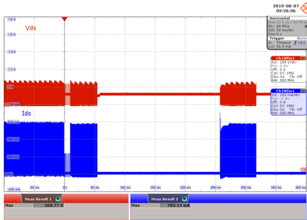
Figure 91 – 85 VAC 60 Hz.
