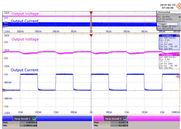
Figure 17 – 230 VAC 50 Hz.
