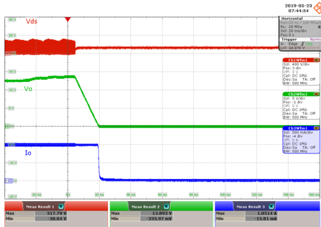
Figure 75 – 85 VAC 60 Hz.
