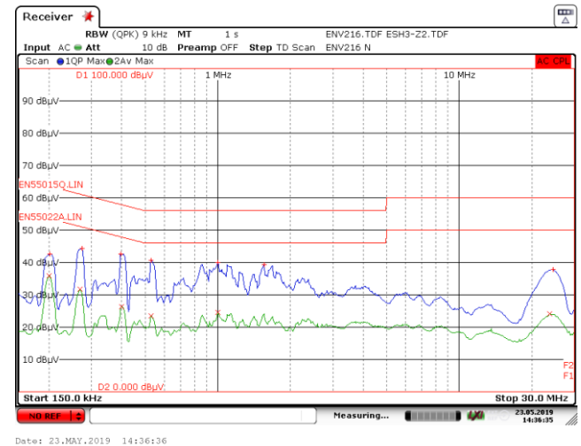
Figure 138 – 230 VAC 60 Hz, Neutral with Artificial Hand.
