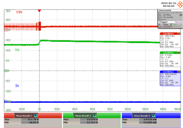
Figure 84 – 85 VAC 60 Hz, No-Load.
