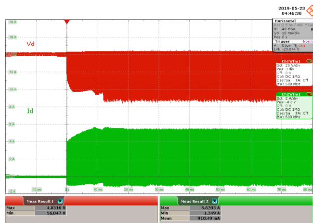
Figure 64 – 115 VAC 60 Hz.
