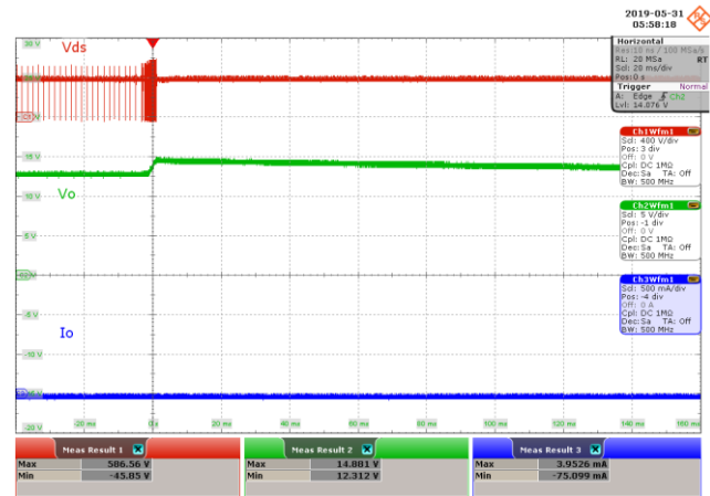
Figure 86 – 265 VAC 50 Hz, No-Load.
