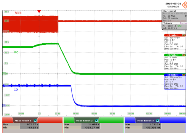
Figure 85 – 265 VAC 50 Hz, Full Load.
