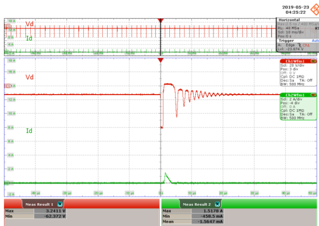
Figure 61 – 230 VAC 50 Hz.
