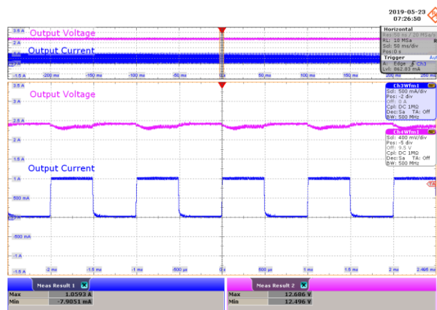
Figure 18 – 265 VAC 50 Hz.
