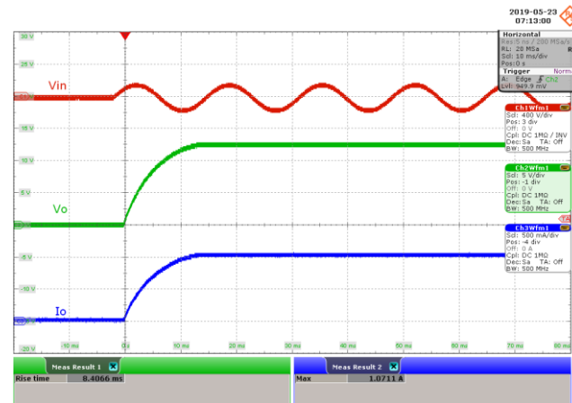
Figure 32 – 115 VAC 60 Hz.
