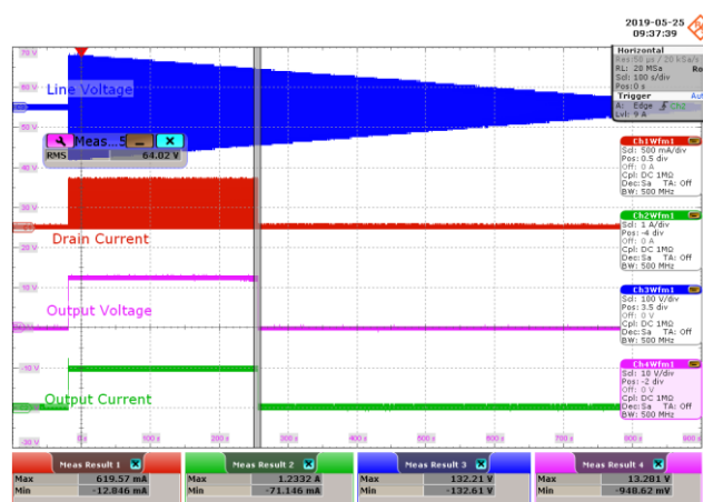
Figure 74 – Brown-In, Full Load.
