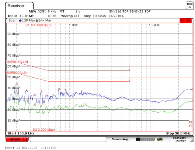
Figure 136 – 115 VAC 60 Hz, Neutral with Artificial Hand.
