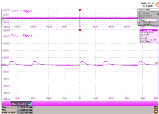
Figure 117 – 85 VAC 60 Hz.
