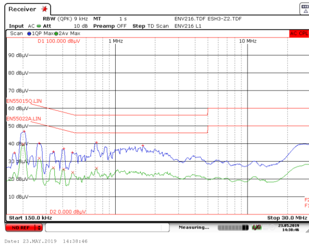
Figure 135 – 115 VAC 60 Hz, Line with Artificial Hand.
