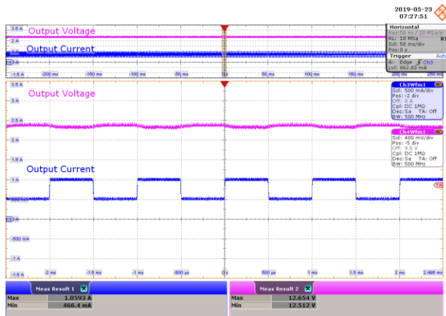
Figure 21 – 230 VAC 50 Hz.
