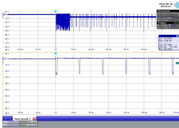
Figure 97 – 230 VAC 50 Hz, Full Load.
