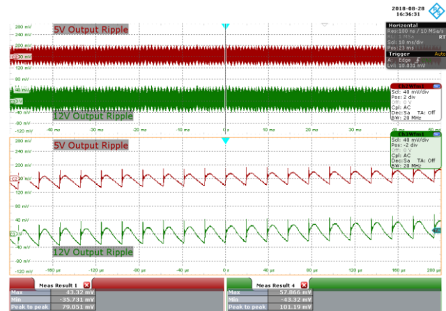
Figure 117 – 277 VAC 50 Hz, 75% Load.
