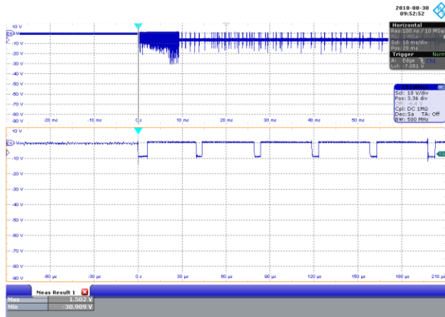
Figure 95 – 85 VAC 60 Hz, Full Load.
