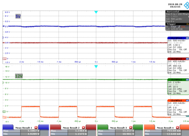
Figure 33 – 230 VAC 50 Hz.
