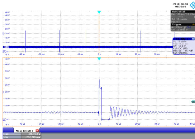
Figure 73 – 230 VAC 50 Hz, No-Load.
