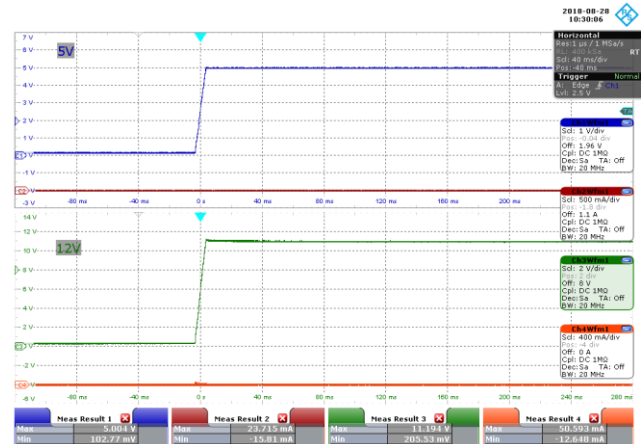
Figure 42 – 277 VAC 50 Hz, No-Load Start-up.
