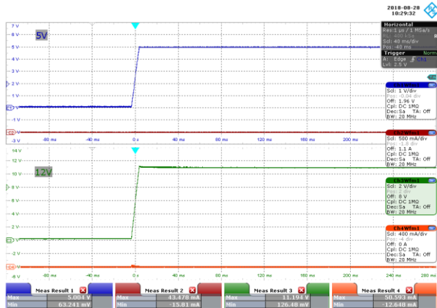
Figure 41 – 230 VAC 50 Hz, No-Load Start-up.
