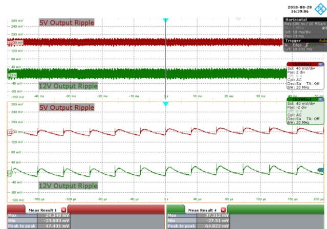
Figure 123 – 115 VAC 60 Hz, 25% Load.
