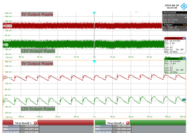
Figure 120 – 230 VAC 50 Hz, 50% Load.
