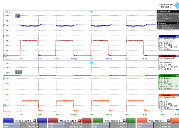
Figure 20 – 115 VAC 60 Hz.
