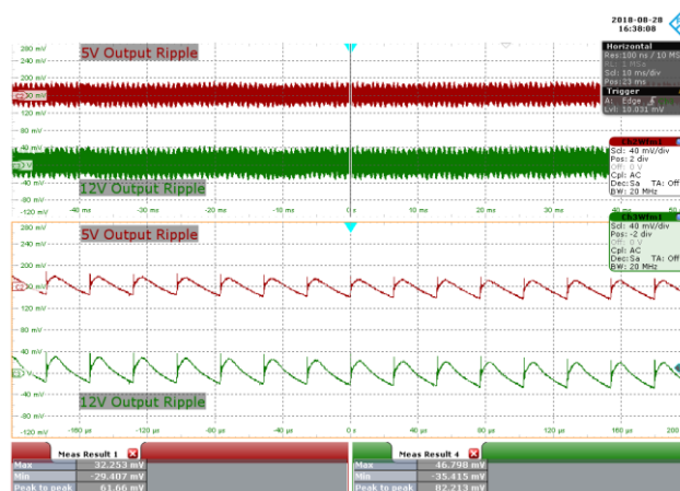
Figure 121 – 277 VAC 50 Hz, 50% Load.
