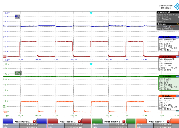
Figure 21 – 230 VAC 50 Hz.
