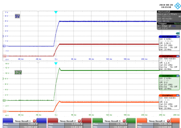
Figure 45 – 230 VAC 50 Hz, Full Load Start-up.
