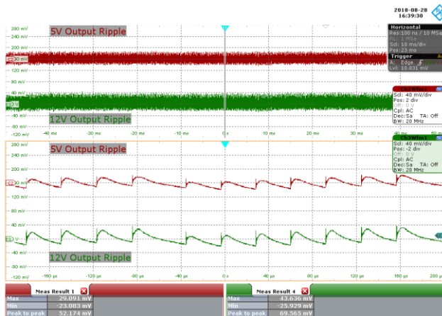
Figure 124 – 230 VAC 50 Hz, 25% Load.
