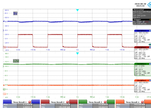
Figure 30 – 277 VAC 50 Hz.
