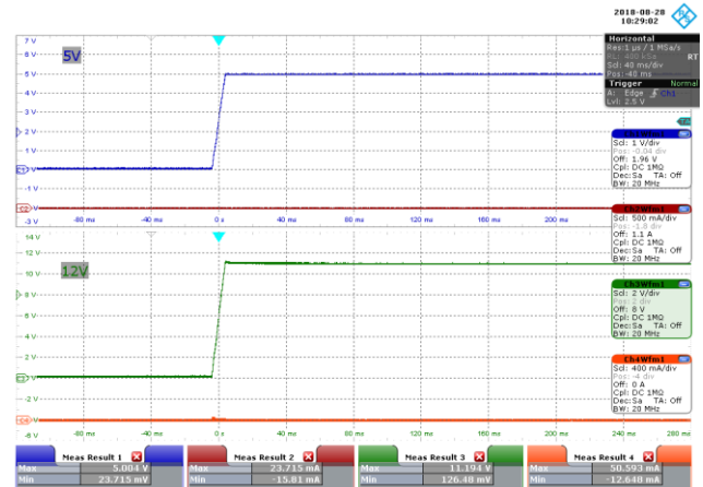
Figure 40 – 115 VAC 60 Hz, No-Load Start-up.
