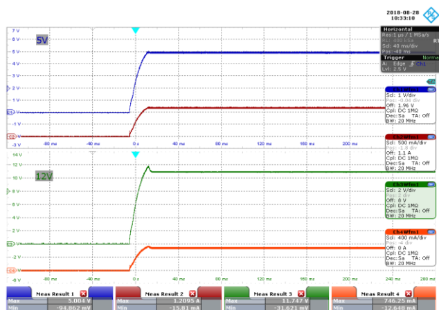
Figure 43 – 85 VAC 60 Hz, Full Load Start-up.
