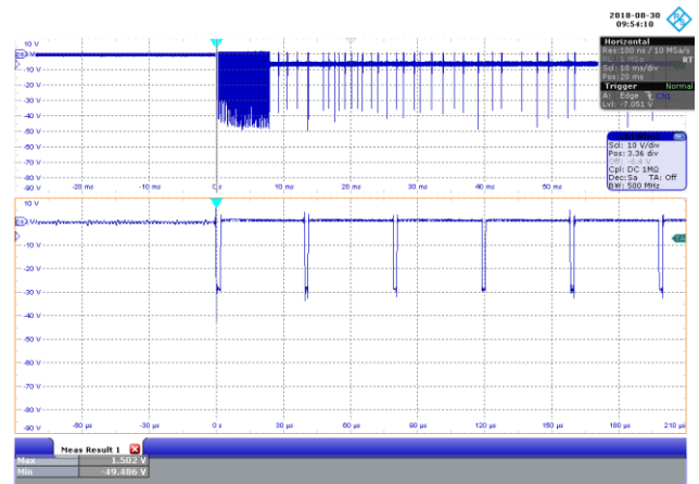
Figure 98 – 277 VAC 50 Hz, Full Load.
