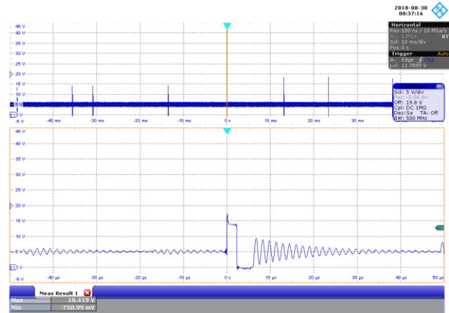
Figure 72 – 115 VAC 60 Hz, No-Load.
