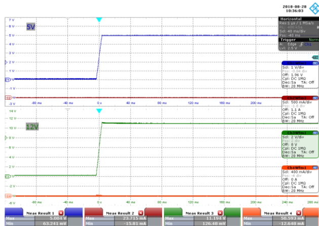
Figure 49 – 230 VAC 50 Hz, No-Load Start-up.
