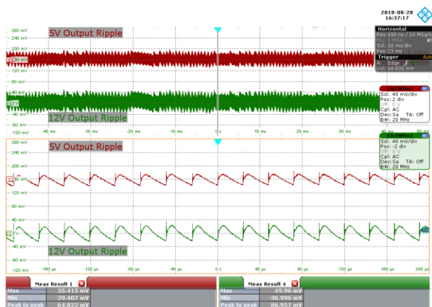
Figure 118 – 85 VAC 60 Hz, 50% Load.
