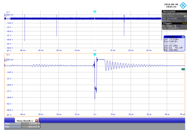
Figure 90 – 277 VAC 50 Hz, No-Load.
