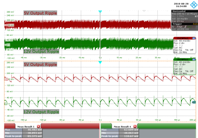
Figure 115 – 115 VAC 60 Hz, 75% Load.
