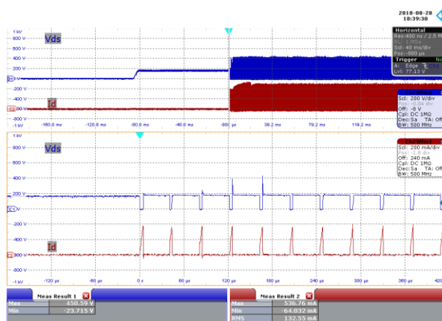
Figure 60 – 115 VAC 60 Hz, Full Load Start-up. CH1: V_{DS} , 200 V / div., 40 ms / div. CH2: I_{DS} , 200 mA / div., 40 ms / div. Zoom: 60 \mu s / div. V_{DS(MAX)} = 450.59 V, I_{DS(MAX)} = 536.76 mA.
