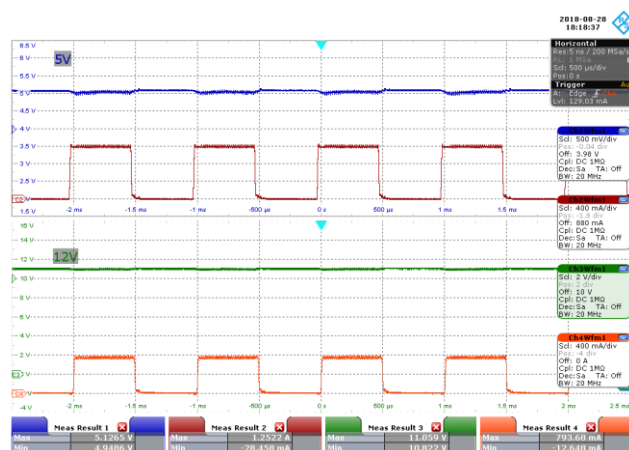
Figure 22 – 277 VAC 50 Hz.
