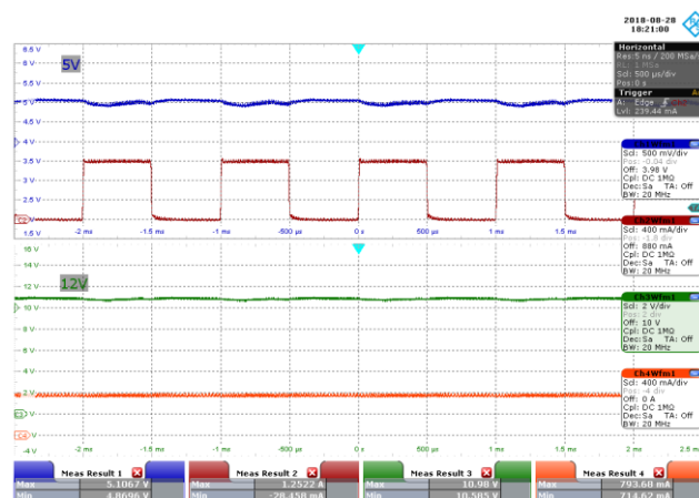
Figure 28 – 115 VAC 60 Hz.
