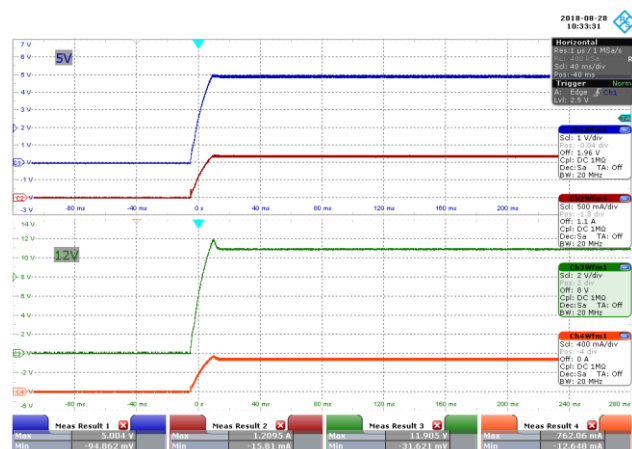
Figure 44 – 115 VAC 60 Hz, Full Load Start-up.
