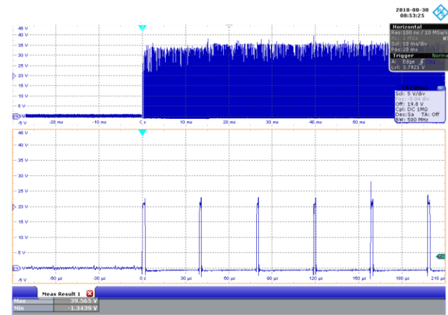
Figure 78 – 277 VAC 50 Hz, Full Load.
