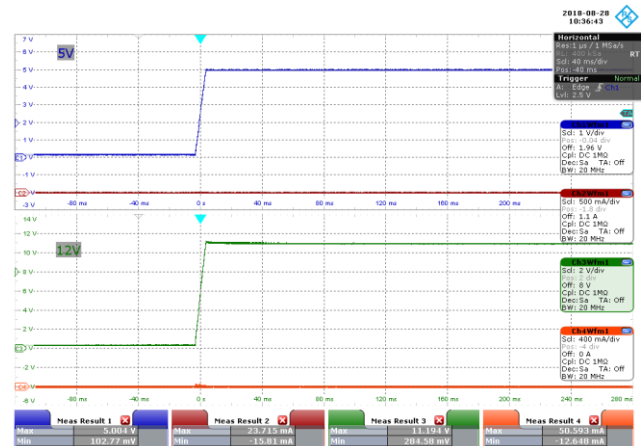
Figure 50 – 277 VAC 50 Hz, No-Load Start-up.
