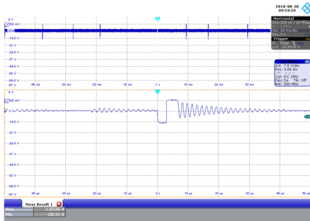
Figure 87 – 85 VAC 60 Hz, No-Load.
