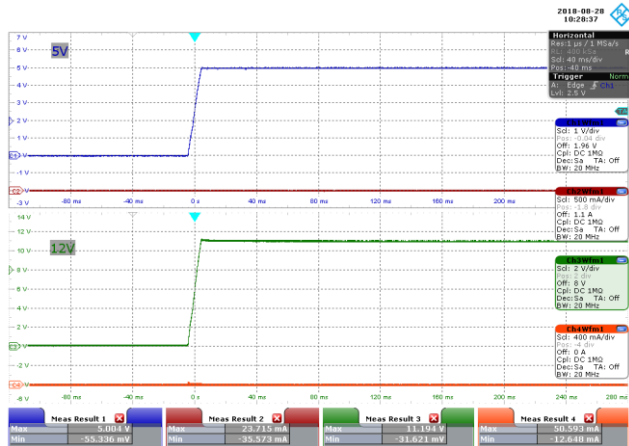
Figure 39 – 85 VAC 60 Hz, No-Load Start-up.
