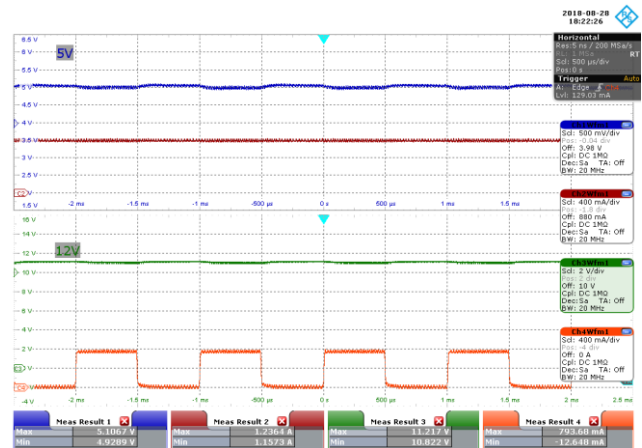
Figure 32 – 115 VAC 60 Hz.
