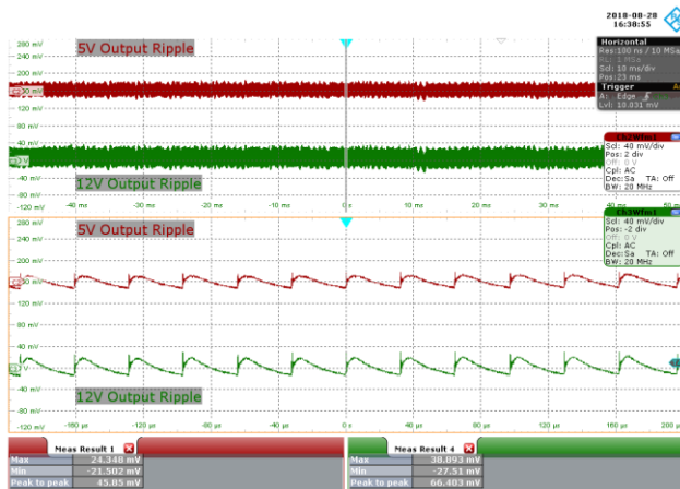
Figure 122 – 85 VAC 60 Hz, 25% Load.
