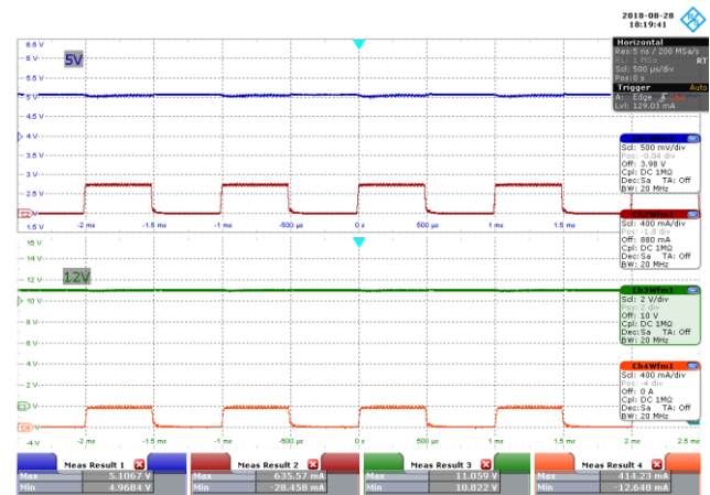
Figure 24 – 115 VAC 60 Hz.
