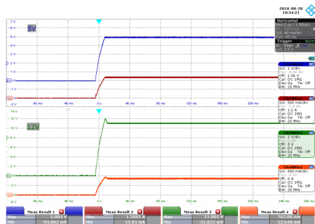
Figure 46 – 277 VAC 50 Hz, Full Load Start-up.
