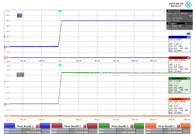
Figure 48 – 115 VAC 60 Hz, No-Load Start-up.
