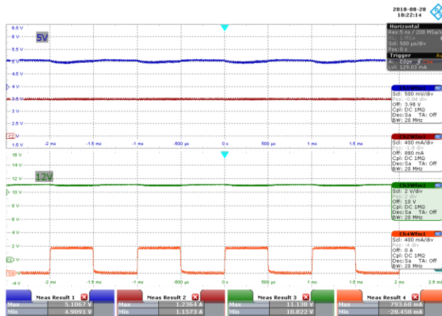
Figure 31 – 85 VAC 60 Hz.
