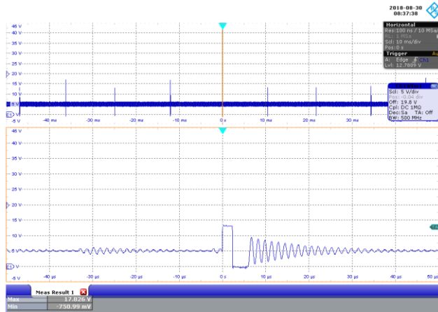
Figure 71 – 85 VAC 60 Hz, No-Load.
