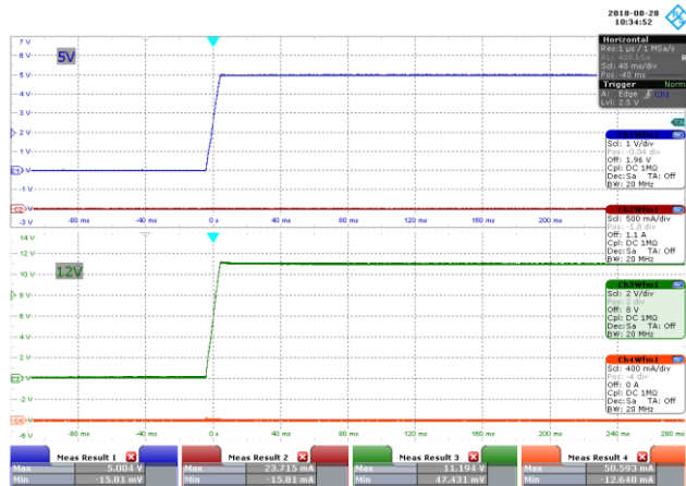
Figure 47 – 85 VAC 60 Hz, No-Load Start-up.
