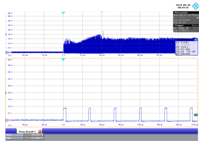
Figure 76 – 115 VAC 60 Hz, Full Load.
