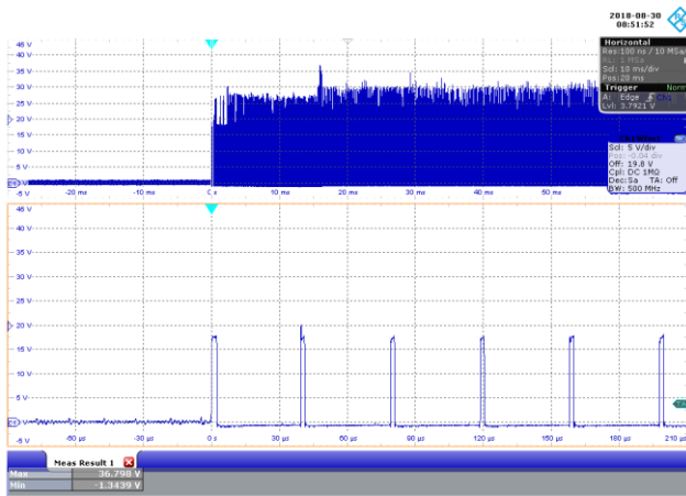
Figure 77 – 230 VAC 50 Hz, Full Load.
