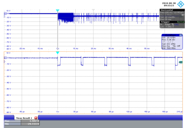
Figure 96 – 115 VAC 60 Hz, Full Load.
