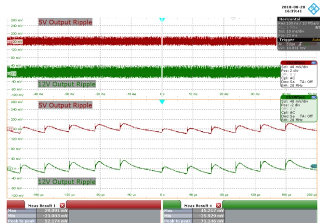
Figure 125 – 277 VAC 50 Hz, 25% Load.
