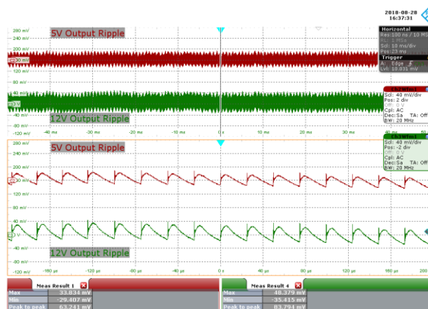
Figure 119 – 115 VAC 60 Hz, 50% Load.
