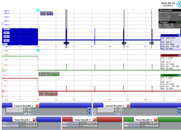
Figure 101 – 85 VAC, Short-Circuit during Normal Running Operation.
