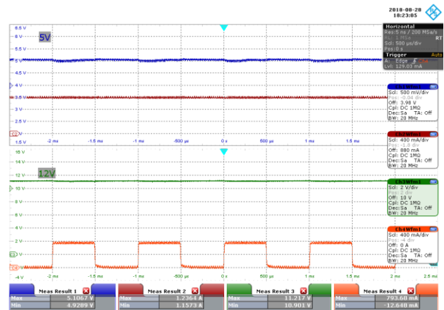
Figure 34 – 277 VAC 50 Hz.
