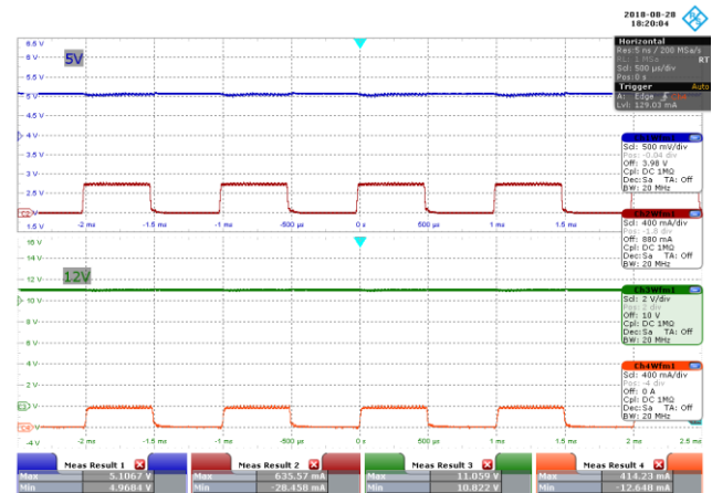
Figure 26 – 277 VAC 50 Hz.
