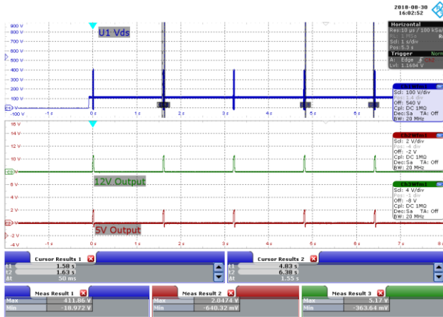
Figure 103 – 85 VAC, Short-Circuit during Start-up.
