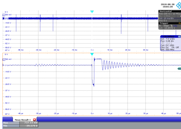
Figure 89 – 230 VAC 50 Hz, No-Load.
