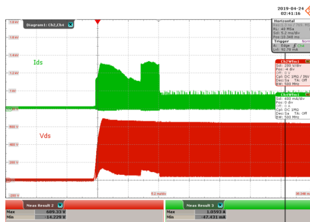
Figure 17 – Drain Voltage and Current Waveforms. 440 VAC, 120 mA Output. Upper: I_{DRAIN} , 400 mA / div. Lower: V_{DRAIN} , 200 V, 5.2 ms / div. I_{MAX} = 1.0593 A, V_{MAX} = 689.3 V
