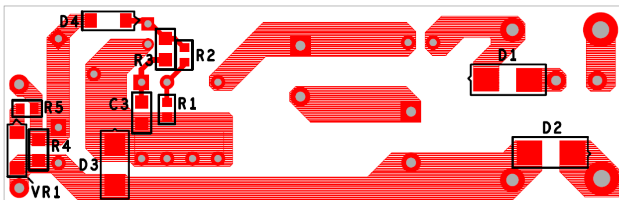
Figure 5 – Printed Circuit Layout, Bottom.
