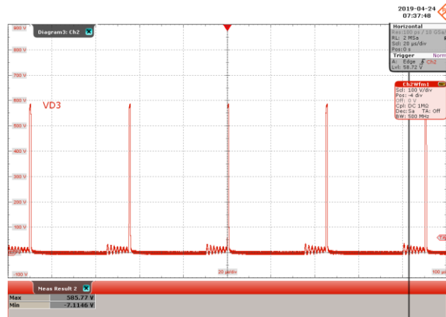
Figure 21 – Freewheeling Diode Voltage Waveforms. 440 VAC, 120 mA Output. 100 V, 20 \mu s / div. V_{MAX} : 585.77 V.
