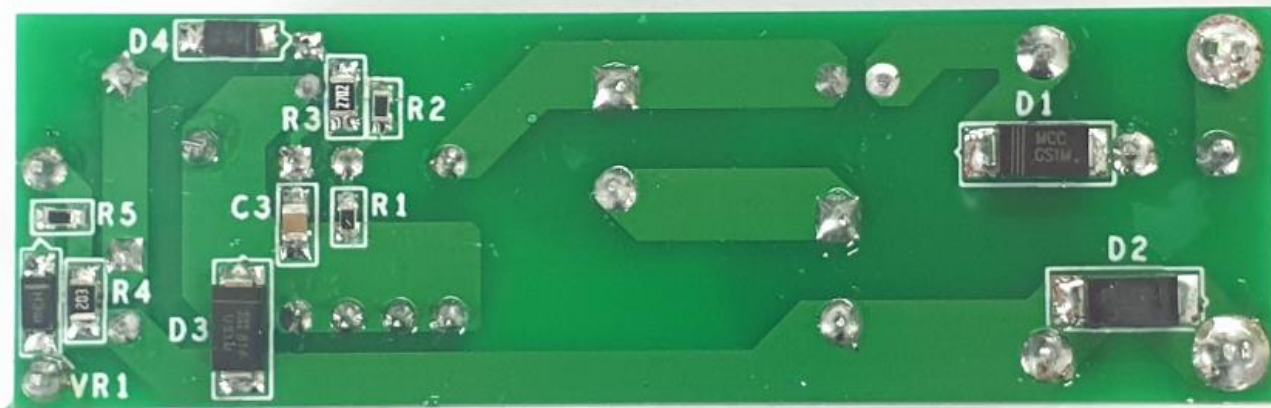
Figure 2 – Populated Circuit Board Photograph, Bottom.
