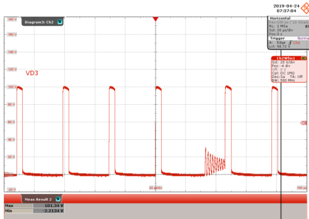
Figure 20 – Freewheeling Diode Voltage Waveforms. 85 VAC, 120 mA Output. 20 V, 20 \mu s / div. V_{MAX} : 101.34 V.
