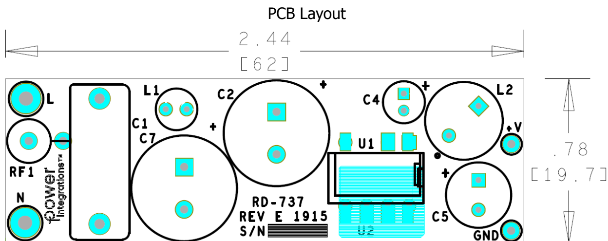
Figure 4 – Printed Circuit Layout, Top (2.44" [62 mm] L x .78" [19.7 mm] W).
