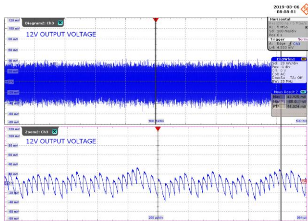
Figure 33 – Output Voltage Ripple Waveforms. 265 VAC, 120 mA Output. 20 mV, 100 ms / div.; 200 \mu s / div. V_{PK-PK} : 98.024 mV.
