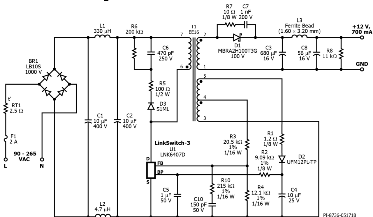
Figure 3 – Schematic Diagram.
