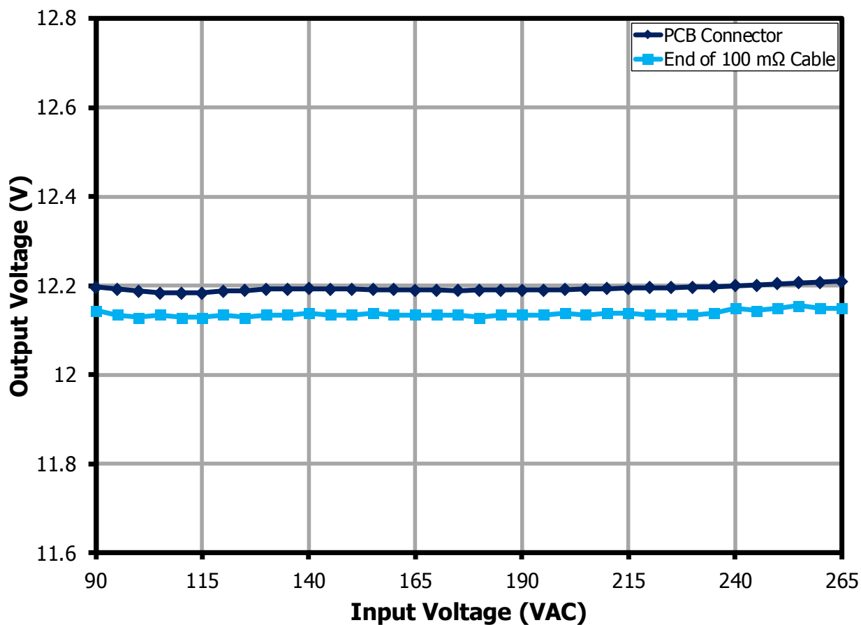
Figure 19 – Line Regulation.
