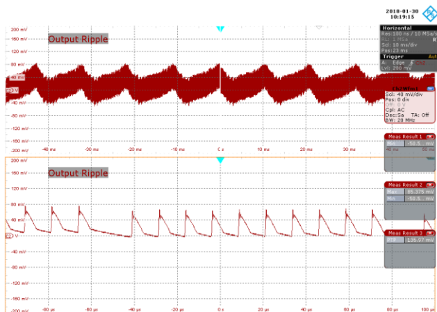
Figure 100 – 90 VAC 47 Hz, 100% Load. CH1: V_{OUT} , 40 mV / div., 10 ms / div. Zoom: 20 μs / div. Voltage Ripple ( V_{OUT(PK-PK)} ) = 135.9 mV).
