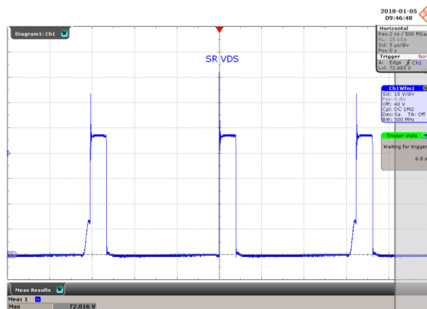
Figure 55 – SR FET Voltage Waveform. 265 VAC, 5.1 V, 6.0 A Load, (72.01 V MAX ). V DRAIN , 10 V, 5 \mu s / div.
