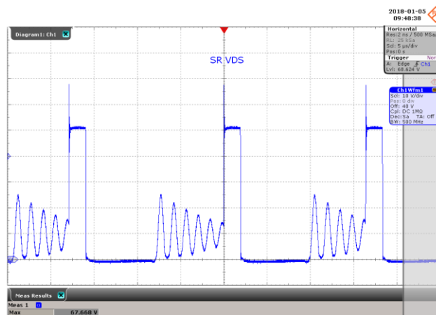
Figure 57 – SR FET Voltage Waveform. 265 VAC, 9.0 V, 3.3 A Load, (67.67 V MAX ). V DRAIN , 10 V, 5 \mu s / div.
