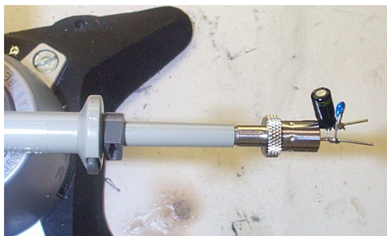
Figure 67 – Oscilloscope Probe with Probe Master ( www.probemaster.com ) 4987A BNC Adapter. (Modified with wires for ripple measurement, and two parallel decoupling capacitors added)
