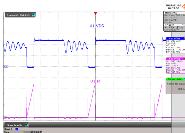
Figure 45 – Drain Voltage and Current Waveforms. 265 VAC, 9.0 V, 3.3 A Load, (530 V MAX ). Upper: V DRAIN , 200 V, 5 \mu s / div. Lower: I DRAIN , 0.5 A / div.
