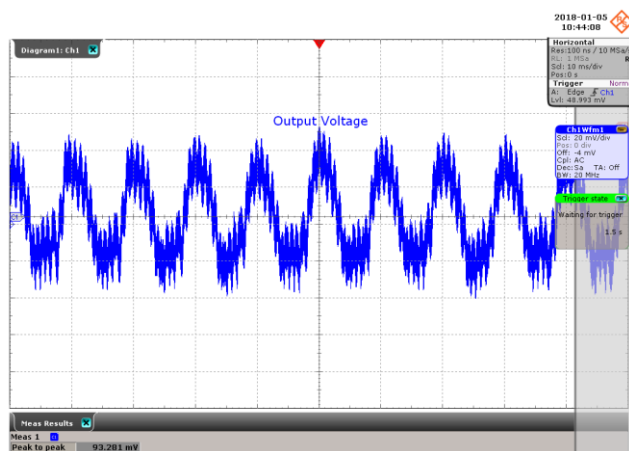
Figure 74 – Output Ripple. 180 VAC Input, 15.0 V, 2.0 A Load. V_{OUT} , 20 mV / div., 10 ms / div.
