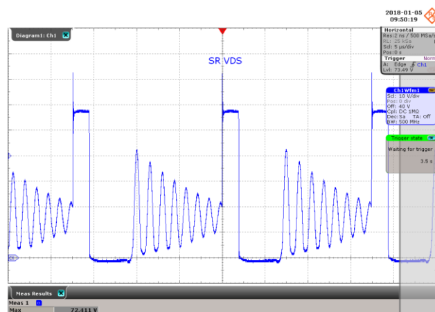
Figure 59 – SR FET Voltage Waveform. 265 VAC, 15.0 V, 2.0 A Load, (72.4 V MAX ). V DRAIN , 10 V, 5 \mu s / div.
