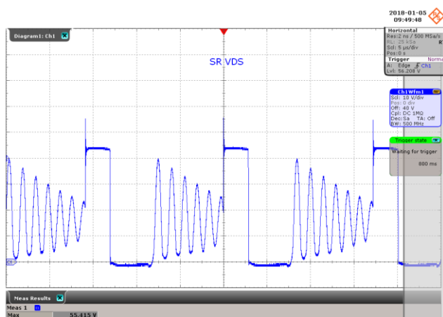
Figure 58 – SR FET Voltage Waveform. 180 VAC, 15.0 V, 2.0 A Load, (55.4 V MAX ). V DRAIN , 10 V, 5 \mu s / div.
