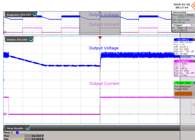
Figure 41 – Transient Response. 265 VAC, 15.3 V, 0 – 2 A Load Step. V_{\text{MIN}} : 15.36 V, V_{\text{MAX}} : 16.23 V. Upper: V_{\text{OUT}} , 0.4V / div., 100 ms / div. Lower: I_{\text{LOAD}} , 1 A / div.
