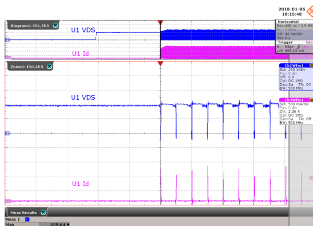
Figure 51 – Drain Voltage and Current Waveforms. 265 VAC, 9.0 V, 3.3 A Load, (530 V MAX ). Upper: V_{DRAIN} , 200 V, 40 ms / div. Lower: I_{DRAIN} , 0.5 A / div.
