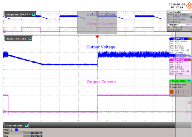
Figure 40 – Transient Response. 180 VAC, 15.3 V, 0 – 2 A Load Step. V_{\text{MIN}} : 15.39 V, V_{\text{MAX}} : 16.20 V. Upper: V_{\text{OUT}} , 0.4 V / div., 100 ms / div. Lower: I_{\text{LOAD}} , 1 A / div.
