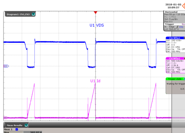
Figure 43 – Drain Voltage and Current Waveforms. 265 VAC, 5.1 V, 6.0 A Load, (506 V MAX ). Upper: V DRAIN , 200 V, 5 \mu s / div. Lower: I DRAIN , 0.5 A / div.
