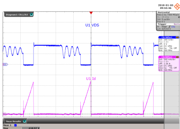
Figure 44 – Drain Voltage and Current Waveforms. 180 VAC, 9.0 V, 3.3 A Load, (419 V MAX ). Upper: V DRAIN , 200 V, 5 \mu s / div. Lower: I DRAIN , 0.5 A / div.
