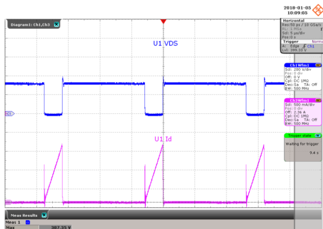
Figure 42 – Drain Voltage and Current Waveforms. 180 VAC, 5.1 V, 6.0 A Load, (387 V MAX ). Upper: V DRAIN , 200 V, 5 \mu s / div. Lower: I DRAIN , 0.5 A / div.
