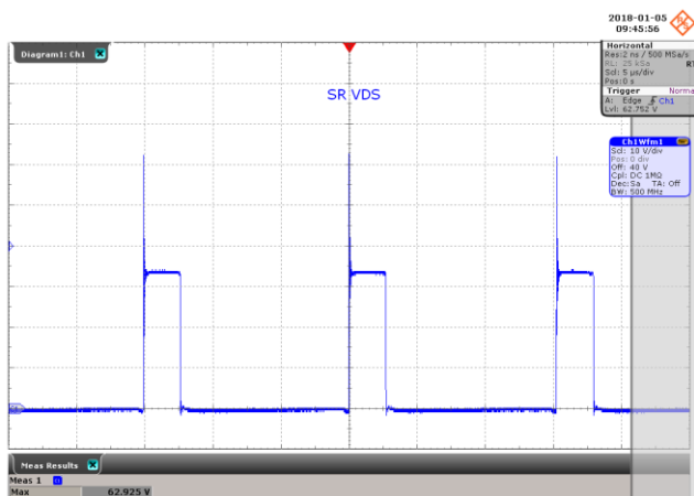
Figure 54 – SR FET Voltage Waveform. 180 VAC, 5.1 V, 6.0 A Load, (62.93 V MAX ). V DRAIN , 10 V, 5 \mu s / div.
