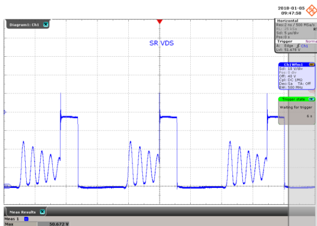
Figure 56 – SR FET Voltage Waveform. 180 VAC, 9.0 V, 3.3 A Load, (50.67 V MAX ). V DRAIN , 10 V, 5 \mu s / div.
