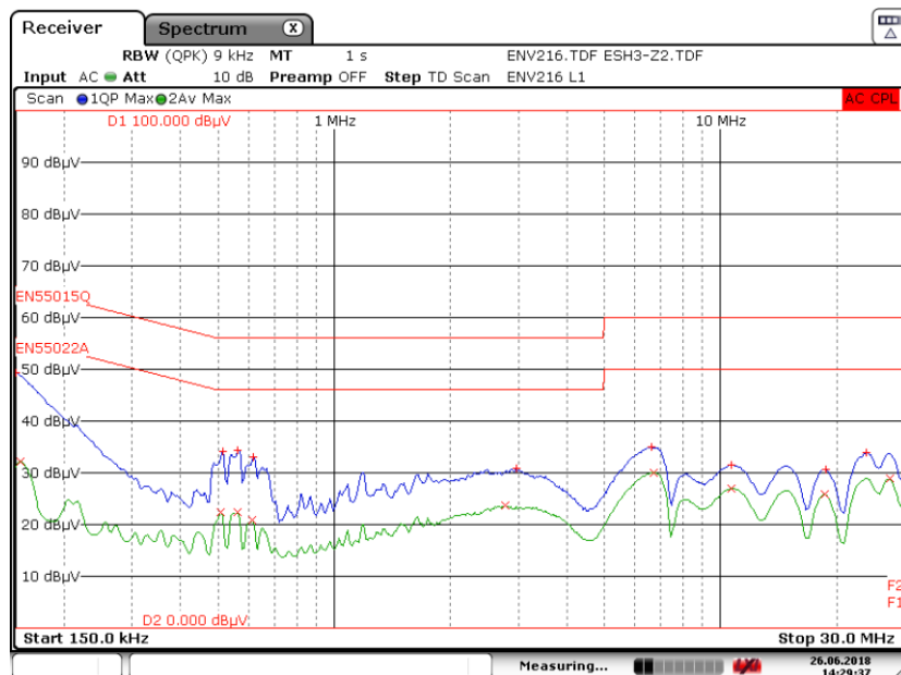
Figure 121 – Earth Ground EMI, 20 V / 2 A Load 115 VAC, 60 Hz, and EN55022 B Limits (Line).
