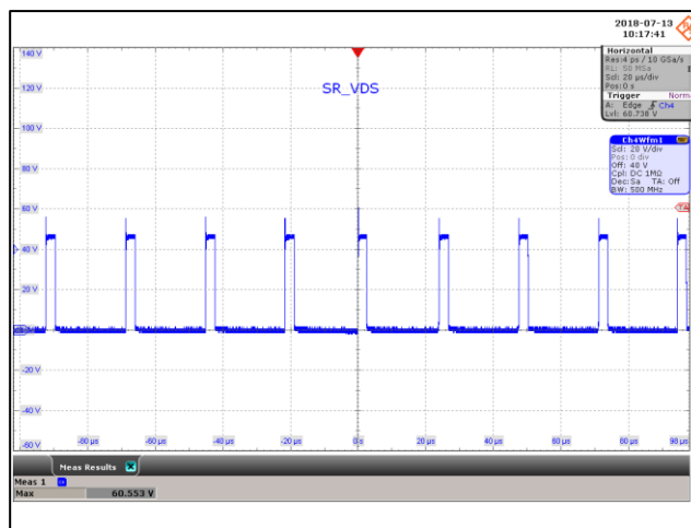
Figure 80 – SR FET Voltage Waveforms. 265 VAC, 5.0 V, 5 A Load (60.55 V MAX ). SR_V DRAIN , 20 V / div., 20 μs / div.
