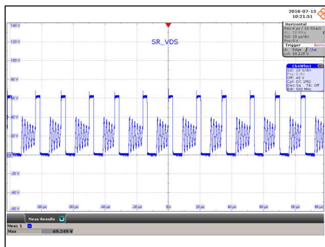
Figure 86 – SR FET Voltage Waveforms. 265 VAC, 20.0 V, 2 A Load (69.24 V MAX ). SR_V DRAIN , 20 V / div., 20 μs / div.
