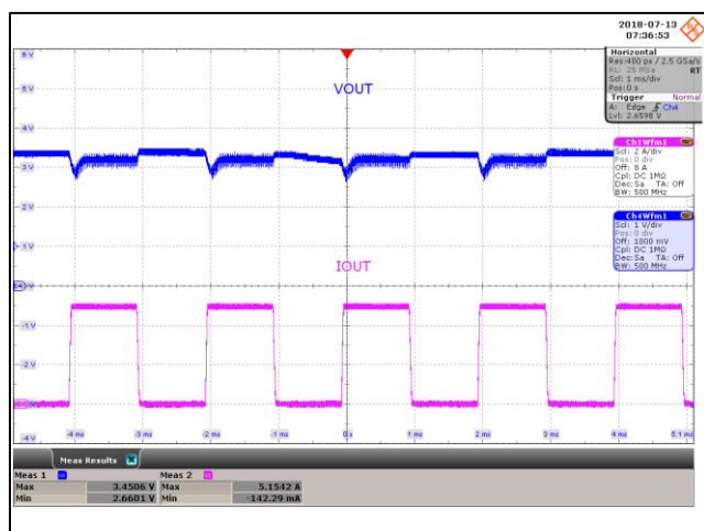
Figure 55 – Transient Response. 85 VAC, 3.0 V, 0 - 5 A Load Step. V_{\text{MIN}} : 2.66 V, V_{\text{MAX}} : 3.45 V. Upper: V OUT , 1 V / div., 1 ms / div. Lower: I LOAD , 2 A / div.
