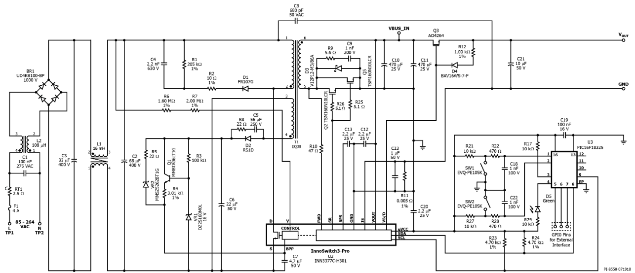
Figure 3 – Schematic.
