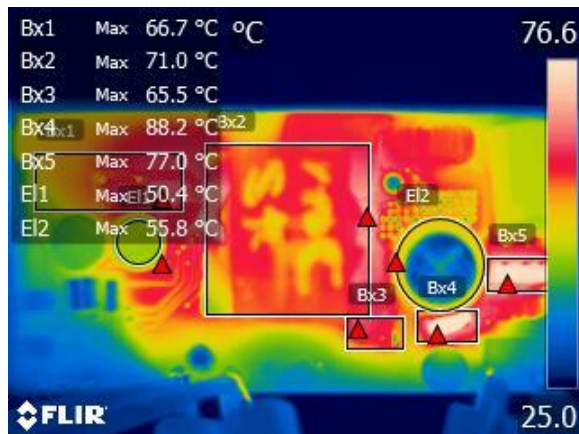
Figure 43 – Top Components, Ambient = 27 °C.
