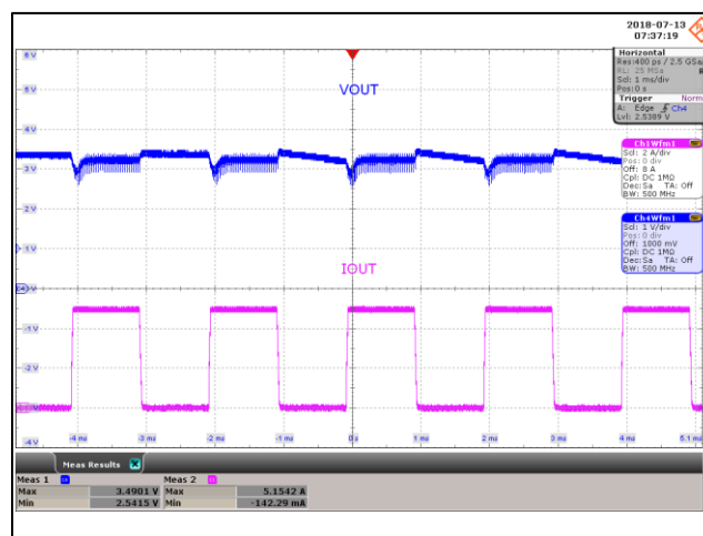
Figure 56 – Transient Response. 265 VAC, 3.0 V, 0 - 5 A Load Step. V_{\text{MIN}} : 2.54 V, V_{\text{MAX}} : 3.49 V. Upper: V OUT , 1 V / div., 1 ms / div. Lower: I LOAD , 2 A / div.
