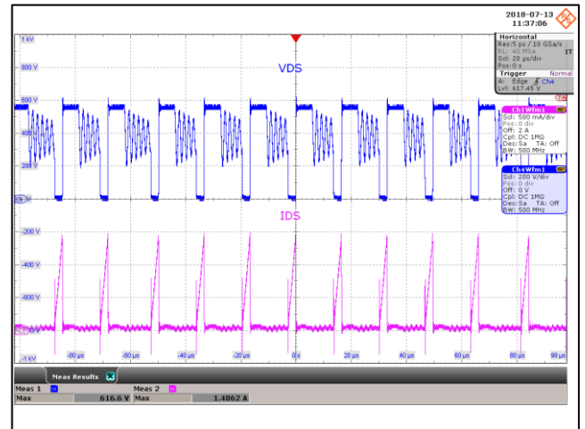
Figure 74 – Drain Voltage and Current Waveforms. 265 VAC, 20.0 V, 2.0 A Load (616 V MAX ). Upper: V DRAIN , 200 V / div., 20 µs / div. Lower: I DRAIN , 500 mA / div.
