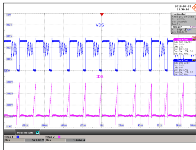
Figure 72 – Drain Voltage and Current Waveforms. 265 VAC, 15.0 V, 2.66 A Load (577 V MAX ). Upper: V DRAIN , 200 V / div., 20 μs / div. Lower: I DRAIN , 500 mA / div.
