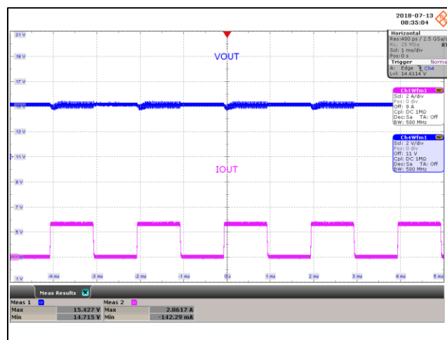
Figure 62 – Transient Response. 265 VAC, 15.0 V, 0 - 2.66 A Load Step. V_{MIN} : 14.71 V, V_{MAX} : 15.42 V. Upper: V_{OUT} , 2 V / div., 1 ms / div. Lower: I_{LOAD} , 2 A / div.
