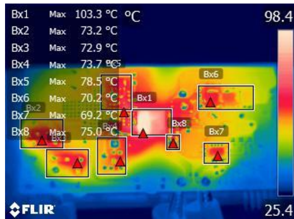
Figure 44 – Bottom Components, Ambient = 27 °C.
