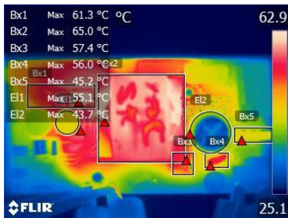
Figure 45 – Top Components, Ambient = 27 °C.
