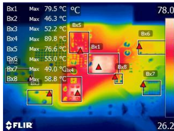
Figure 54 – Bottom Components, Ambient = 27 °C.
