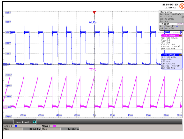
Figure 73 – Drain Voltage and Current Waveforms. 85 VAC, 20.0 V, 2.0 A Load (363 V MAX ). Upper: V DRAIN , 100 V / div., 20 µs / div. Lower: I DRAIN , 500 mA / div.
