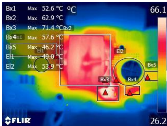
Figure 53 – Top Components, Ambient = 27 °C.
