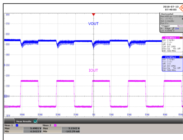
Figure 58 – Transient Response. 265 VAC, 5.0 V, 0 - 5 A Load Step. V_{\text{MIN}} : 4.54 V, V_{\text{MAX}} : 5.49 V. Upper: V OUT , 1 V / div., 1 ms / div. Lower: I LOAD , 2 A / div.
