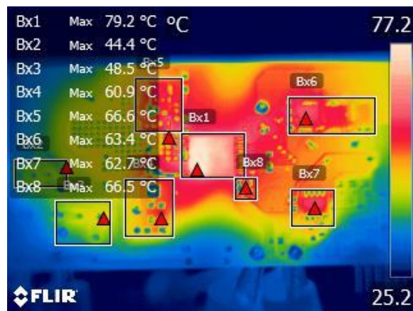
Figure 46 – Bottom Components, Ambient = 27 °C.
