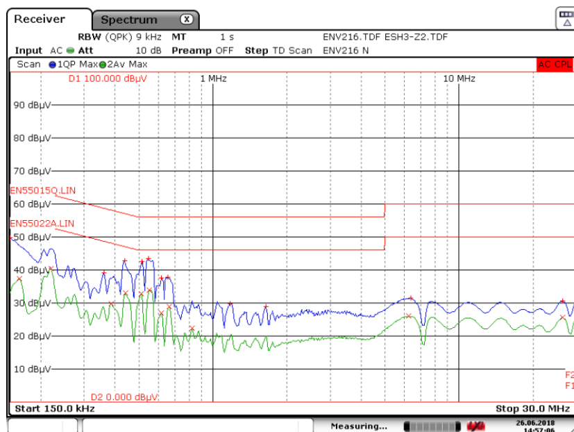
Figure 122 – Earth Ground EMI, 20 V / 2 A Load 115 VAC, 60 Hz, and EN55022 B Limits (Neutral).
