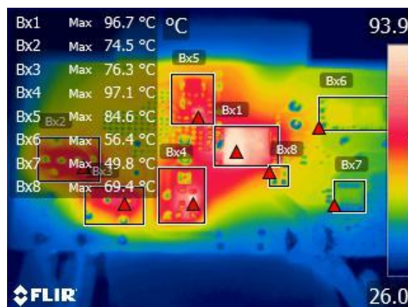
Figure 52 – Bottom Components, Ambient = 27 °C.
