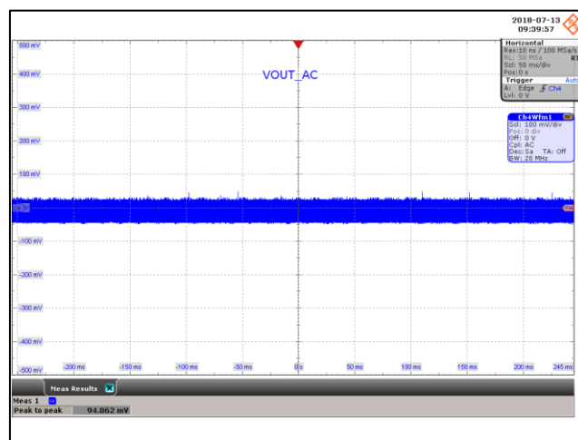
Figure 94 – Output Ripple.(PK-PK – 94 mV) 265 VAC Input 5.0 V, 5 A Load. V_{OUT} , 100 mV / div., 50 ms / div.
