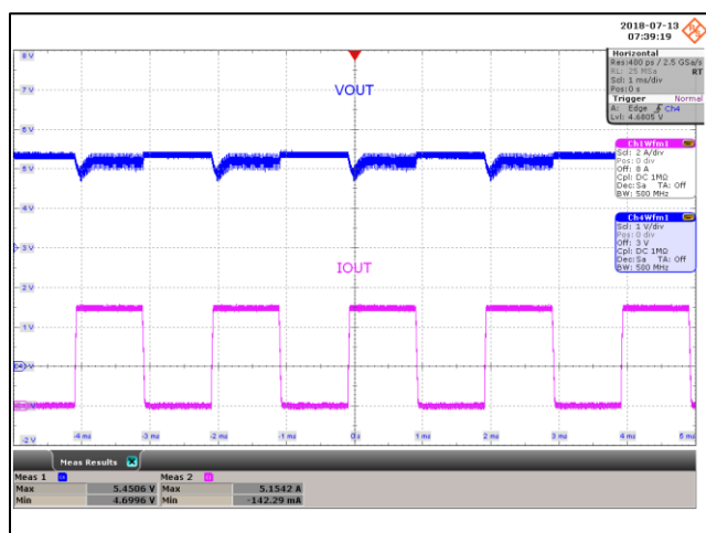
Figure 57 – Transient Response. 85 VAC, 5.0 V, 0 - 5 A Load Step. V_{\text{MIN}} : 4.69 V, V_{\text{MAX}} : 5.45 V. Upper: V OUT , 1 V / div., 1 ms / div. Lower: I LOAD , 2 A / div.
