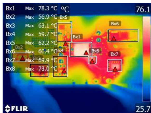
Figure 40 – Bottom Components, Ambient = 27 °C.
