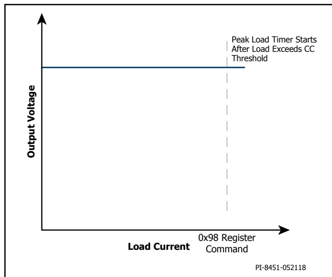
Figure 16. Constant Voltage Only (CVO) Mode.
