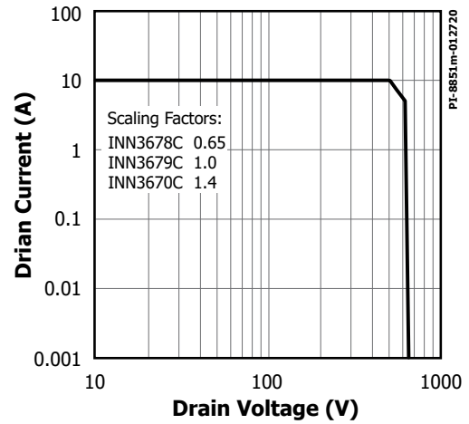
Figure 38. Maximum Allowable Drain Current vs. Drain Voltage (PowiGaN Devices INN3678C / INN3679C / INN3670C).
