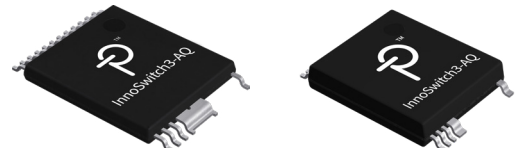
Figure 2. Safety-Compliant InSOP-24D and InSOP-T28G Packages Provide Extended Creepage and Clearance.
