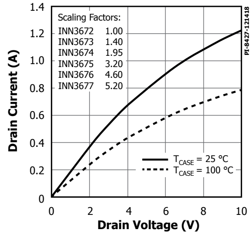
Figure 25. Output Characteristics.
