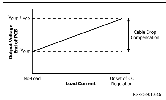
Figure 7. Cable Drop Compensation Characteristics.
