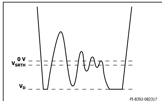
Figure 16. Unacceptable FORWARD Pin Waveform After Handshake With SR MOSFET Conduction During Flyback Cycle.
