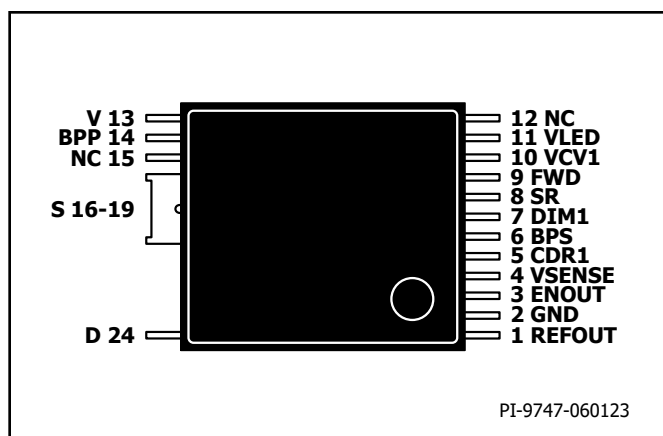
Figure 6. InnoMux2-BL InSOP-24D 1CV+4LED Single Dimming with SR Pin Configuration.
