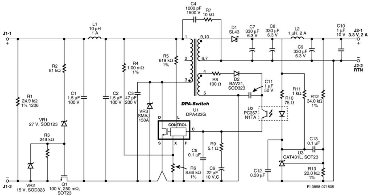
Figure 2 - EP68 Schematic.
