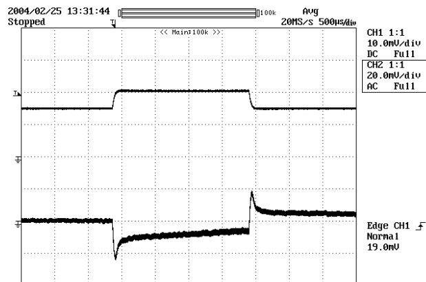
Figure 18 - Transient Response, 57 VDC, 75-100-75% Load Step. Top: Load Current, 1 A / div. Bottom: Output Voltage, 20 mV, 500 µs / div.
