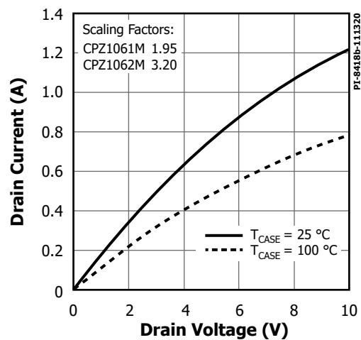
Figure 9. Output Characteristics.
