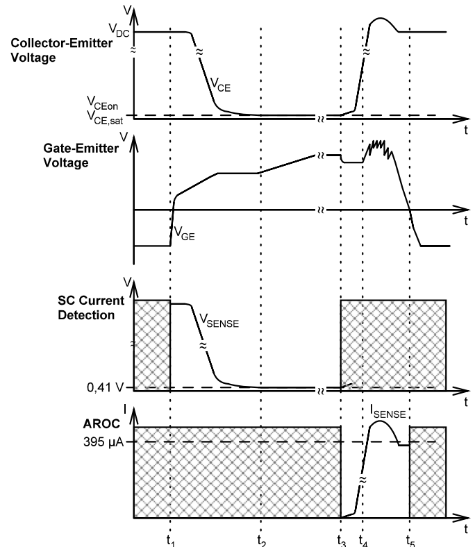
Figure 17. AROC and Short-Circuit Detection on SENSE Potential.
