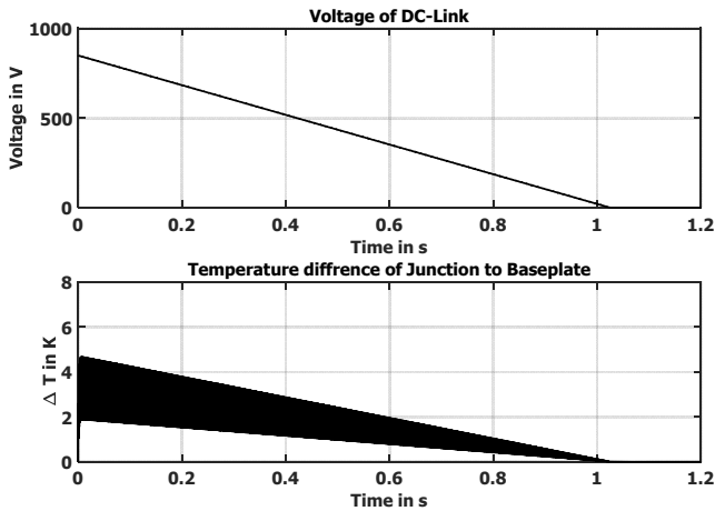
Figure 10. Thermal Simulation of active discharge using FF900R12ME7W_B11 with 1100 \mu\text{F} Cap at 850 V, 2 \mu\text{s} , 1 kHz.
