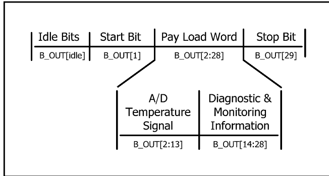
Figure 15. B_OUT Bit Assignment.
