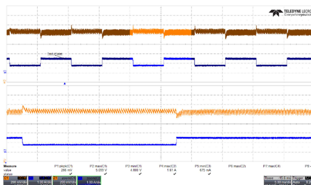
Figure 41 – Transient Response. 265 VAC, 5.0 V, 0.75 – 1.5 A Load Step. V_{MIN} : 4.800 V, V_{MAX} : 5.099 V. Upper: V_{OUT} , 0.2 V / div., 5 ms / div. Lower: I_{LOAD} , 1 A / div. Zoom: 1 ms / div.
