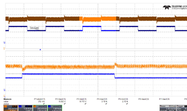
Figure 53 – Transient Response. 265 VAC, 9.0 V, 2.25 – 3 A Load Step. V_{MIN} : 8.773 V, V_{MAX} : 9.092 V. Upper: V_{OUT} , 0.2 V / div., 5 ms / div. Lower: I_{LOAD} , 1 A / div. Zoom: 1 ms / div.
