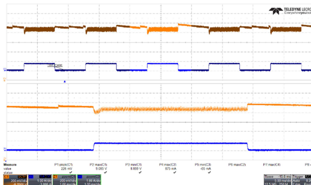
Figure 47 – Transient Response. 265 VAC, 9.0 V, 0 – 0.75 A Load Step. V_{MIN} : 8.859 V, V_{MAX} : 9.085 V. Upper: V_{OUT} , 0.2 V / div., 5 ms / div. Lower: I_{LOAD} , 1 A / div. Zoom: 1 ms / div.
