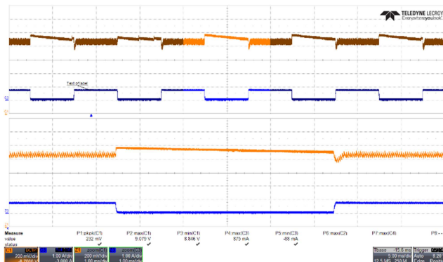
Figure 46 – Transient Response. 90 VAC, 9.0 V, 0 – 0.75 A Load Step. V_{MIN} : 8.846 V, V_{MAX} : 9.079 V. Upper: V_{OUT} , 0.2 V / div., 5 ms / div. Lower: I_{LOAD} , 1 A / div. Zoom: 1 ms / div.
