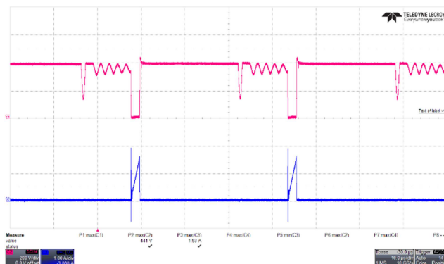
Figure 71 – Drain Voltage Waveforms. 265 VAC, 5.0 V, 3 A Load (441 V_{MAX} ). Upper: V_{DRAIN} , 200 V / div. Lower: I_{DRAIN} , 1 A / div. Time: 10 \mu s / div.
