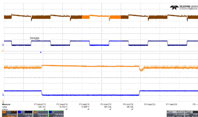
Figure 54 – Transient Response.
