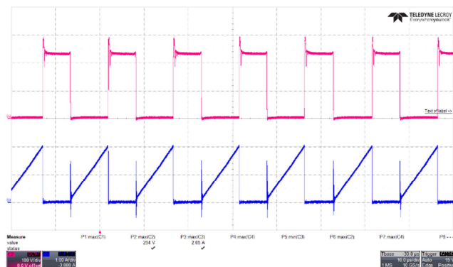
Figure 76 – Drain Voltage Waveforms. 90 VAC, 20 V, 3 A Load (294 V_{MAX} ). Upper: V_{DRAIN} , 100 V / div. Lower: I_{DRAIN} , 1 A / div. Time: 10 \mu s / div.
