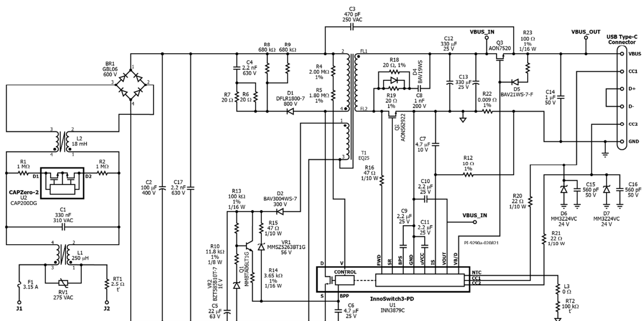
Figure 4 – Schematic.
