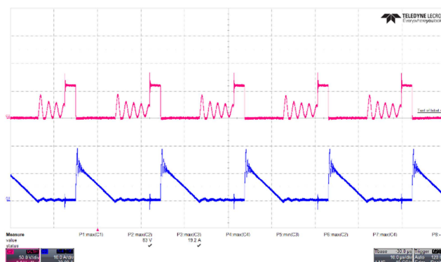
Figure 83 – SR FET Voltage Waveforms. 265 VAC, 15.0 V, 3 A Load (83 V_{MAX} ). Upper: V_{DRAIN} , 50 V / div. Lower: I_{DRAIN} , 10 A / div. Time: 10 \mu s / div.
