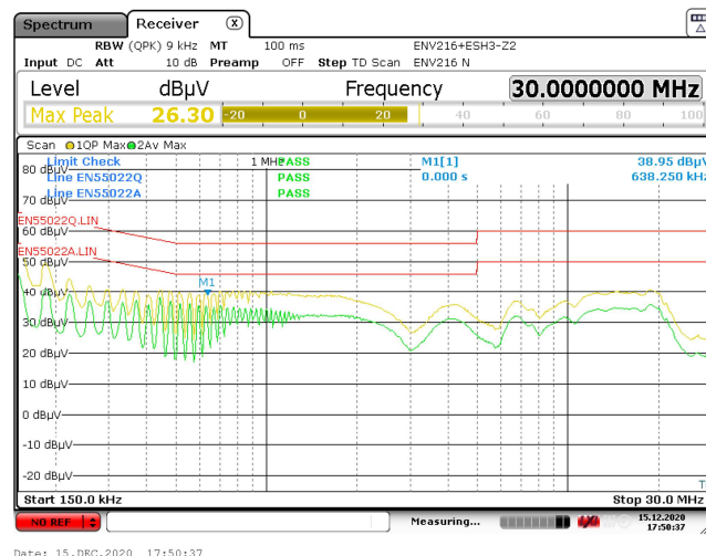
Figure 125 – Earth Grounded EMI, 9 V / 3 A Load.
