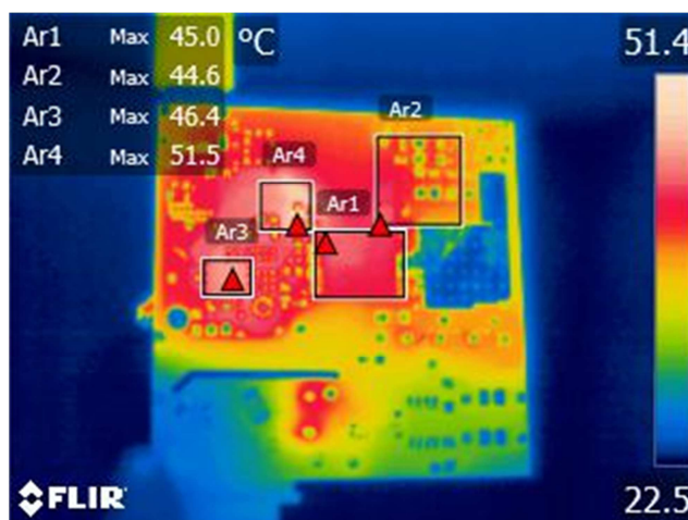
Figure 23 – Bottom Thermal Image.
