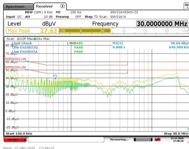
Figure 121 – Earth Floating EMI, 9 V / 3 A Load.
