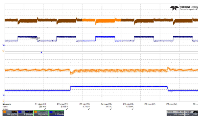
Figure 40 – Transient Response. 90 VAC, 5.0 V, 0.75 – 1.5 A Load Step. V_{MIN} : 4.786 V, V_{MAX} : 5.085 V. Upper: V_{OUT} , 0.2 V / div., 5 ms / div. Lower: I_{LOAD} , 1 A / div. Zoom: 1 ms / div.
