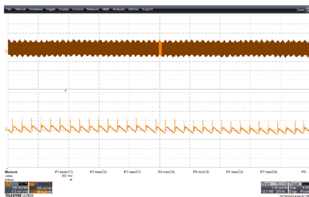
Figure 111 – Output Ripple. PK-PK = 193 mV. 265 VAC IN 20 V, 3 A Load. V OUT , 100 mV / div., 5 ms / div. Zoom: 50 μs / div.
