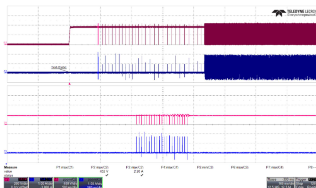
Figure 89 – Drain Voltage Waveforms. 265 VAC, 5.0 V, 3 A Load (452 V_{MAX} ). Upper: V_{DRAIN} , 200 V / div. Lower: I_{DRAIN} , 1 A / div. Time: 100 ms / div. (Zoom: 500 \mu s / div.)
