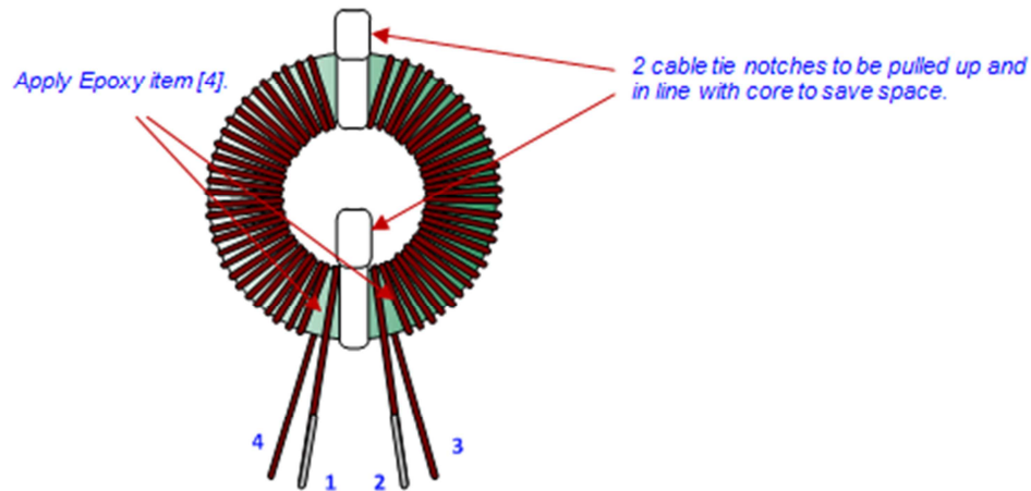
Figure 11 – 18 mH CMC Illustration Image.
