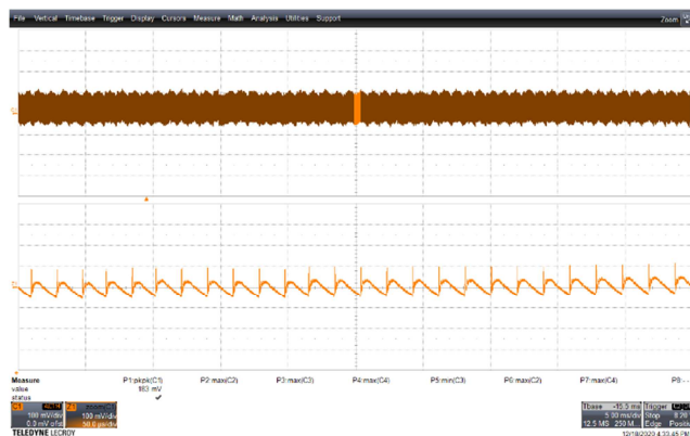
Figure 107 – Output Ripple. PK-PK = 183 mV. 265 VAC IN , 15.0 V, 3 A Load. V OUT , 100 mV / div., 5 ms / div. Zoom: 50 μs / div.
