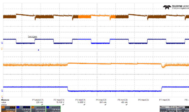
Figure 55 – Transient Response.
