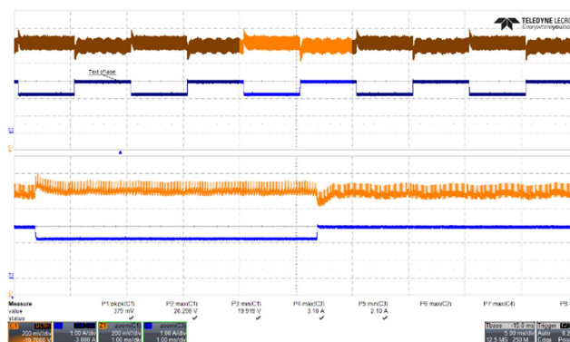
Figure 69 – Transient Response. 265 VAC, 20 V, 2.25 – 3 A Load Step. V_{MIN} : 19.919 V, V_{MAX} : 20.298 V. Upper: V_{OUT} , 0.2 V / div., 5 ms / div. Lower: I_{LOAD} , 1 A / div. Zoom: 1 ms / div.
