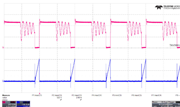
Figure 75 – Drain Voltage Waveforms. 265 VAC, 15.0 V, 3 A Load (525 V_{MAX} ). Upper: V_{DRAIN} , 200 V / div. Lower: I_{DRAIN} , 1 A / div. Time: 10 \mu s / div.
