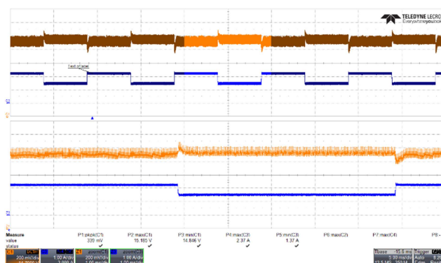
Figure 59 – Transient Response. 265 VAC, 15 V, 1.5 – 2.25 A Load Step. V_{MIN} : 14.846 V, V_{MAX} : 15.185 V. Upper: V_{OUT} , 0.2 V / div., 5 ms / div. Lower: I_{LOAD} , 1 A / div. Zoom: 1 ms / div.
