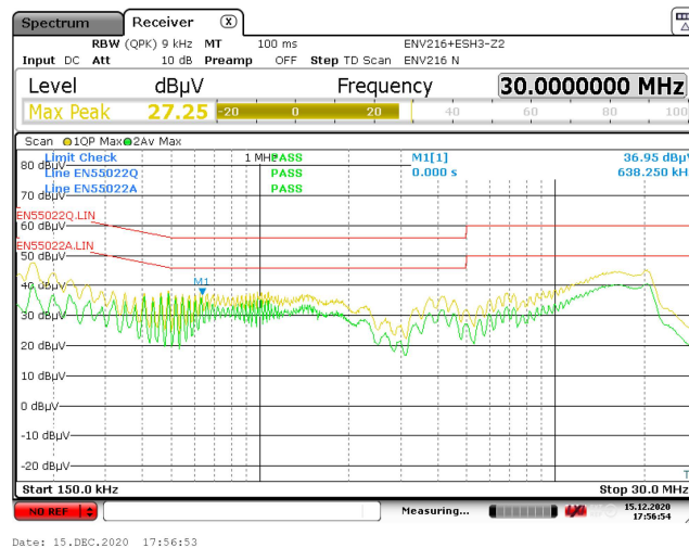
Figure 120 – Earth Floating EMI, 5 V / 3 A Load.
