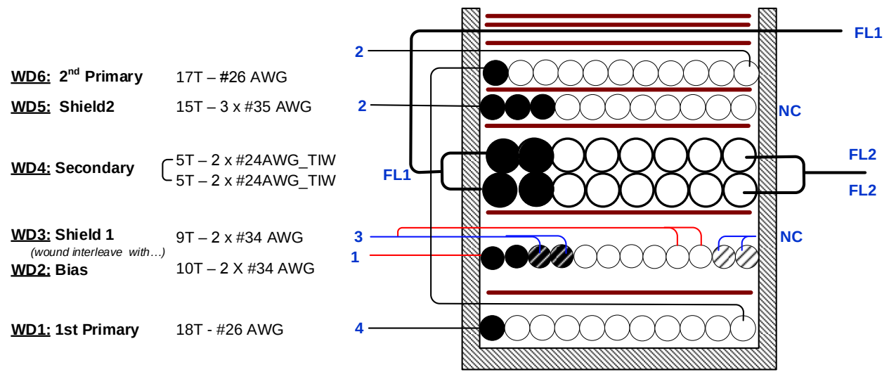
Figure 8 – Transformer Build Diagram.
