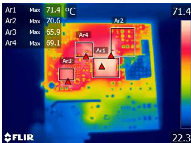
Figure 33 – Bottom Thermal Image.
