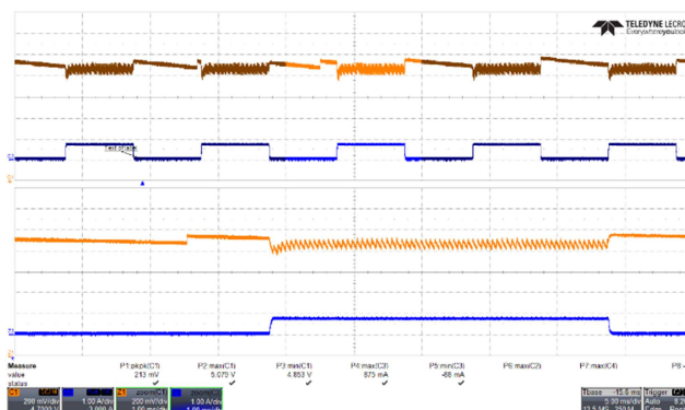
Figure 39 – Transient Response. 265 VAC, 5.0 V, 0 – 0.75 A Load Step. V_{MIN} : 4.853 V, V_{MAX} : 5.079 V. Upper: V_{OUT} , 0.2 V / div., 5 ms / div. Lower: I_{LOAD} , 1 A / div. Zoom: 1 ms / div.
