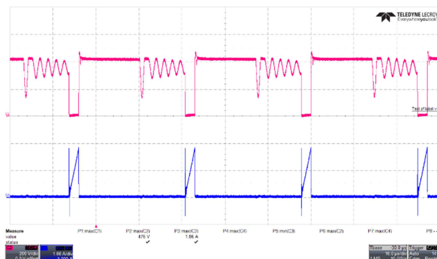
Figure 73 – Drain Voltage Waveforms. 265 VAC, 9 V, 3 A Load (476 V_{MAX} ). Upper: V_{DRAIN} , 200 V / div. Lower: I_{DRAIN} , 1 A / div. Time: 10 \mu s / div.
