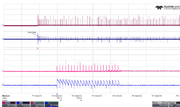
Figure 91 – SR FET Voltage Waveforms. 265 VAC, 5.0 V, 0 A Load (103 V_{MAX} ). Upper: V_{DRAIN} , 50 V / div. Lower: I_{DRAIN} , 10 A / div. Time: 100 ms / div. (Zoom: 250 \mu s / div.)
