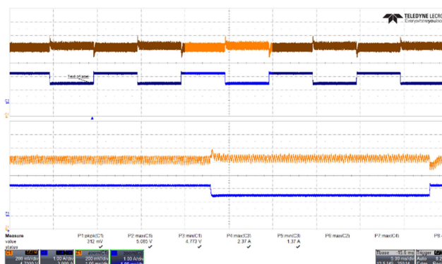
Figure 43 – Transient Response. 265 VAC, 5.0 V, 1.5 – 2.25 A Load Step. V_{MIN} : 4.773 V, V_{MAX} : 5.085 V. Upper: V_{OUT} , 0.2 V / div., 5 ms / div. Lower: I_{LOAD} , 1 A / div. Zoom: 1 ms / div.
