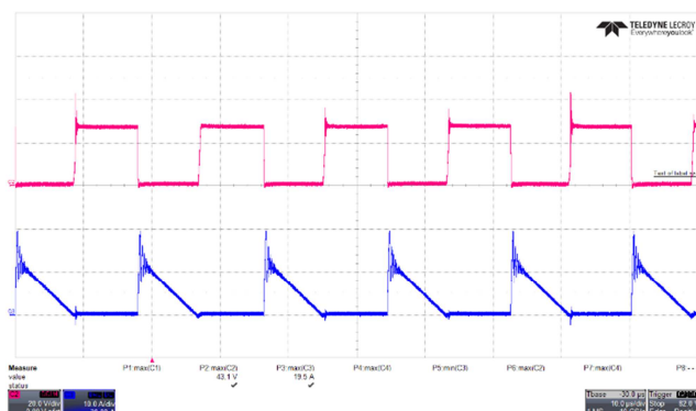
Figure 82 – SR FET Voltage Waveforms. 90 VAC, 15.0 V, 3 A Load (43.1 V_{MAX} ). Upper: V_{DRAIN} , 20 V / div. Lower: I_{DRAIN} , 10 A / div. Time: 10 \mu s / div.
