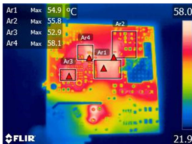
Figure 27 – Bottom Thermal Image.
