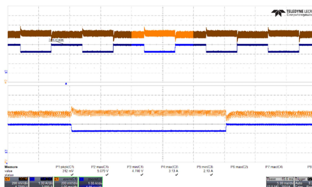
Figure 45 – Transient Response. 265 VAC, 5.0 V, 2.25 – 3 A Load Step. V_{MIN} : 4.740 V, V_{MAX} : 5.079 V. Upper: V_{OUT} , 0.2 V / div., 5 ms / div. Lower: I_{LOAD} , 1 A / div. Zoom: 1 ms / div.
