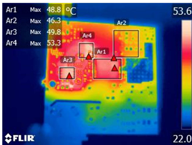
Figure 25 – Bottom Thermal Image.
