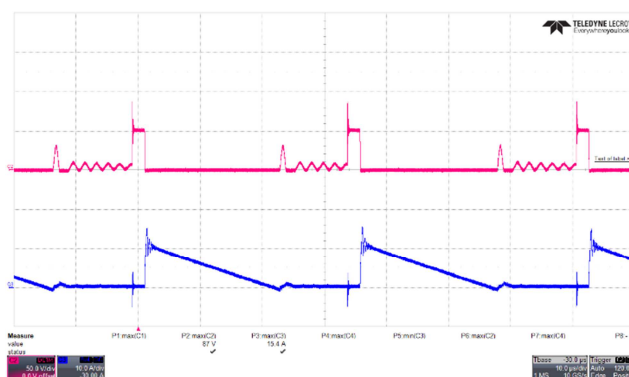
Figure 79 – SR FET Voltage Waveforms. 265 VAC, 5.0 V, 3 A Load (87 V_{MAX} ). Upper: V_{DRAIN} , 50 V / div. Lower: I_{DRAIN} , 10 A / div. Time: 10 \mu s / div.
