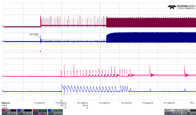
Figure 92 – SR FET Voltage Waveforms. 90 VAC, 5.0 V, 3 A Load (39.9 V_{MAX} ). Upper: V_{DRAIN} , 20 V / div. Lower: I_{DRAIN} , 10 A / div. Time: 100 ms / div. (Zoom: 250 \mu s / div.)
