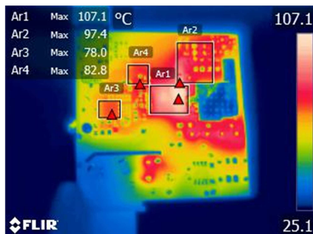
Figure 35 – Bottom Thermal Image.
