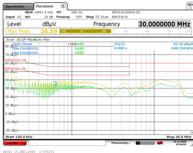
Figure 124 – Earth Grounded EMI, 5 V / 3 A Load
