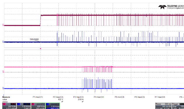
Figure 87 – Drain Voltage Waveforms. 265 VAC, 5.0 V, 0 A Load (432 V_{MAX} ). Upper: V_{DRAIN} , 200 V / div. Lower: I_{DRAIN} , 1 A / div. Time: 100 ms / div. (Zoom: 500 \mu s / div.)
