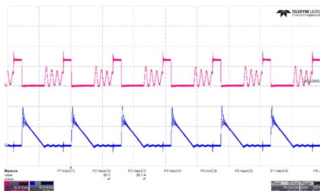
Figure 85 – SR FET Voltage Waveforms. 265 VAC, 20 V, 3 A Load (86 V_{MAX} ). Upper: V_{DRAIN} , 50 V / div. Lower: I_{DRAIN} , 10 A / div. Time: 10 \mu s / div.
