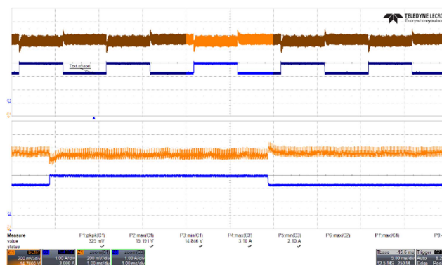
Figure 61 – Transient Response. 265 VAC, 15 V, 2.25 – 3.0 A Load Step. V_{MIN} : 14.846 V, V_{MAX} : 15.191 V. Upper: V_{OUT} , 0.2 V / div., 5 ms / div. Lower: I_{LOAD} , 1 A / div. Zoom: 1 ms / div.
