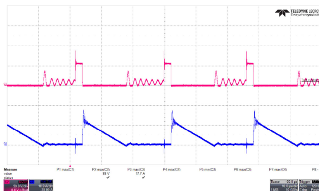
Figure 81 – SR FET Voltage Waveforms. 265 VAC, 9.0 V, 3 A Load (88 V_{MAX} ). Upper: V_{DRAIN} , 50 V / div. Lower: I_{DRAIN} , 10 A / div. Time: 10 \mu s / div.
