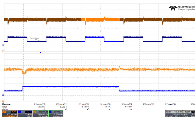
Figure 49 – Transient Response. 265 VAC, 9.0 V, 0.75 – 1.5 A Load Step. V_{MIN} : 8.793 V, V_{MAX} : 9.099 V. Upper: V_{OUT} , 0.2 V / div., 5 ms / div. Lower: I_{LOAD} , 1 A / div. Zoom: 1 ms / div.
