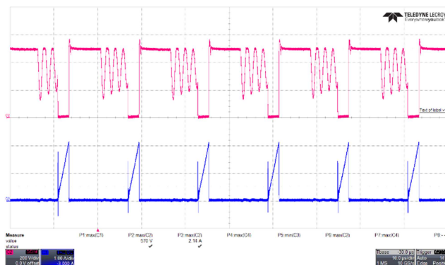
Figure 77 – Drain Voltage Waveforms. 265 VAC, 20 V, 3 A Load (570 V_{MAX} ). Upper: V_{DRAIN} , 200 V / div. Lower: I_{DRAIN} , 1 A / div. Time: 10 \mu s / div.
