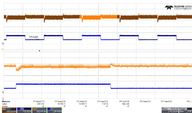
Figure 56 – Transient Response.
