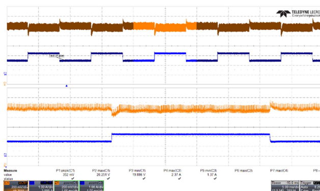
Figure 67 – Transient Response. 265 VAC, 20 V, 1.5 – 2.25 A Load Step. V_{MIN} : 19.886 V, V_{MAX} : 20.251 V. Upper: V_{OUT} , 0.2 V / div., 5 ms / div. Lower: I_{LOAD} , 1 A / div. Zoom: 1 ms / div.
