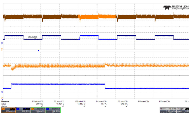
Figure 57 – Transient Response.
