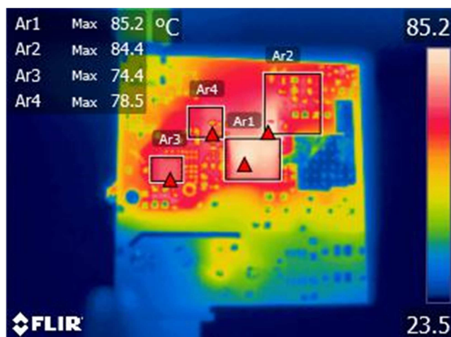
Figure 37 – Bottom Thermal Image.
