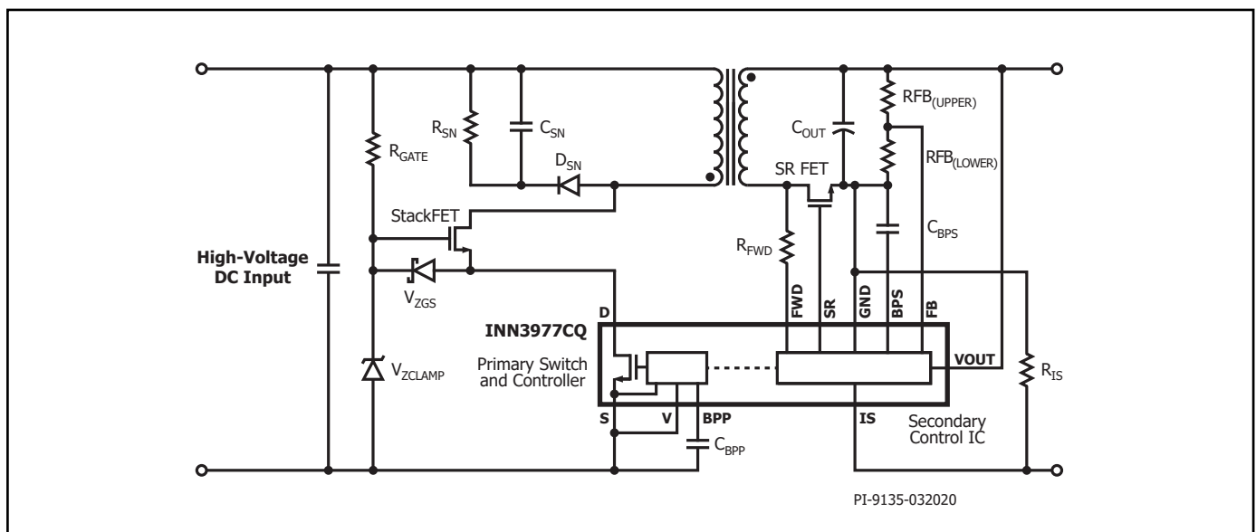
Figure 10. StackFET Circuit Configuration.
