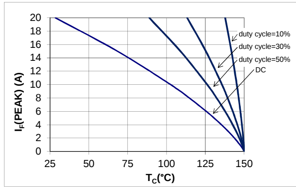
Figure 10. IF (Peak) vs TC, f = 70 \text{ kHz}
