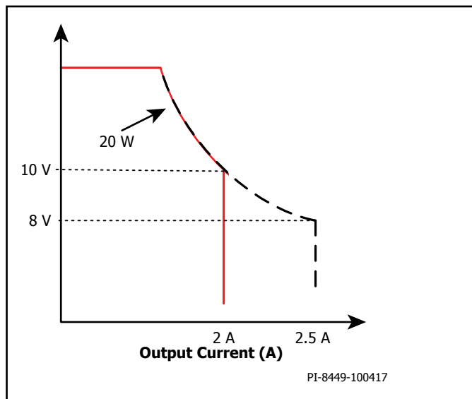
Figure 10. Constant Output Power Profile with Reduced CC Regulation Threshold.
