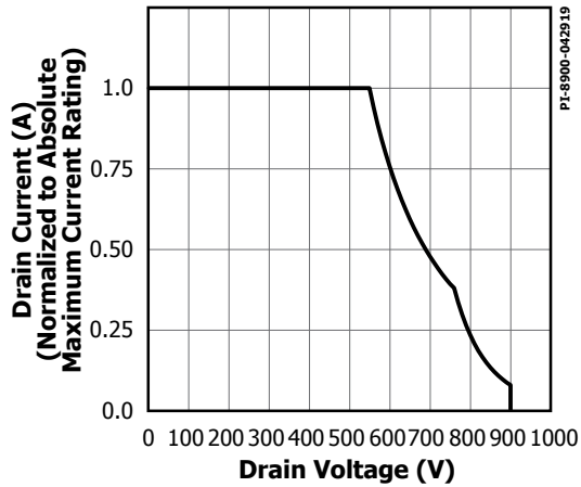
Figure 42. Maximum Allowable Drain Current vs. Drain Voltage (INN389x).
