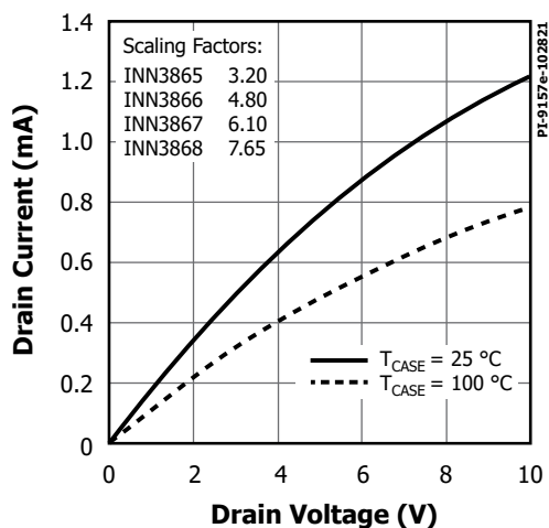
Figure 28. Output Characteristics.
