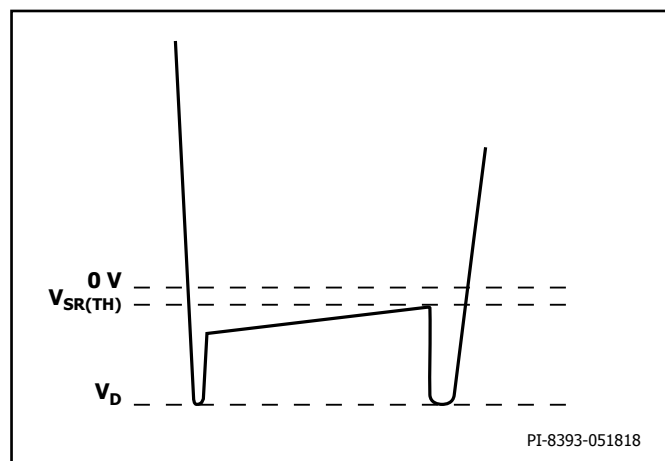
Figure 19. Acceptable FORWARD Pin Waveform After Handshake With SR FET Conduction During Flyback Cycle.
