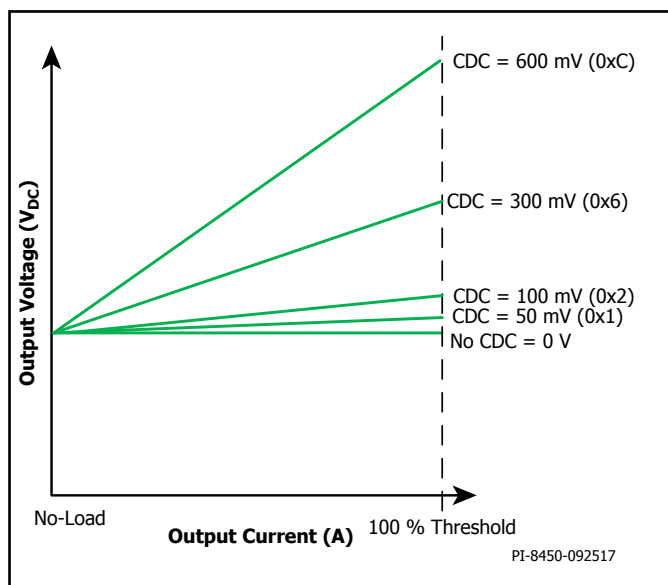
Figure 11. CDC as Function of Load Current.
