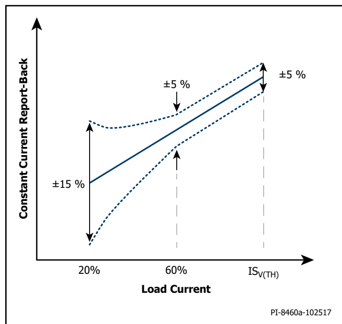
Figure 14. Constant-Current Report Back Tolerance.
