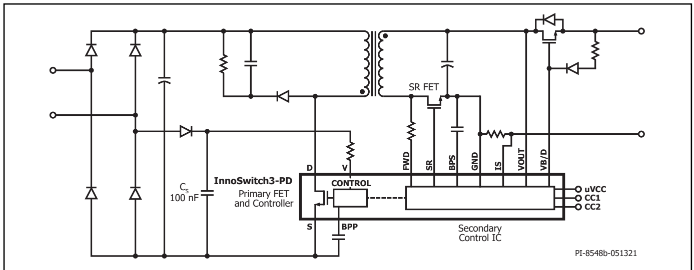
Figure 17. Figure 3. Fast AC Reset Configuration.
