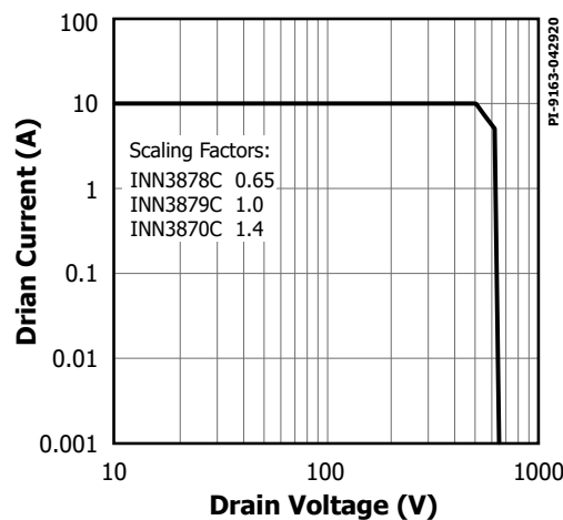
Figure 37. Maximum Allowable Drain Current vs. Drain Voltage (PwGaN Devices INN3878-INN3870).
