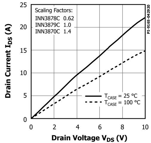
Figure 34. Output Characteristics.
