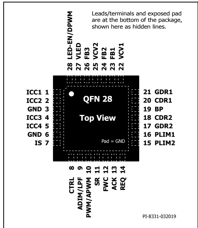
Figure 5. InnoMux QFN-28 Controller Pin Configuration.
