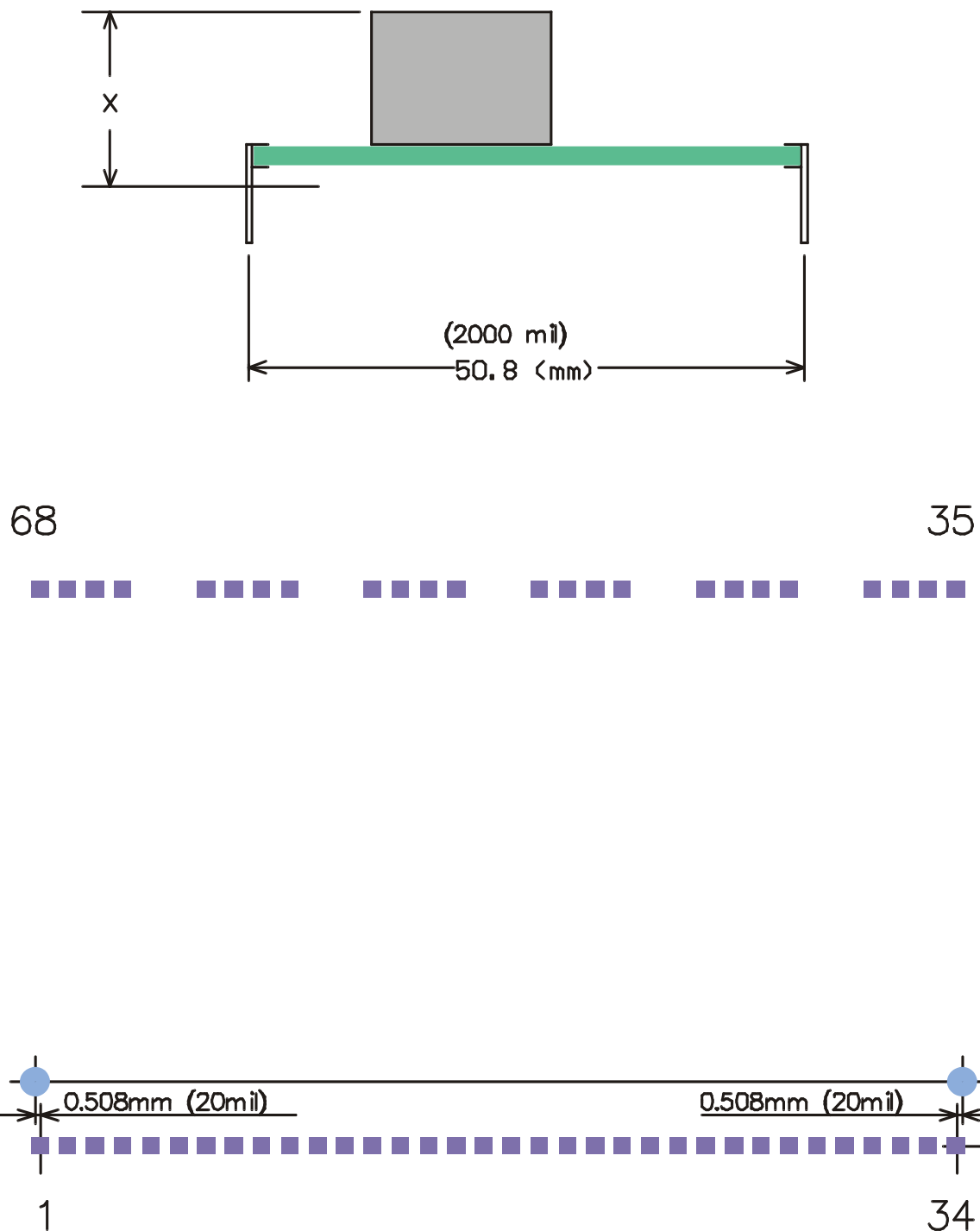
Fig. 3 Side view (top) / Mechanical fixing (bottom) 6SD106EI-17
