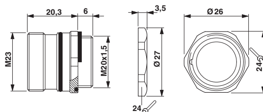
Dimensional drawing
