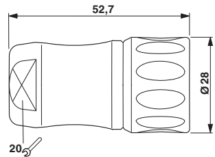
Dimensional drawing
