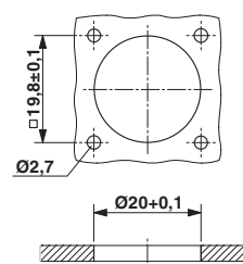
Dimensional drawing
