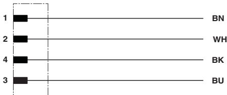
Contact assignment of M12 plugs / sockets bridged
