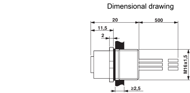
M12 flush-type connector
