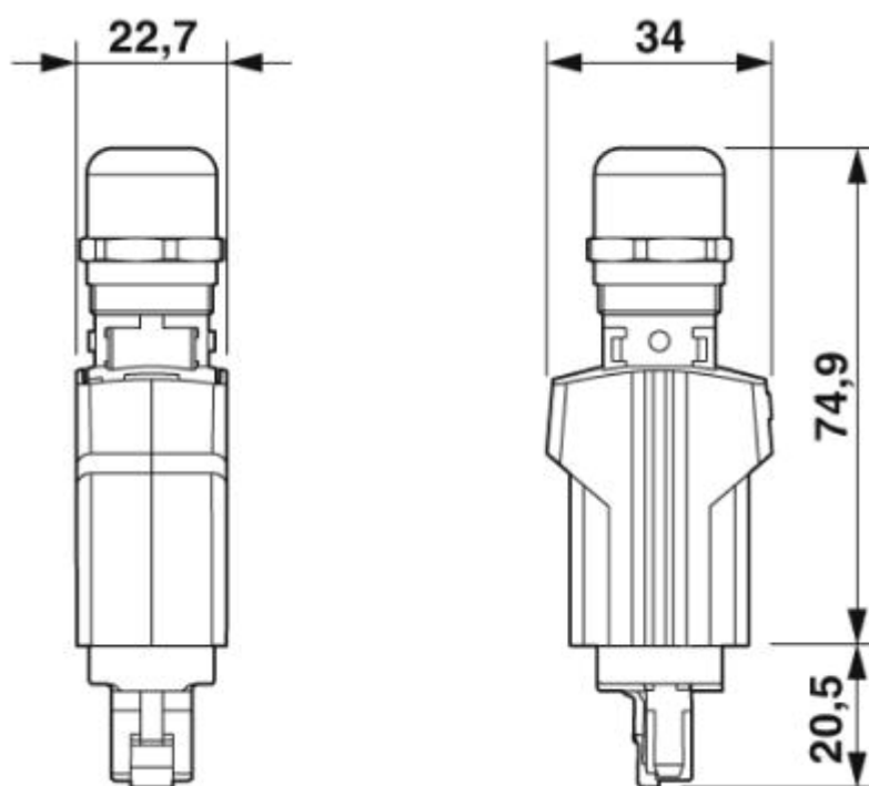
Dimensional drawing
