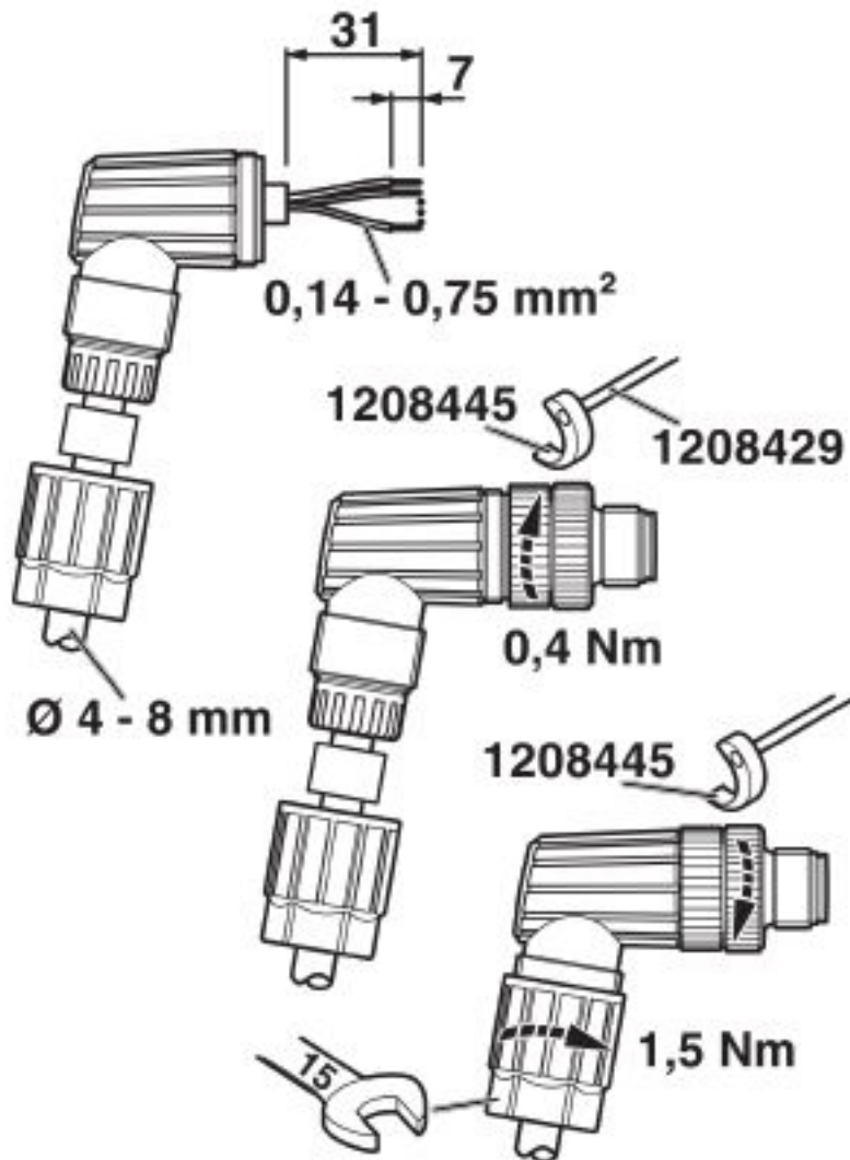
Functional drawing
