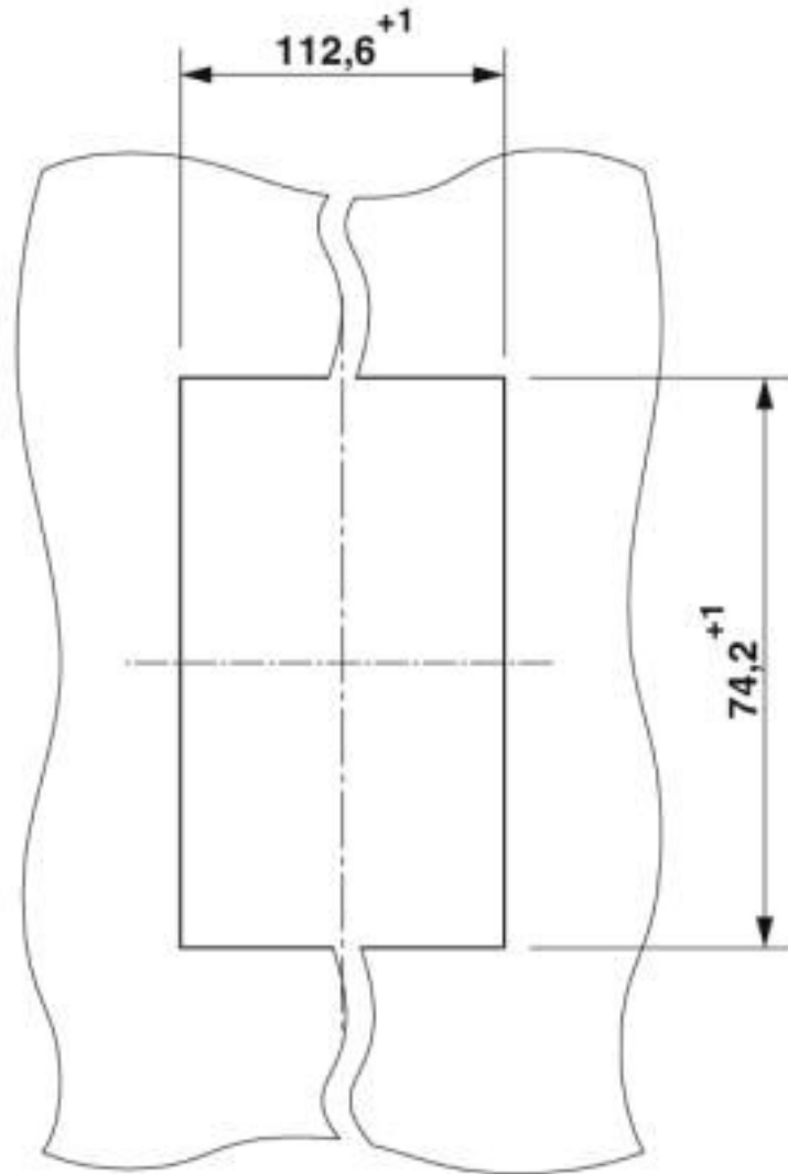
Dimensional drawing
