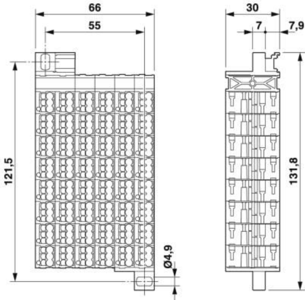
Dimensional drawing
