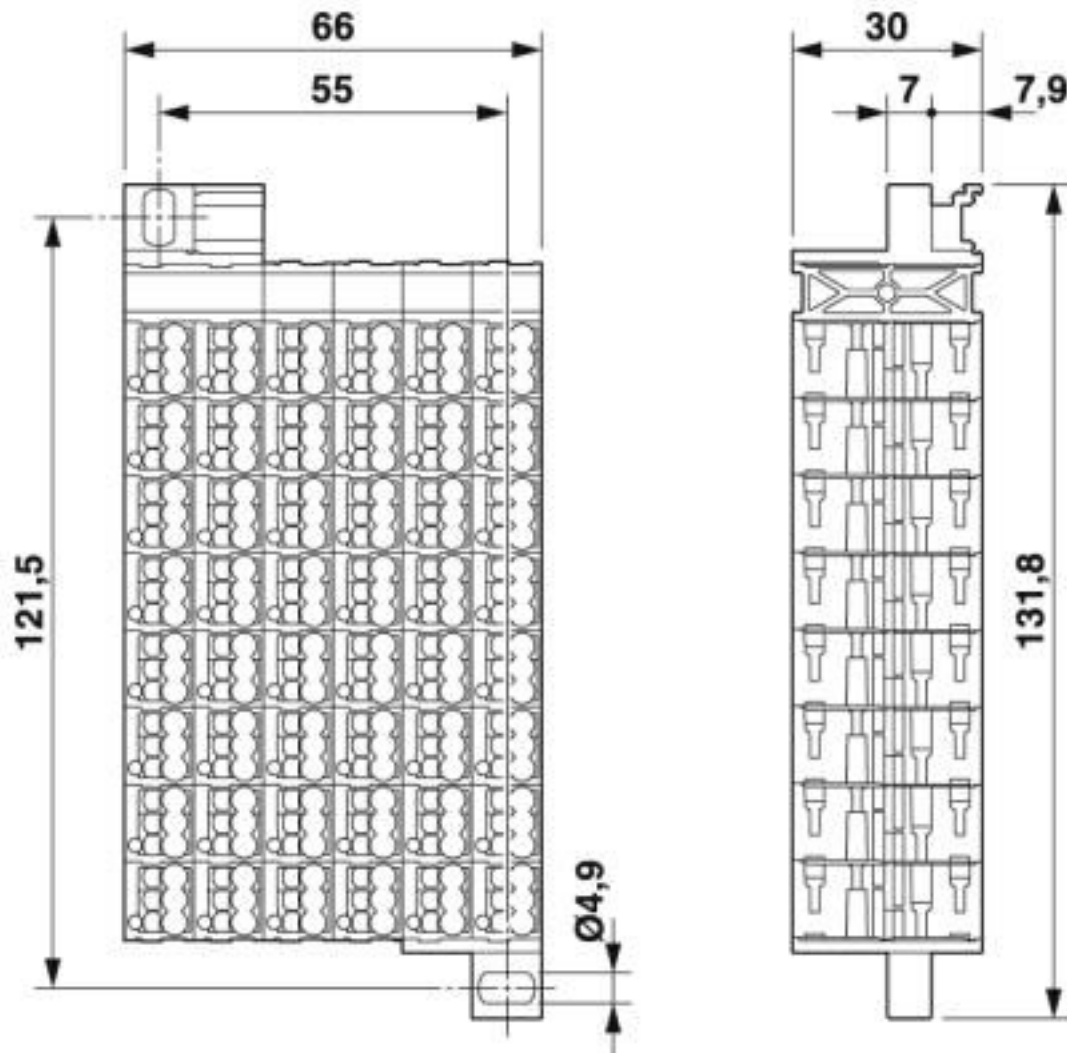
Dimensional drawing
