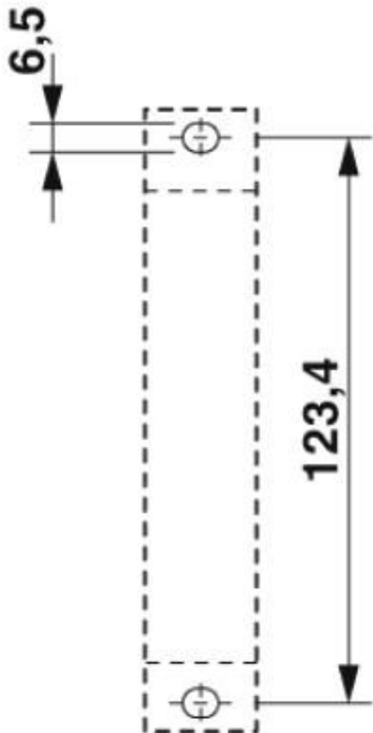
Dimensional drawing
