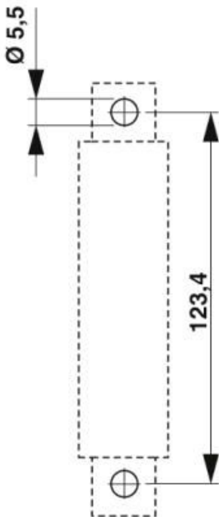
Dimensional drawing
