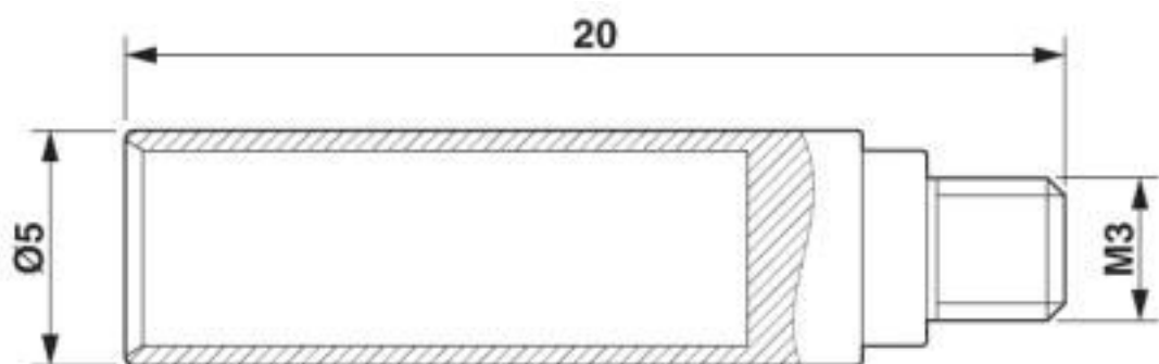
Dimensional drawing
