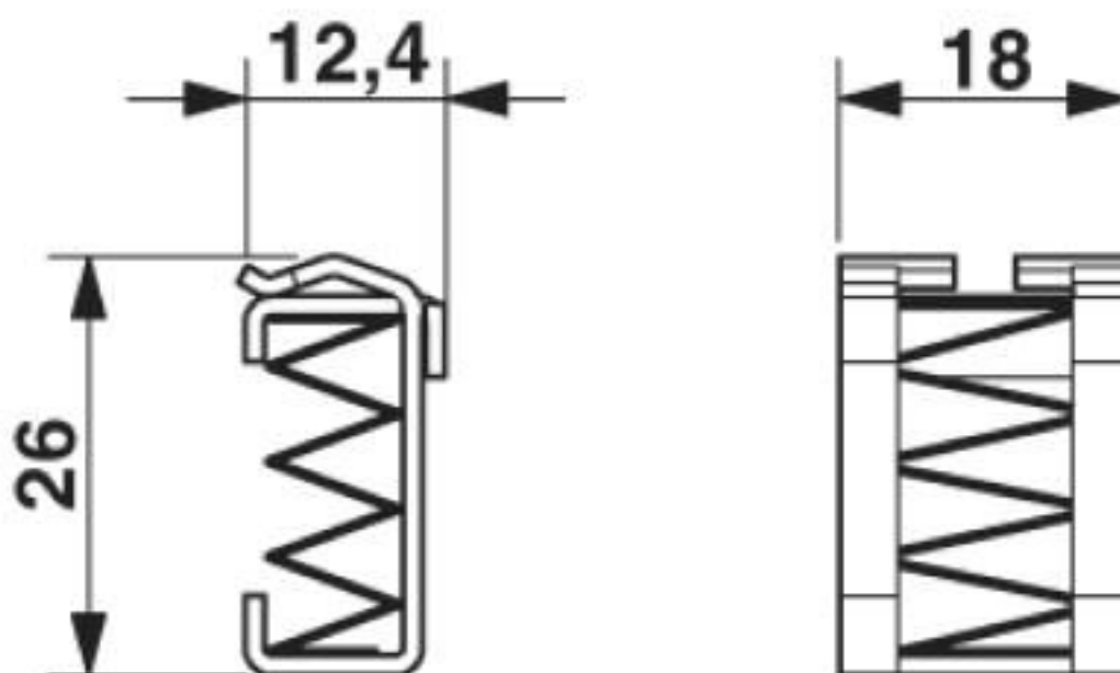
Dimensional drawing
