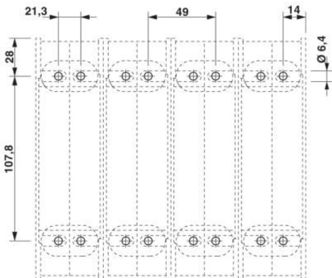
Dimensional drawing
