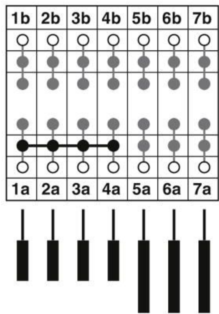
Circuit diagram
