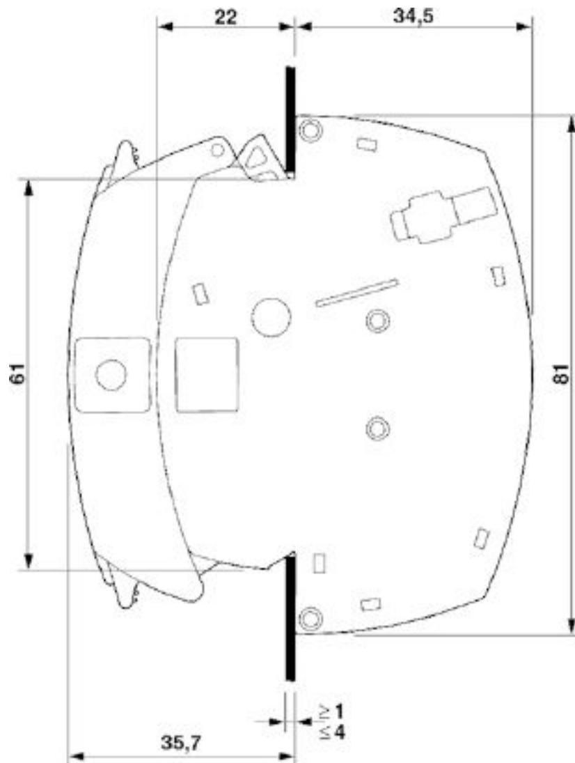
Dimensional drawing
